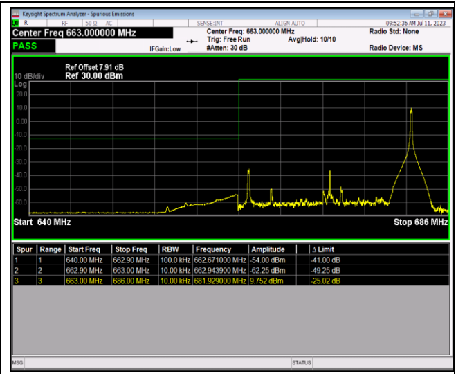
Band71-20MHz-64QAM-133372-1RB#0
