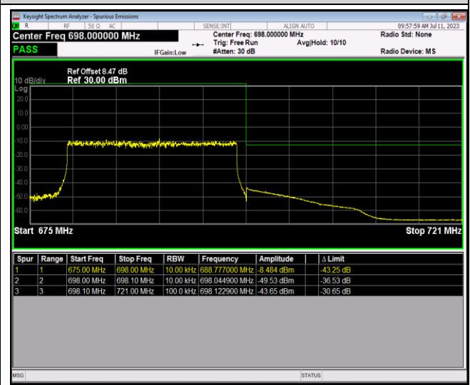
Band71-20MHz-64QAM-133372-100RB#0
