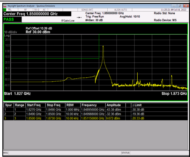
Band25-20MHz-QPSK-26140-100RB#0
