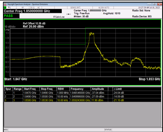
Band25-1.4MHz-16QAM-26047-6RB#0
