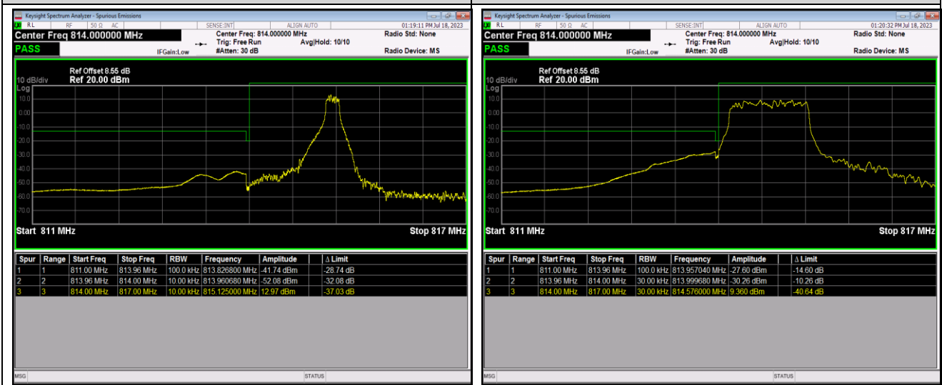
Band26-1.4MHz-64QAM-26783-1RB#0
