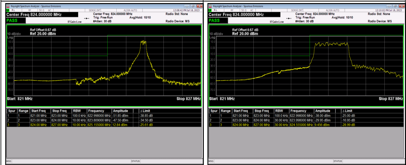
Band26-1.4MHz-64QAM-27033-1RB#0
