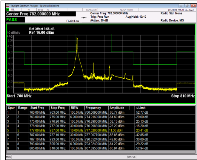
Band13-10MHz-64QAM-23230-50RB#0
