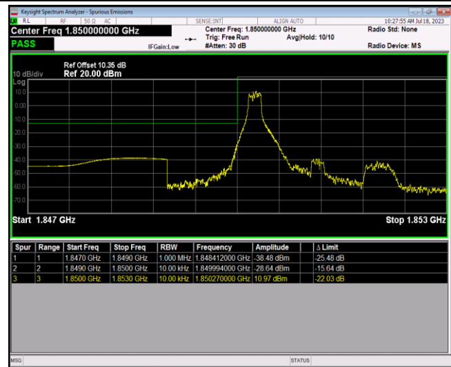
Band25-1.4MHz-64QAM-26047-6RB#0
