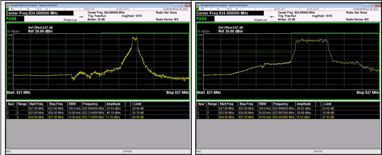
Band26-1.4MHz-QPSK-27033-1RB#0
