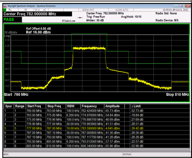
Band13-10MHz-64QAM-23230-1RB#49
