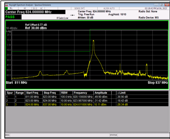
Band5-10MHz-64QAM-20450-50RB#0
