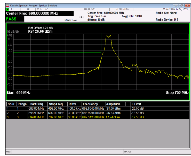
Band12-1.4MHz-16QAM-23017-6RB#0
