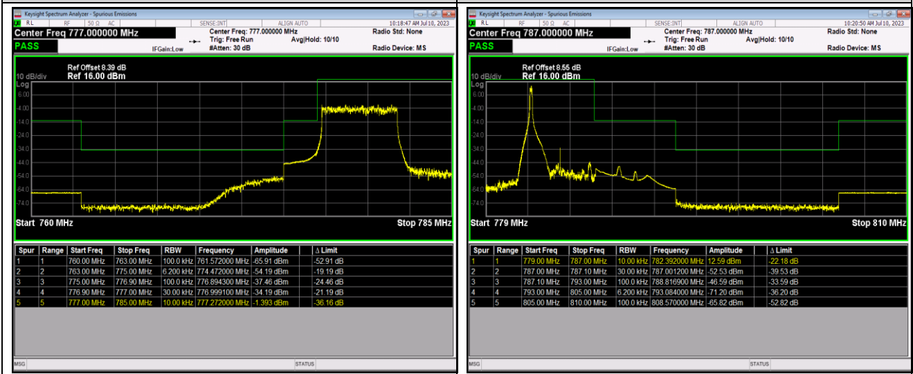
Band13-5MHz-16QAM-23255-1RB#24
