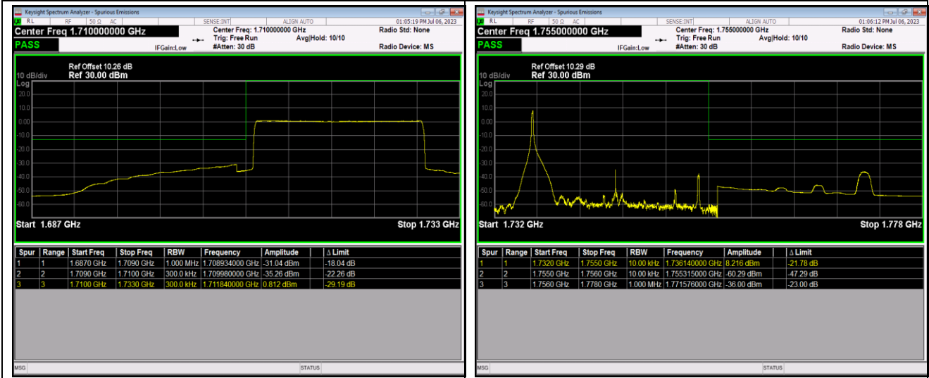
Band4-20MHz-64QAM-20300-1RB#99
