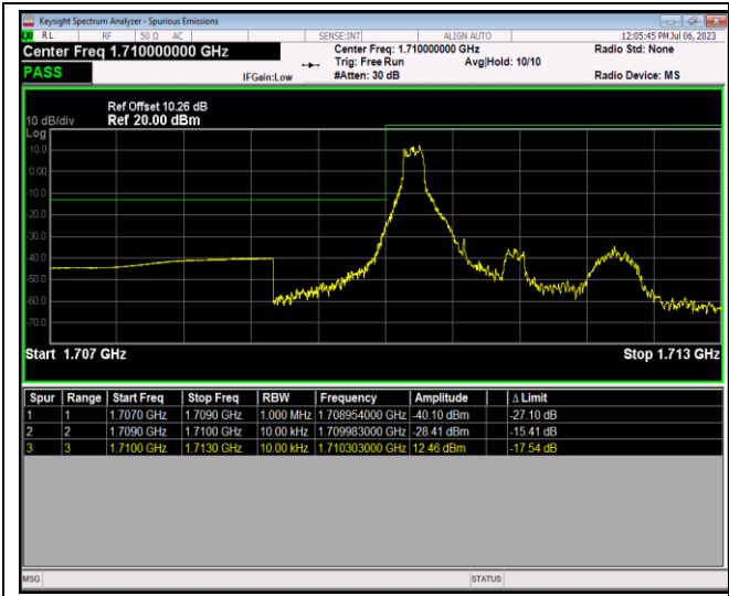
Band4-1.4MHz-64QAM-19957-6RB#0
