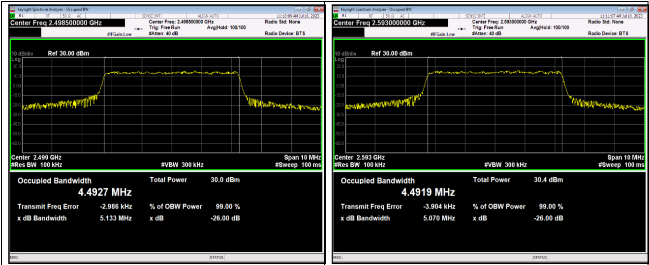
Band41-5MHz-16QAM-41565-25RB#0
