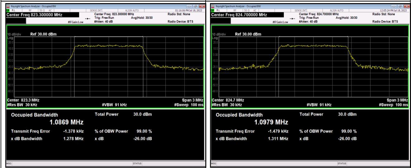
Band26-1.4MHz-64QAM-26915-6RB#0
