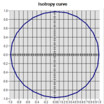
Isotropy: +/- 1.66% (+/- 0.07dB)
