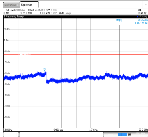
Band4-3MHz-QPSK-20175-1RB#0-3000~20000-PASS
