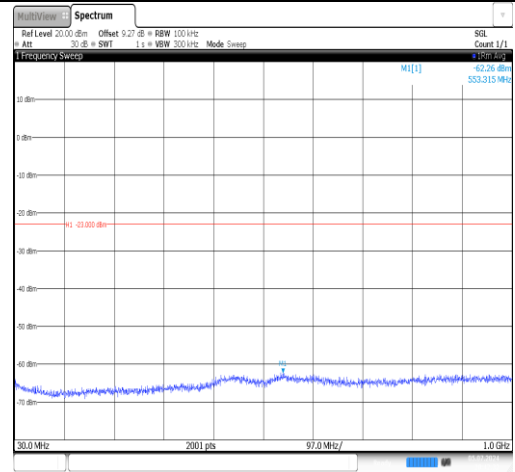
Band4-1.4MHz-QPSK-20175-1RB#0-30~1000-PASS
