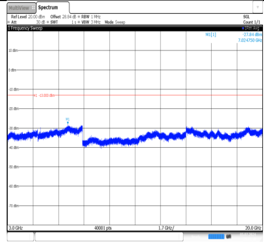
Band4-1.4MHz-QPSK-20175-1RB#0-3000~20000-PASS
