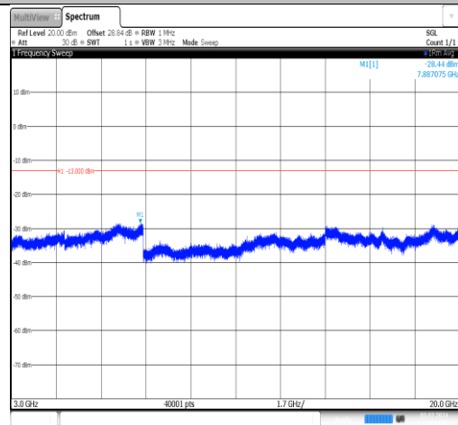
Band2-10MHz-16QAM-19150-1RB#0-3000~20000-PASS
