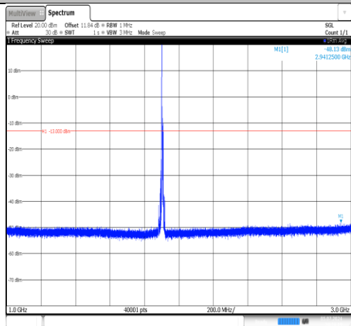
Band2-10MHz-16QAM-19150-1RB#0-1000~3000-PASS
