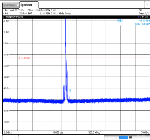
Band2-15MHz-16QAM-18675-1RB#0-1000~3000-PASS
