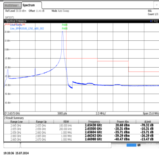
Band41(2535-2655)-15MHz-QPSK-40115-75RB#0-PASS
