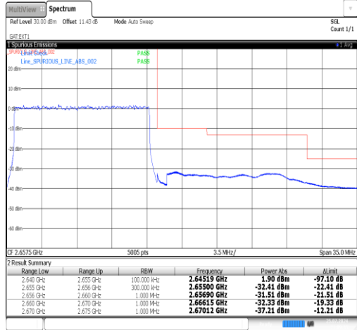
Band41(2535-2655)-15MHz-QPSK-41165-75RB#0-PASS
