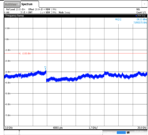
Band2-3MHz-16QAM-18615-1RB#0-3000~20000-PASS
