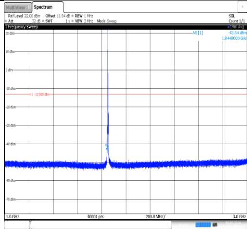
Band2-3MHz-16QAM-18615-1RB#0-1000~3000-PASS
