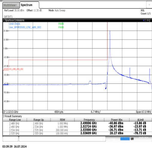
Band41(2535-2655)-20MHz-16QAM-40140-1RB#99-PASS
