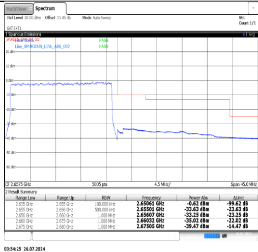
Band41(2535-2655)-20MHz-16QAM-41140-100RB#0-PASS
