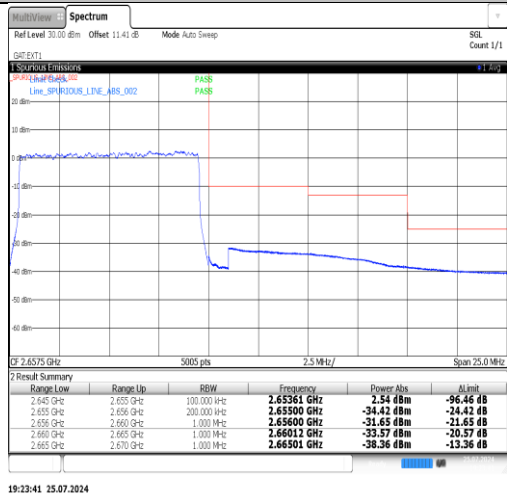
Band41(2535-2655)-15MHz-QPSK-40115-1RB#0-PASS
