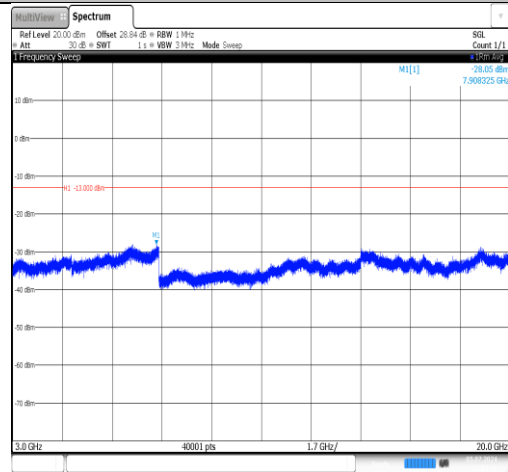
Band2-1.4MHz-16QAM-19193-1RB#0-3000~20000-PASS
