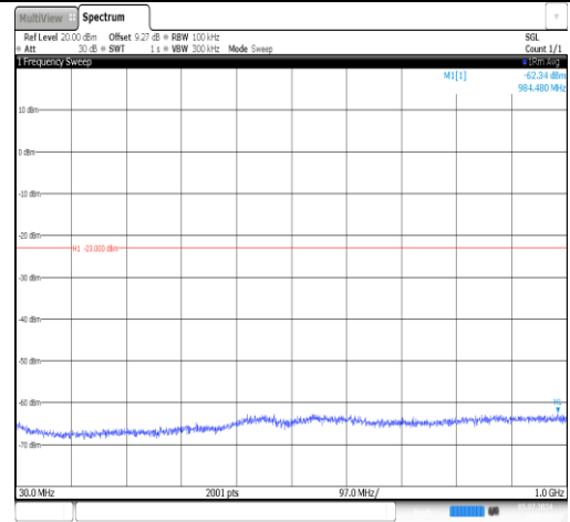
Band2-3MHz-16QAM-18615-1RB#0-30~1000-PASS
