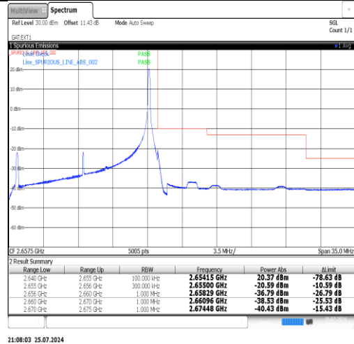
Band41(2535-2655)-20MHz-QPSK-40140-100RB#0-PASS
