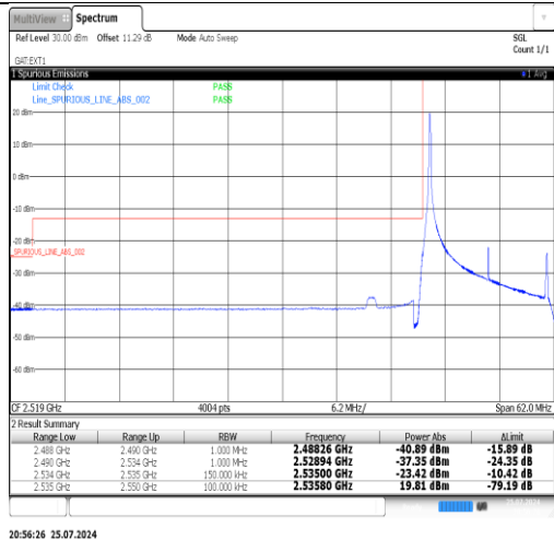
Band41(2535-2655)-15MHz-16QAM-40115-1RB#74-PASS
