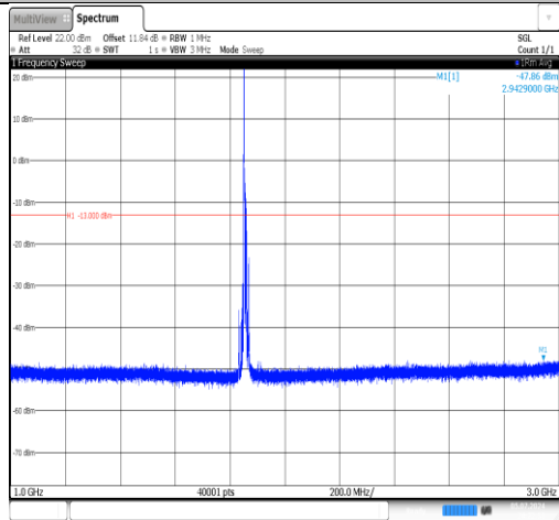
Band2-10MHz-16QAM-18650-1RB#0-1000~3000-PASS
