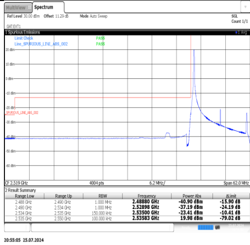
Band41(2535-2655)-15MHz-QPSK-40115-1RB#74-PASS
