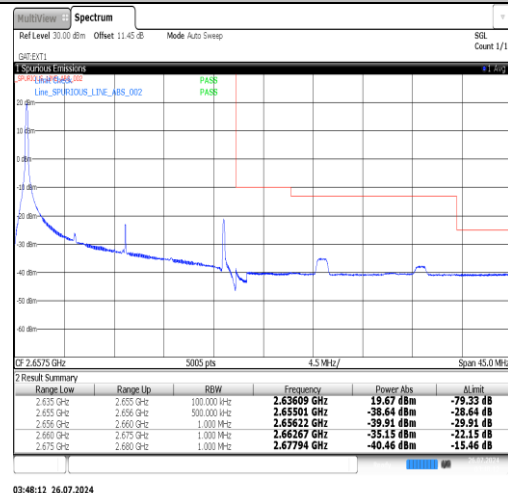
Band41(2535-2655)-20MHz-16QAM-41140-1RB#0-PASS
