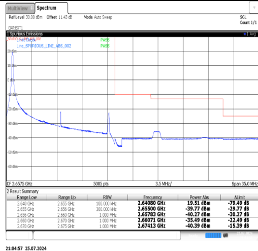
Band41(2535-2655)-15MHz-16QAM-41165-1RB#74-PASS
