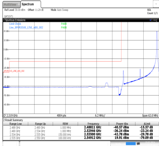
Band41(2535-2655)-15MHz-QPSK-40115-1RB#74-PASS
