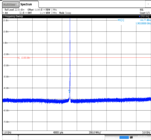
Band2-3MHz-16QAM-19185-1RB#0-1000~3000-PASS
