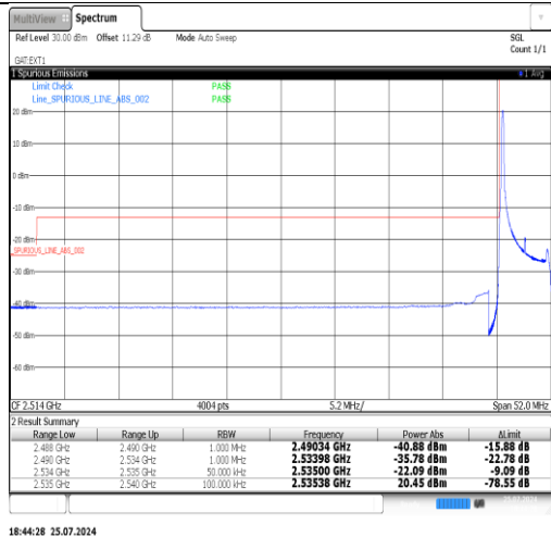
Band41(2535-2655)-5MHz-16QAM-40065-1RB#24-PASS
