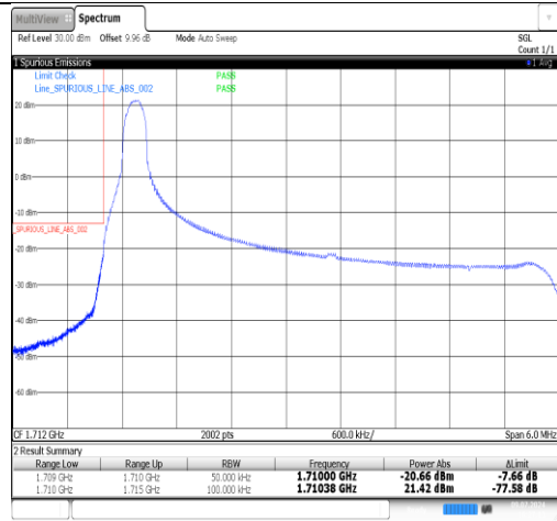
Band66-5MHz-QPSK-131997-1RB#24-PASS
