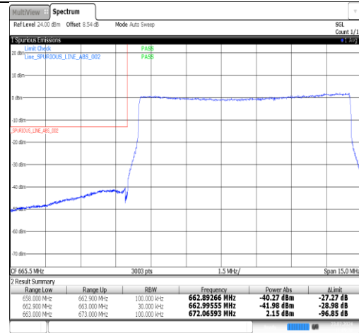
Band71-10MHz-16QAM-133422-1RB#0-PASS
