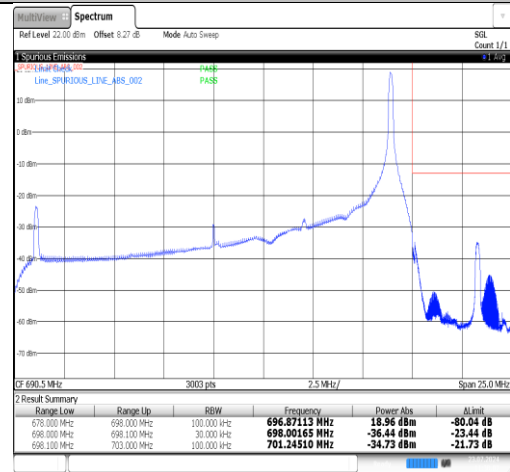
Band71-20MHz-16QAM-133372-1RB#99-PASS
