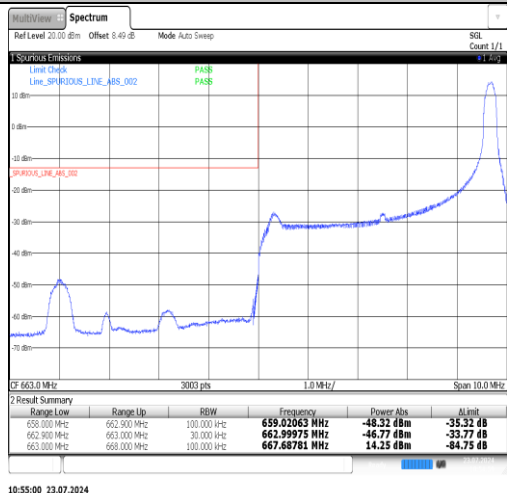
Band71-5MHz-QPSK-133447-25RB#0-PASS
