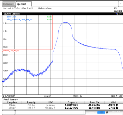
Band66-1.4MHz-16QAM-131979-1RB#5-PASS
