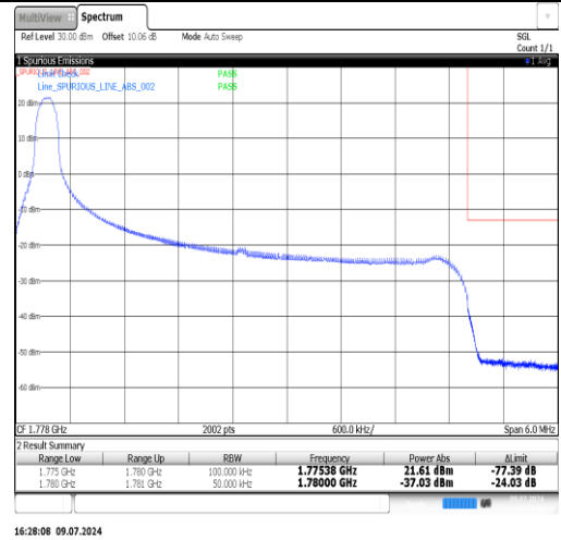
Band66-5MHz-QPSK-132647-1RB#24-PASS
