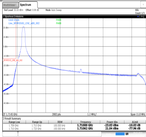
Band66-10MHz-QPSK-132022-1RB#49-PASS
