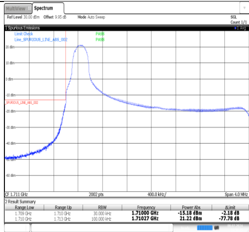
Band66-3MHz-16QAM-131987-1RB#14-PASS
