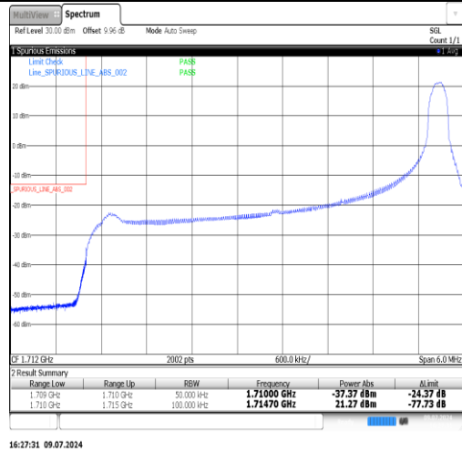
Band66-5MHz-QPSK-132647-25RB#0-PASS
