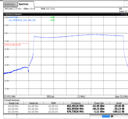
Band71-20MHz-16QAM-133372-1RB#0-PASS
