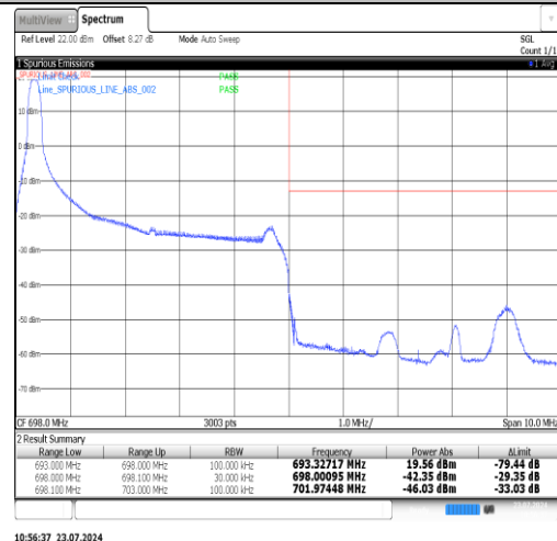
Band71-5MHz-QPSK-133447-1RB#24-PASS
