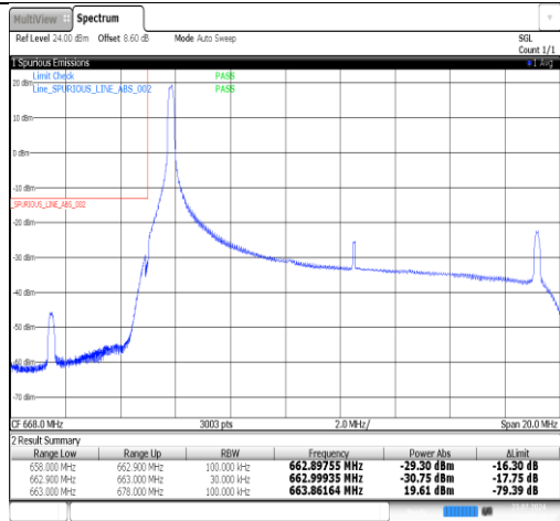
Band71-15MHz-16QAM-133197-1RB#74-PASS
