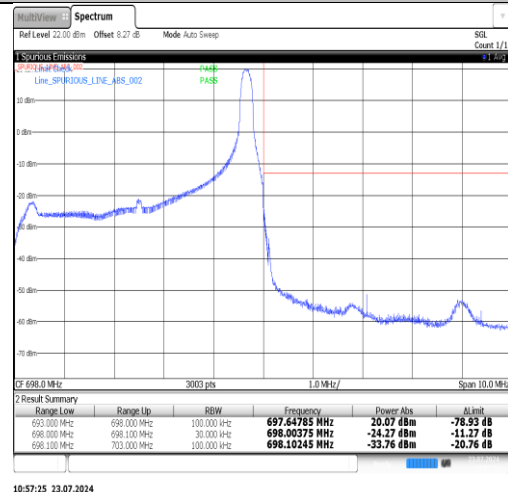
Band71-5MHz-16QAM-133147-25RB#0-PASS
