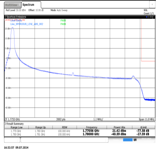
Band66-10MHz-QPSK-132622-1RB#49-PASS
