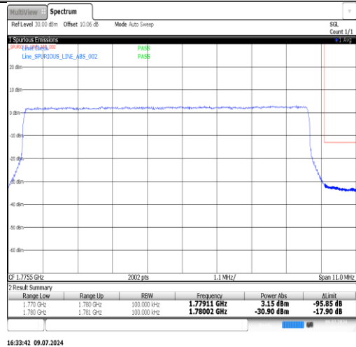
Band66-15MHz-QPSK-132047-1RB#0-PASS
