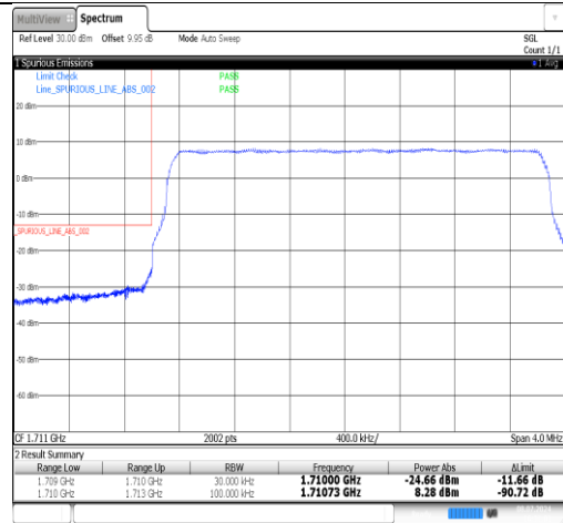
Band66-3MHz-16QAM-132657-1RB#0-PASS
