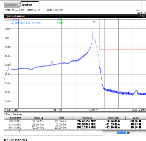
Band71-15MHz-QPSK-133197-75RB#0-PASS
