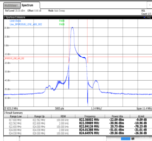
Band26(814-824)-1.4MHz-QPSK-26783-1RB#5-PASS
