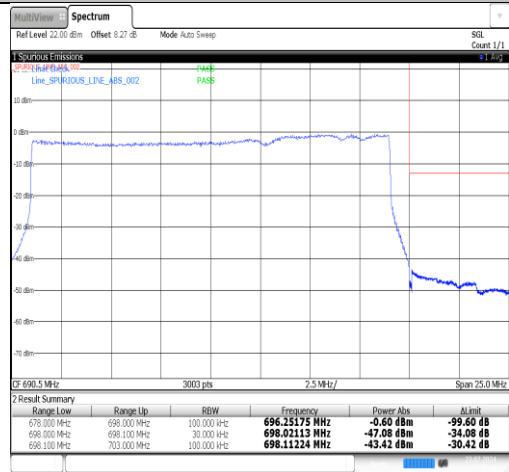
Band71-20MHz-16QAM-133372-100RB#0-PASS
