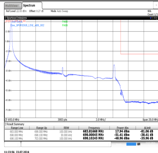
Band71-15MHz-16QAM-133397-1RB#74-PASS
