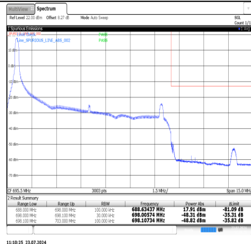
Band71-10MHz-16QAM-133422-1RB#49-PASS
