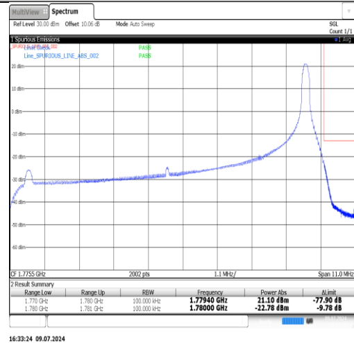
Band66-15MHz-QPSK-132047-75RB#0-PASS
