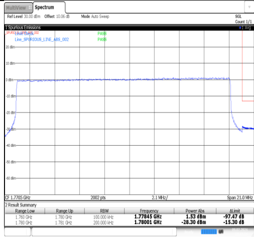
Band66-20MHz-QPSK-132572-100RB#0-PASS
