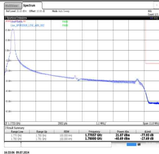
Band66-10MHz-16QAM-132622-1RB#49-PASS
