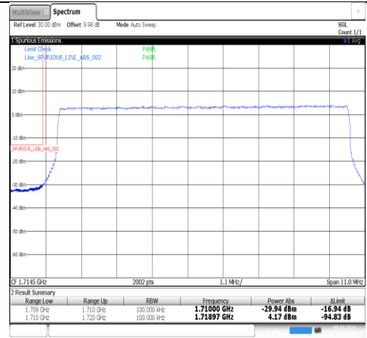
Band66-10MHz-QPSK-132622-1RB#0-PASS
