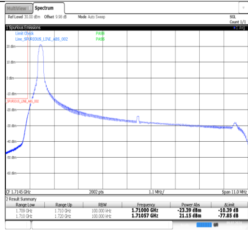
Band66-10MHz-16QAM-132022-1RB#49-PASS
