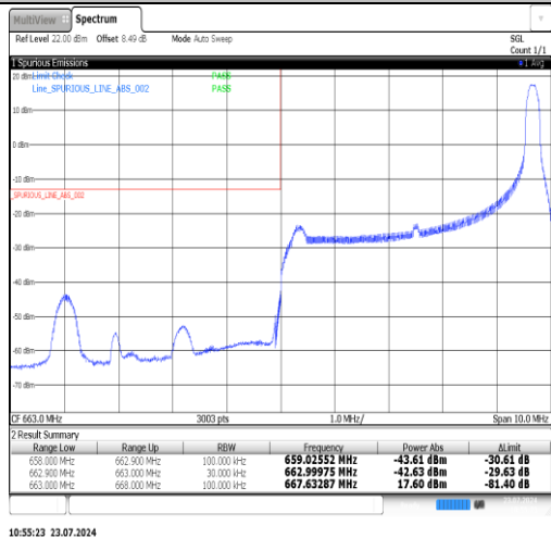
Band71-5MHz-16QAM-133447-25RB#0-PASS
