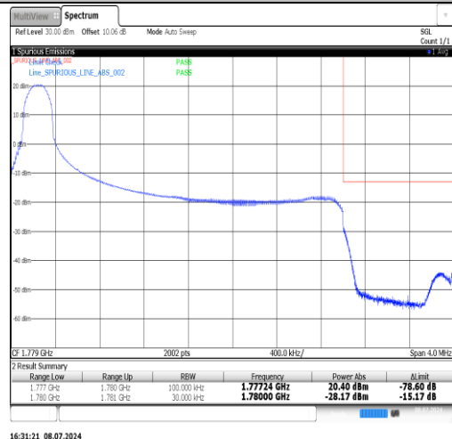
Band66-3MHz-16QAM-132657-1RB#14-PASS
