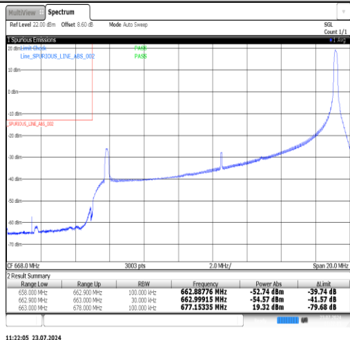
Band71-15MHz-16QAM-133397-75RB#0-PASS
