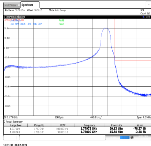
Band66-5MHz-QPSK-131997-25RB#0-PASS
