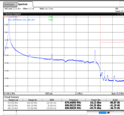
Band71-20MHz-16QAM-133372-1RB#99-PASS
