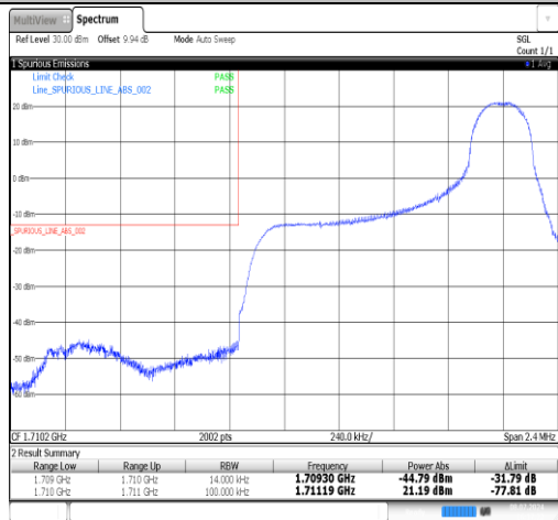
Band66-1.4MHz-16QAM-132665-6RB#0-PASS
