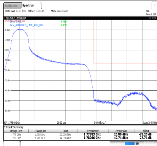
Band66-1.4MHz-16QAM-132665-1RB#5-PASS
