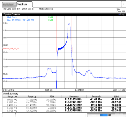
Band26(814-824)-1.4MHz-QPSK-26783-6RB#0-PASS
