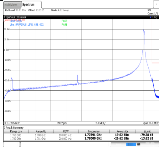
Band66-20MHz-16QAM-132572-1RB#99-PASS
