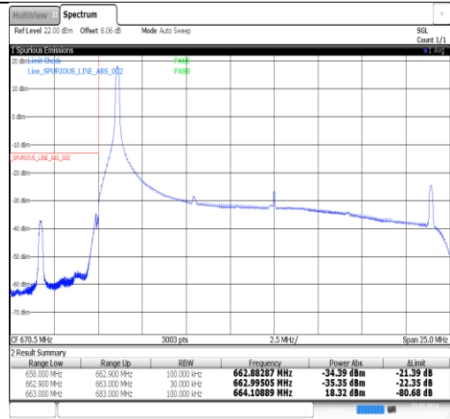
Band71-20MHz-16QAM-133222-1RB#99-PASS
