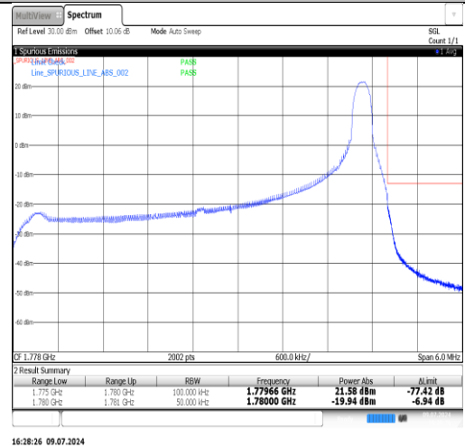
Band66-5MHz-16QAM-131997-25RB#0-PASS
