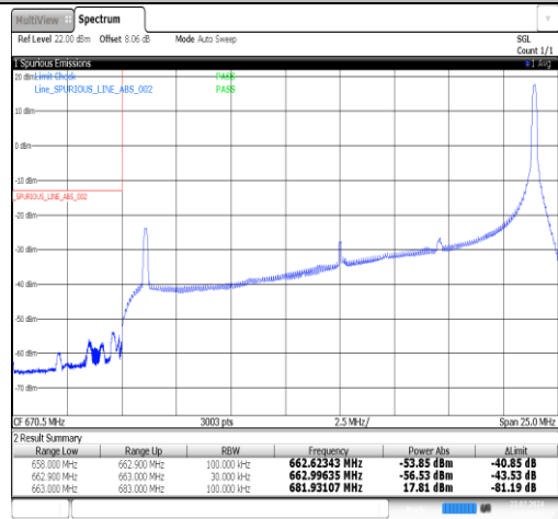
Band71-20MHz-16QAM-133372-100RB#0-PASS
