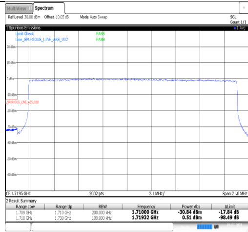
Band66-20MHz-16QAM-132572-1RB#0-PASS
