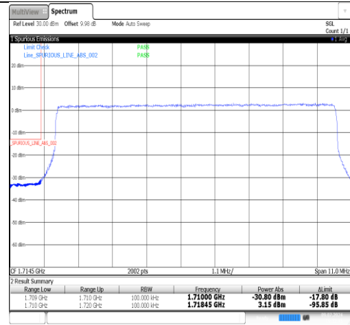
Band66-10MHz-16QAM-132622-1RB#0-PASS
