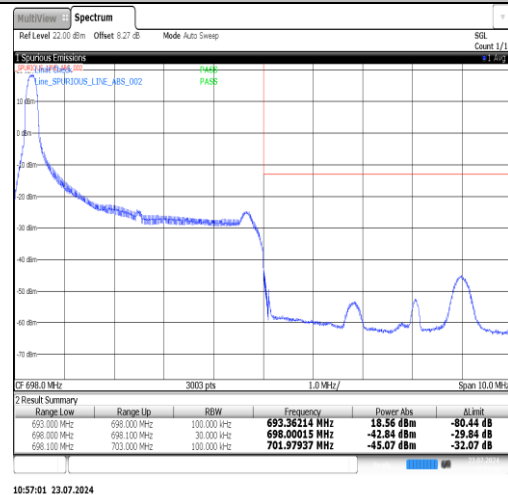
Band71-5MHz-16QAM-133447-1RB#24-PASS
