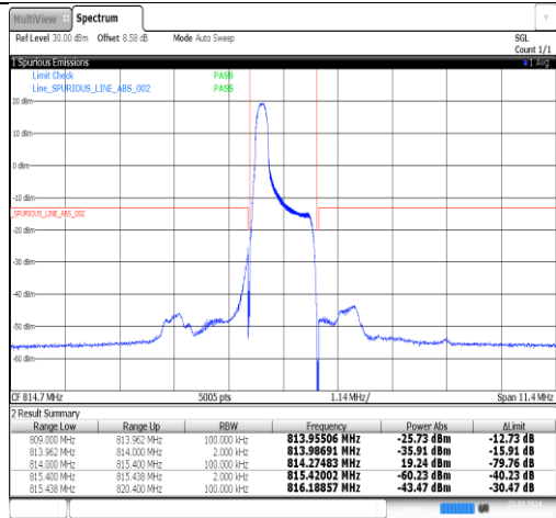
Band26(814-824)-1.4MHz-QPSK-26697-1RB#5-PASS
