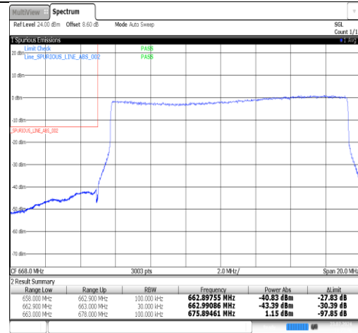
Band71-15MHz-16QAM-133397-1RB#0-PASS
