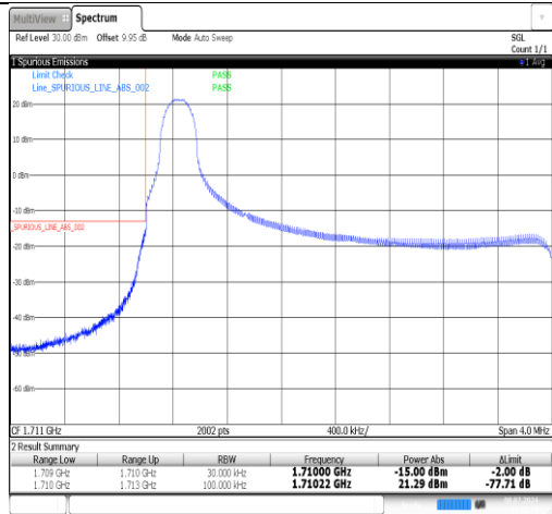
Band66-3MHz-QPSK-131987-1RB#14-PASS
