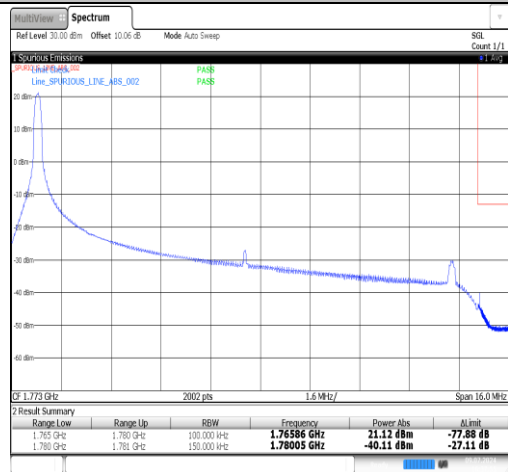
Band66-15MHz-16QAM-132597-1RB#74-PASS
