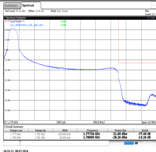
Band66-3MHz-QPSK-132657-1RB#14-PASS
