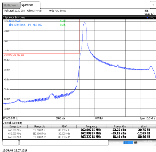
Band71-5MHz-16QAM-133147-1RB#24-PASS
