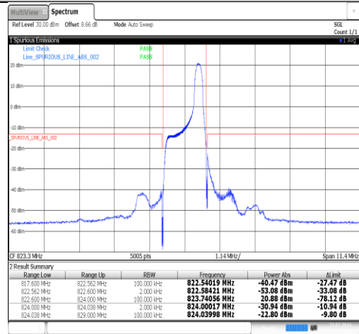
Band26(814-824)-1.4MHz-16QAM-26697-6RB#0-PASS
