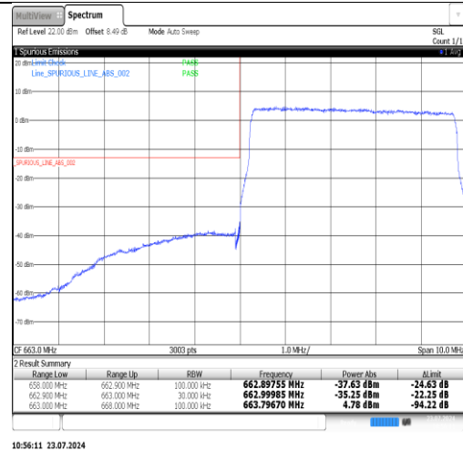
Band71-5MHz-16QAM-133447-1RB#0-PASS
