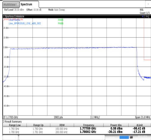
Band66-20MHz-16QAM-132572-100RB#0-PASS
