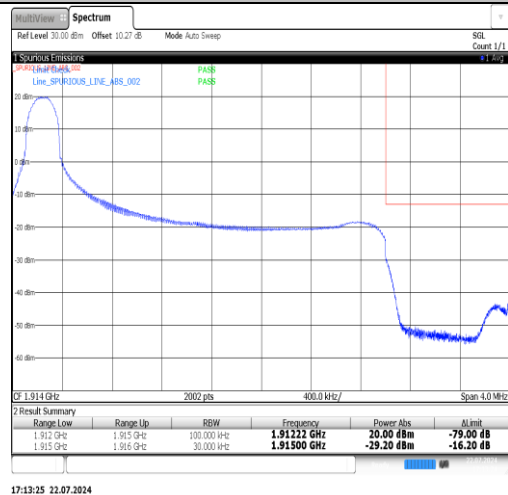
Band25-3MHz-16QAM-26675-1RB#14-PASS
