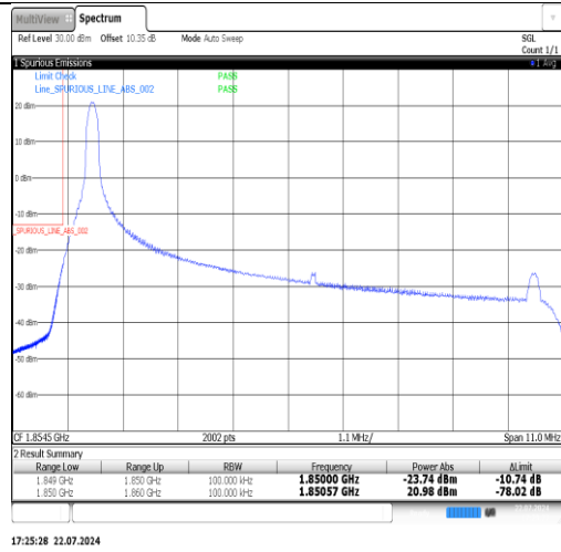
Band25-10MHz-QPSK-26090-1RB#49-PASS
