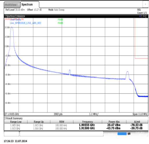
Band25-10MHz-QPSK-26640-1RB#49-PASS
