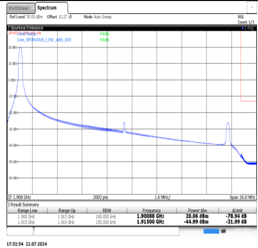
Band25-15MHz-16QAM-26615-1RB#74-PASS
