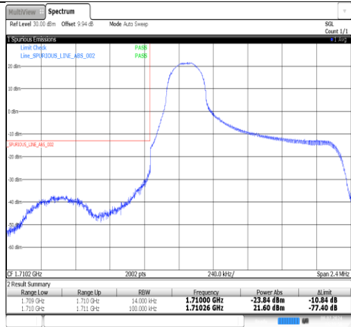
Band66-1.4MHz-QPSK-131979-1RB#5-PASS
