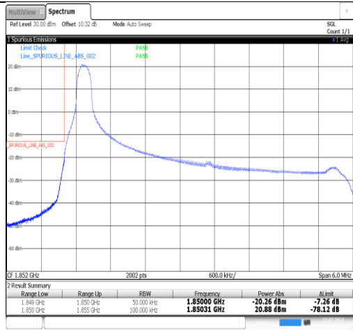
Band25-5MHz-QPSK-26065-1RB#24-PASS
