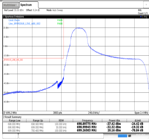
Band12-1.4MHz-16QAM-23017-1RB#5-PASS
