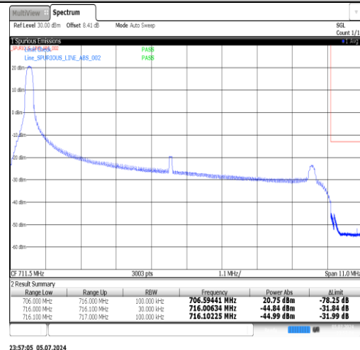
Band12-10MHz-16QAM-23130-1RB#49-PASS
