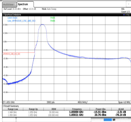
Band25-3MHz-16QAM-26055-1RB#14-PASS
