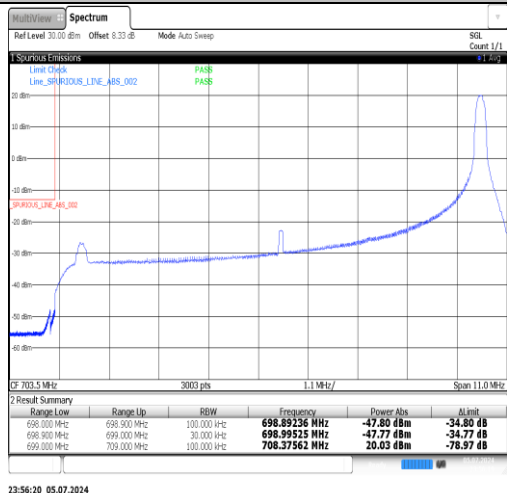
Band12-10MHz-16QAM-23130-50RB#0-PASS
