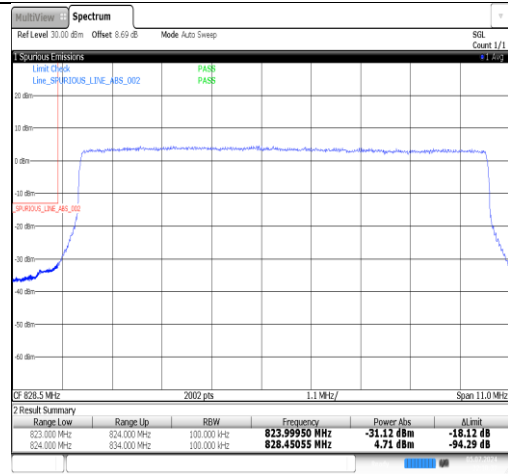
Band5-10MHz-QPSK-20600-1RB#0-PASS
