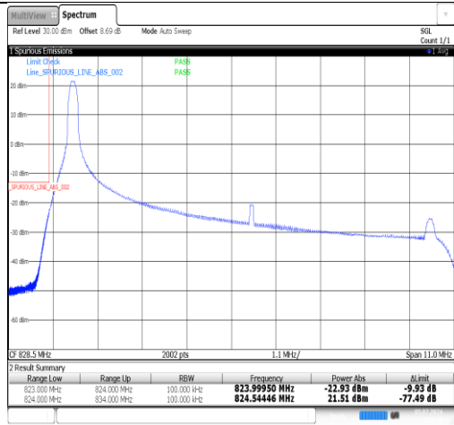
Band5-10MHz-QPSK-20450-1RB#49-PASS
