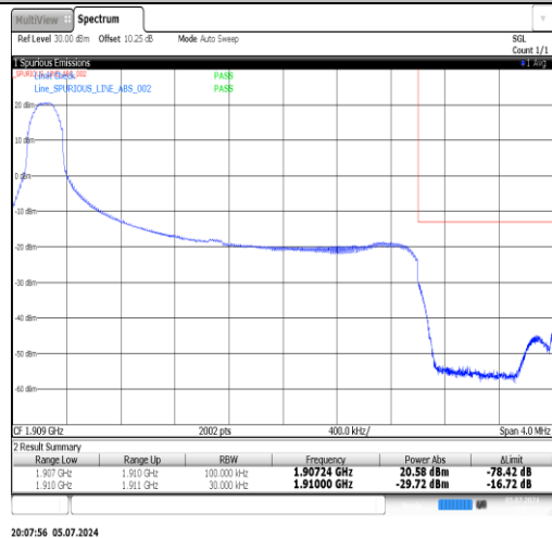
Band2-3MHz-16QAM-19185-1RB#14-PASS
