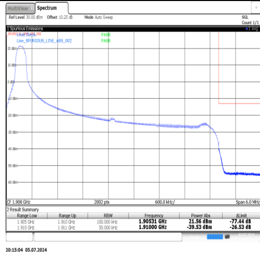
Band2-5MHz-QPSK-19175-1RB#24-PASS
