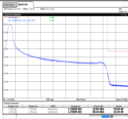
Band4-5MHz-16QAM-20375-1RB#24-PASS
