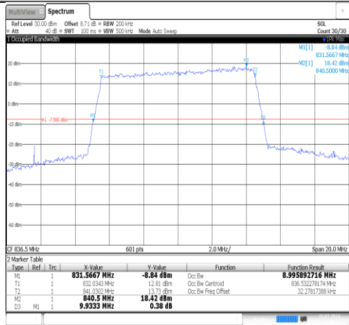
Band26(824-849)-10MHz-QPSK-26915-50RB#0-PASS
