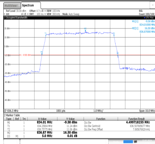
Band26(824-849)-5MHz-16QAM-26915-25RB#0-PASS
