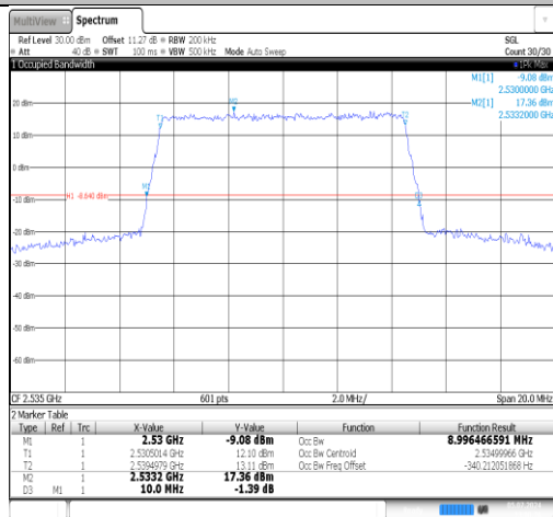
Band7-10MHz-QPSK-21100-50RB#0-PASS
