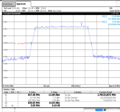
Band26(814-824)-3MHz-QPSK-26740-15RB#0-PASS
