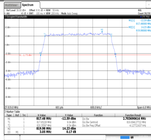
Band26(814-824)-3MHz-16QAM-26740-15RB#0-PASS
