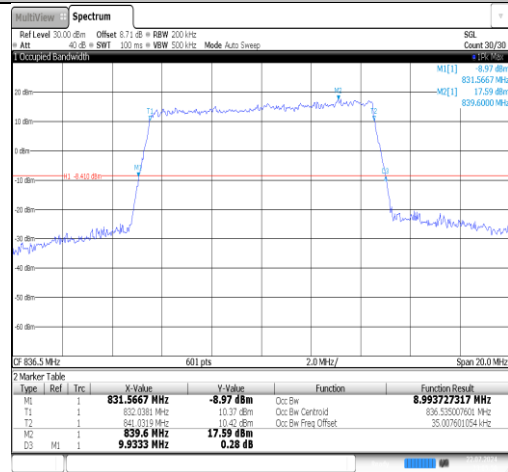
Band26(824-849)-10MHz-16QAM-26915-50RB#0-PASS
