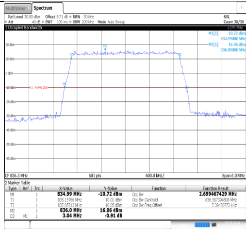
Band26(824-849)-5MHz-QPSK-26915-25RB#0-PASS
