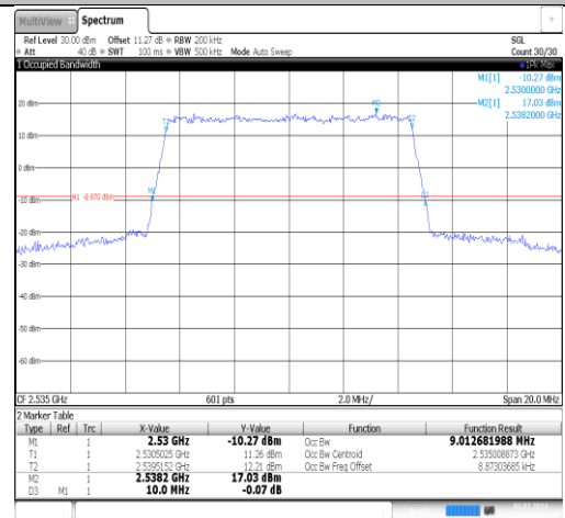
Band7-10MHz-16QAM-21100-50RB#0-PASS
