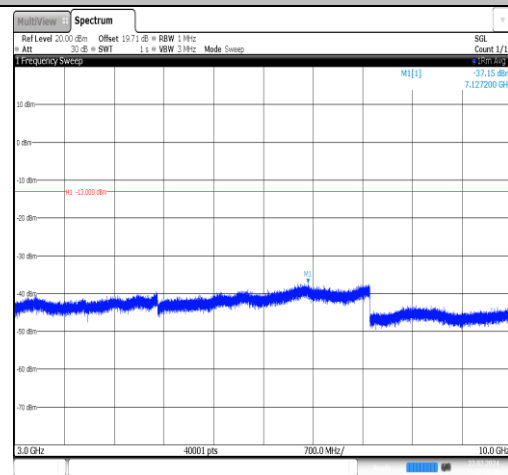
Band26(814-824)-3MHz-16QAM-26775-1RB#0- 3000~10000-PASS
