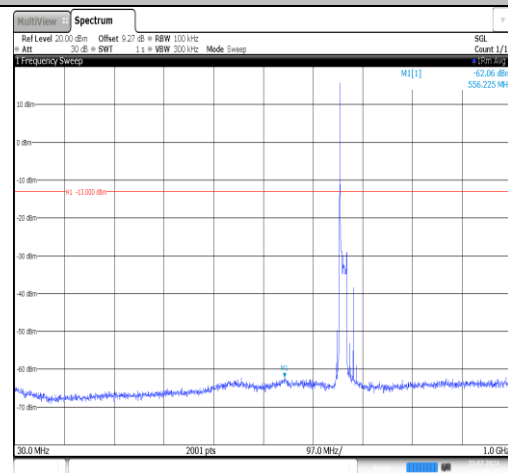
Band71-15MHz-16QAM-133197-1RB#0-30~1000-PASS
