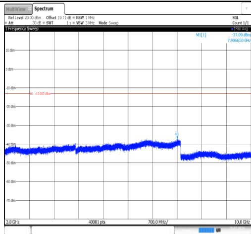
Band71-20MHz-QPSK-133372-1RB#0-3000~10000-PASS
