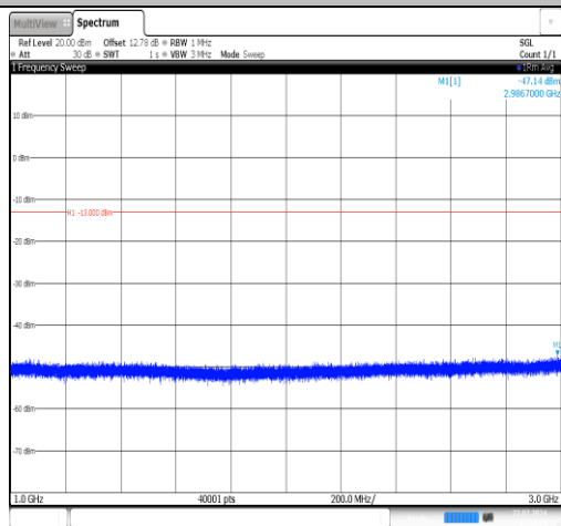
Band26(814-824)-3MHz-16QAM-26775-1RB#0- 1000~3000-PASS
