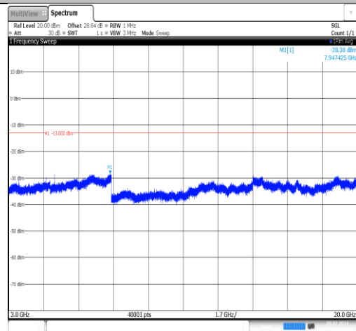
Band66-15MHz-QPSK-132322-1RB#0-3000~20000-PASS
