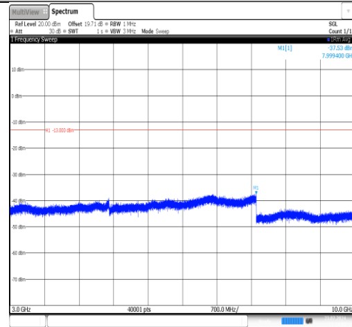
Band71-10MHz-QPSK-133297-1RB#0-3000~10000-PASS
