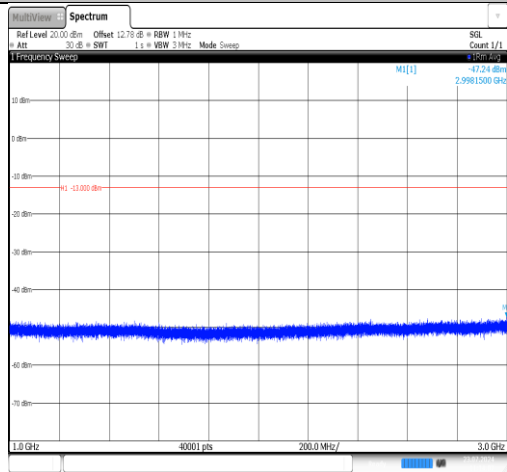
Band71-10MHz-QPSK-133297-1RB#0-1000~3000-PASS
