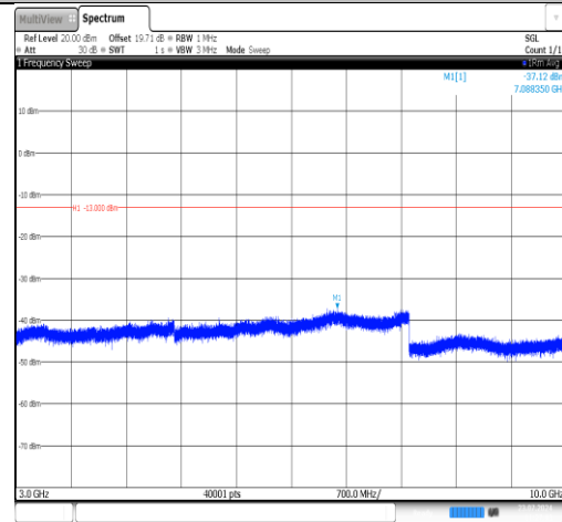
Band71-15MHz-QPSK-133297-1RB#0-3000~10000-PASS
