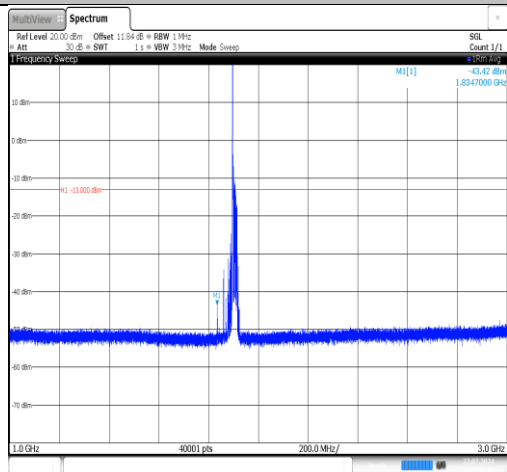
Band25-20MHz-16QAM-26590-1RB#0-1000~3000-PASS
