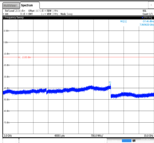
Band71-10MHz-QPSK-133422-1RB#0-3000~10000-PASS
