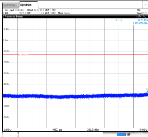
Band71-5MHz-16QAM-133447-1RB#0-1000~3000-PASS
