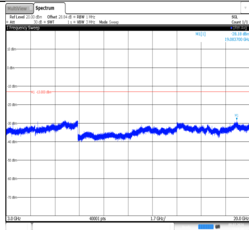
Band66-20MHz-QPSK-132322-1RB#0-3000~20000-PASS
