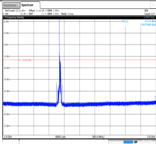
Band66-20MHz-QPSK-132322-1RB#0-1000~3000-PASS
