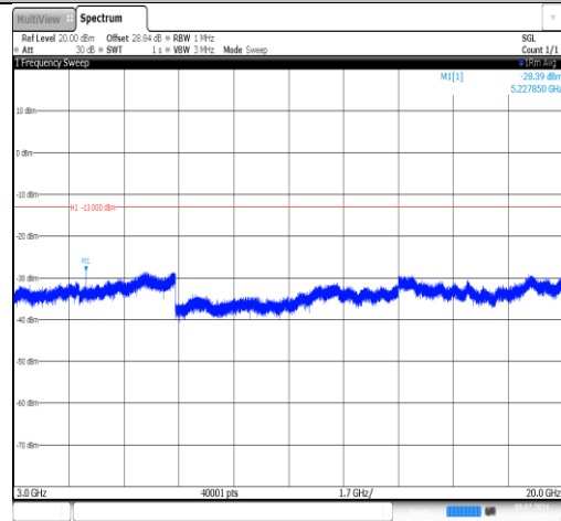
Band66-5MHz-QPSK-132322-1RB#0-3000~20000-PASS
