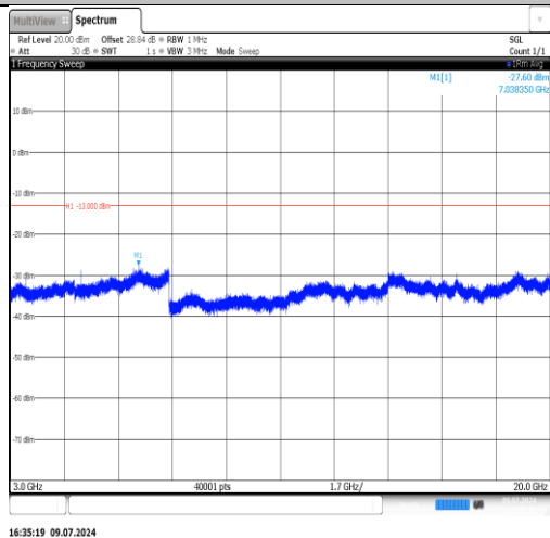
Band66-10MHz-16QAM-132322-1RB#0-3000~20000-PASS
