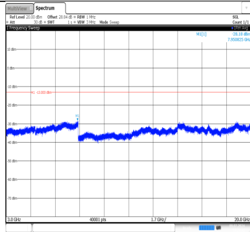
Band66-5MHz-16QAM-131997-1RB#0-3000~20000-PASS
