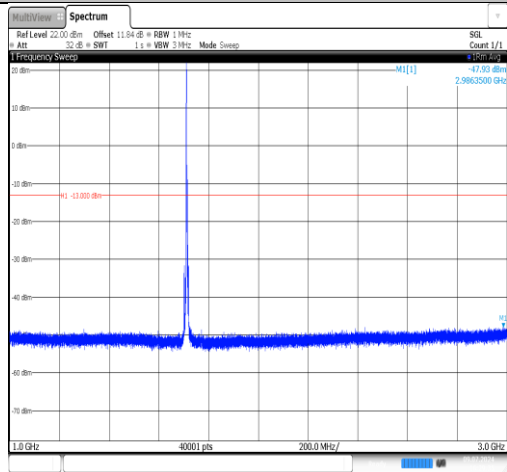
Band66-5MHz-16QAM-131997-1RB#0-1000~3000-PASS
