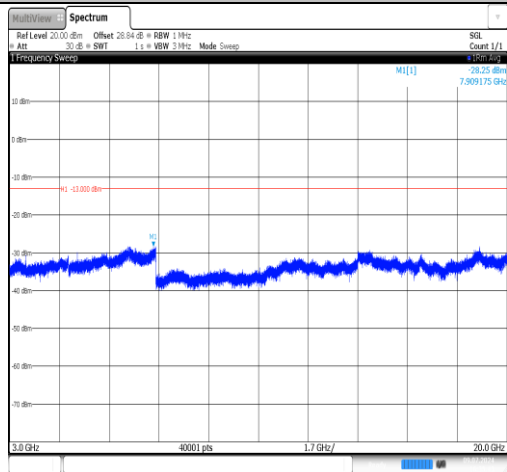
Band66-10MHz-QPSK-132622-1RB#0-3000~20000-PASS
