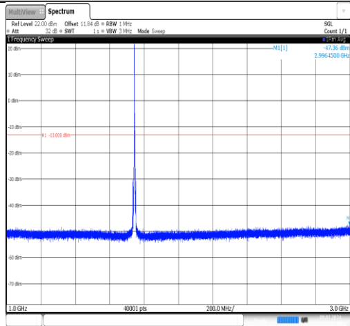
Band66-5MHz-QPSK-132322-1RB#0-1000~3000-PASS
