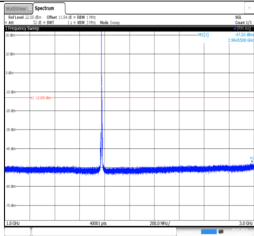
Band66-5MHz-16QAM-132647-1RB#0-1000~3000-PASS
