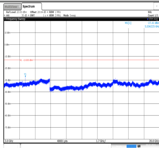
Band66-1.4MHz-16QAM-132665-1RB#0-3000~20000-PASS
