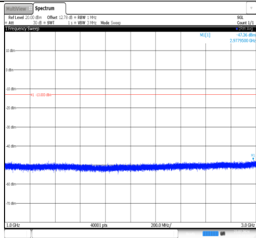
Band71-15MHz-QPSK-133297-1RB#0-1000~3000-PASS
