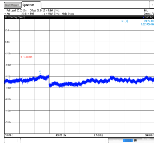
Band66-5MHz-16QAM-132647-1RB#0-3000~20000-PASS
