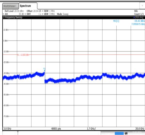
Band25-20MHz-16QAM-26365-1RB#0-3000~20000-PASS
