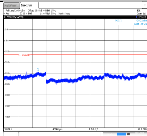
Band25-20MHz-16QAM-26590-1RB#0-3000~20000-PASS
