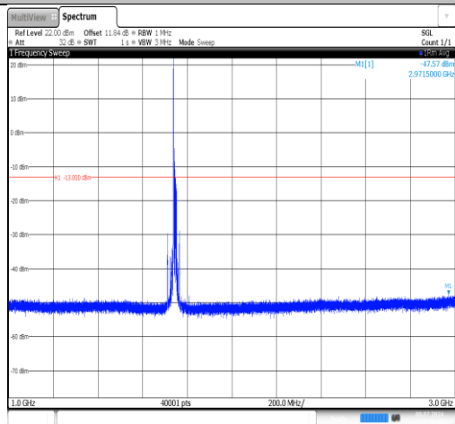
Band66-15MHz-QPSK-132322-1RB#0-1000~3000-PASS
