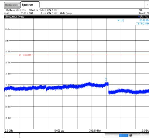
Band71-5MHz-16QAM-133447-1RB#0-3000~10000-PASS
