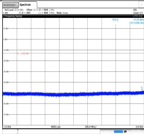
Band12-10MHz-16QAM-23060-1RB#0-1000~3000-PASS
