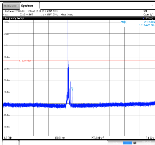
Band25-20MHz-16QAM-26140-1RB#0-1000~3000-PASS
