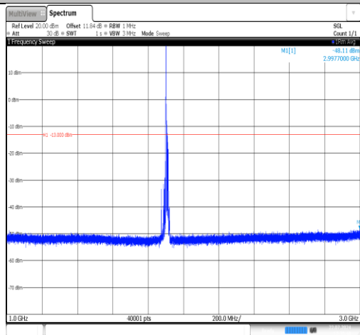
Band25-15MHz-16QAM-26615-1RB#0-1000~3000-PASS
