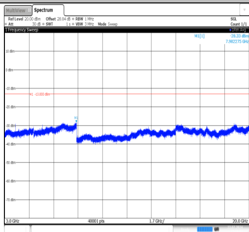
Band25-15MHz-16QAM-26365-1RB#0-3000~20000-PASS
