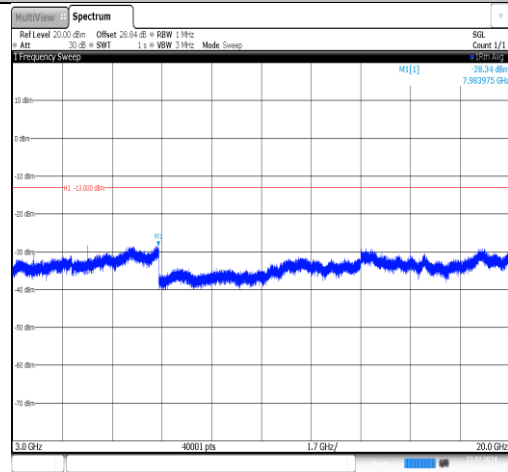
Band25-15MHz-16QAM-26115-1RB#0-3000~20000-PASS
