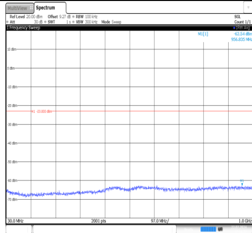
Band25-3MHz-QPSK-26365-1RB#0-30~1000-PASS
