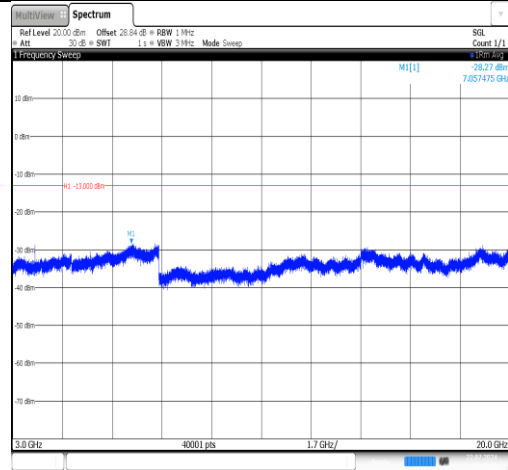
Band25-3MHz-QPSK-26365-1RB#0-3000~20000-PASS
