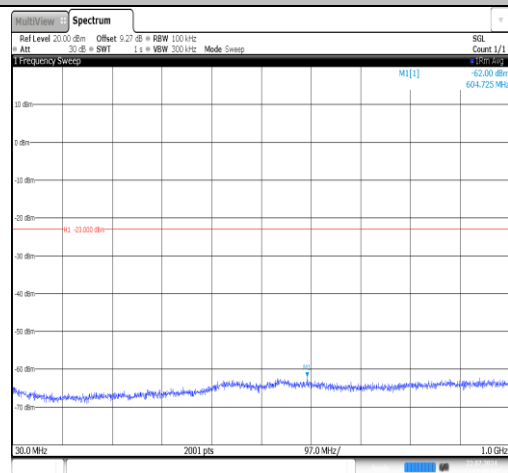
Band25-20MHz-16QAM-26140-1RB#0-30~1000-PASS
