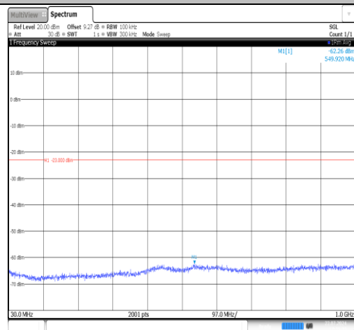
Band25-15MHz-16QAM-26615-1RB#0-30~1000-PASS
