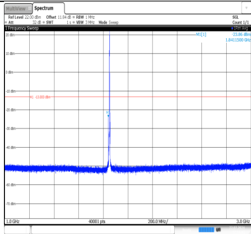
Band25-3MHz-16QAM-26055-1RB#0-1000~3000-PASS
