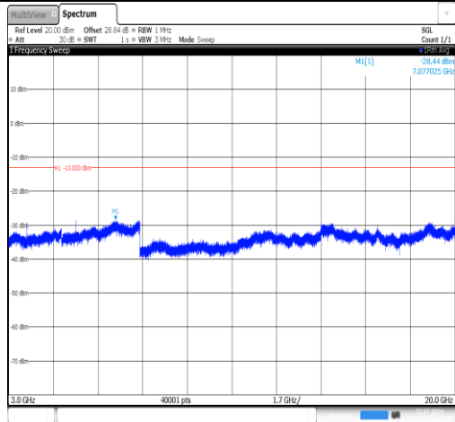
Band25-3MHz-QPSK-26055-1RB#0-3000~20000-PASS
