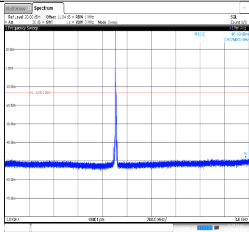
Band25-10MHz-16QAM-26640-1RB#0-1000~3000-PASS
