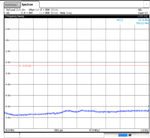
Band25-10MHz-16QAM-26090-1RB#0-30~1000-PASS
