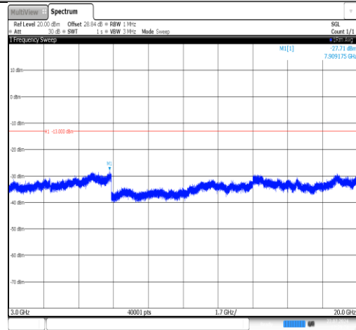
Band25-10MHz-16QAM-26640-1RB#0-3000~20000-PASS
