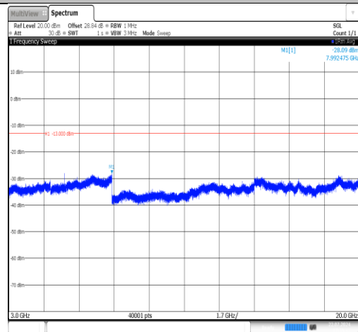
Band25-15MHz-16QAM-26615-1RB#0-3000~20000-PASS
