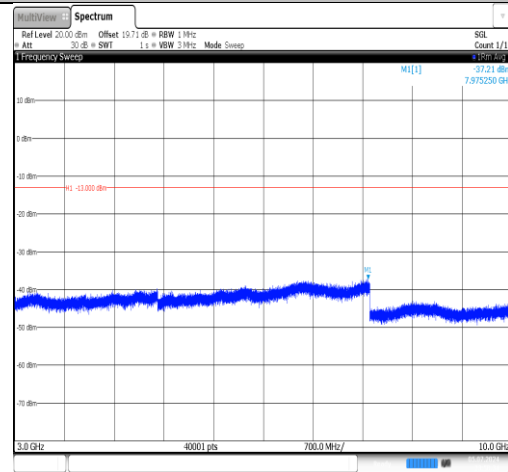
Band12-10MHz-16QAM-23060-1RB#0-3000~10000-PASS
