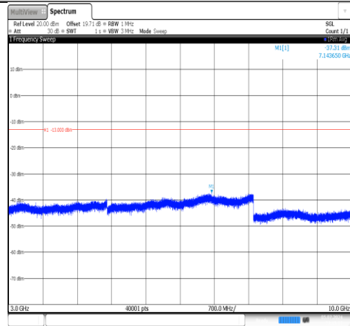
Band12-3MHz-QPSK-23095-1RB#0-3000~10000-PASS
