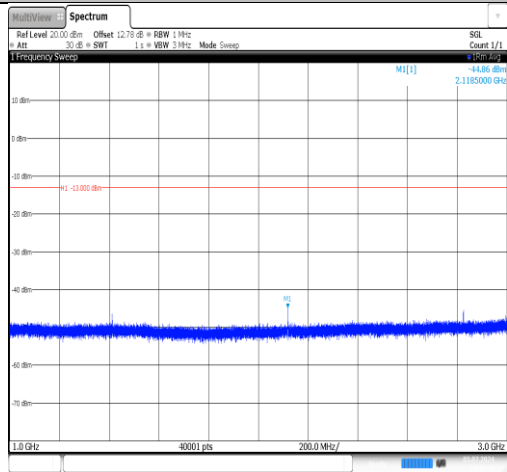
Band12-3MHz-QPSK-23095-1RB#0-1000~3000-PASS
