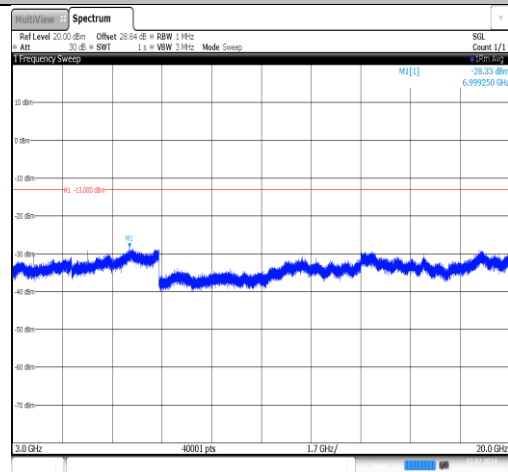
Band25-20MHz-16QAM-26140-1RB#0-3000~20000-PASS
