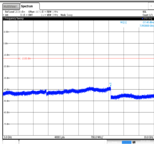
Band5-3MHz-QPSK-20635-1RB#0-3000~10000-PASS
