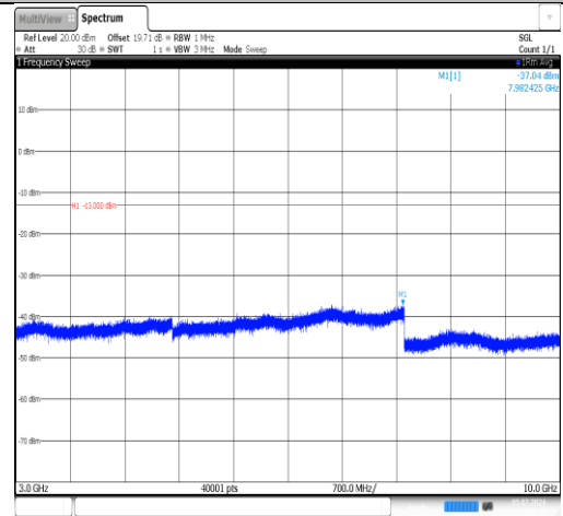
Band5-5MHz-16QAM-20625-1RB#0-3000~10000-PASS
