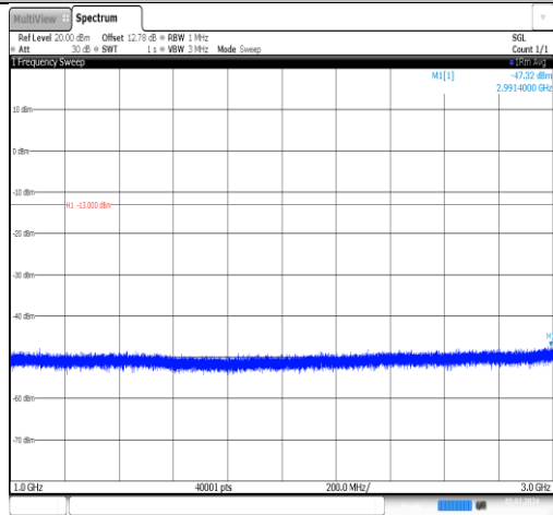
Band12-1.4MHz-16QAM-23173-1RB#0-1000~3000-PASS
