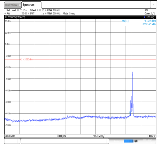
Band5-5MHz-16QAM-20625-1RB#0-30~1000-PASS
