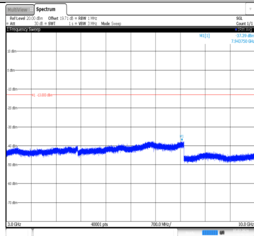
Band5-3MHz-16QAM-20415-1RB#0-3000~10000-PASS
