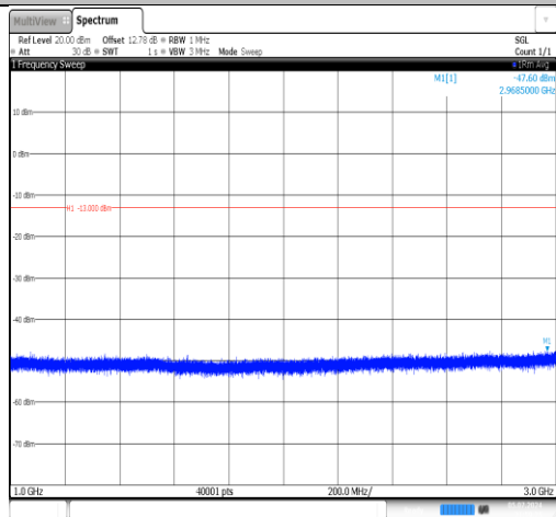
Band5-3MHz-16QAM-20415-1RB#0-1000~3000-PASS
