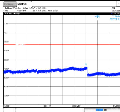
Band12-1.4MHz-16QAM-23173-1RB#0-3000~10000-PASS
