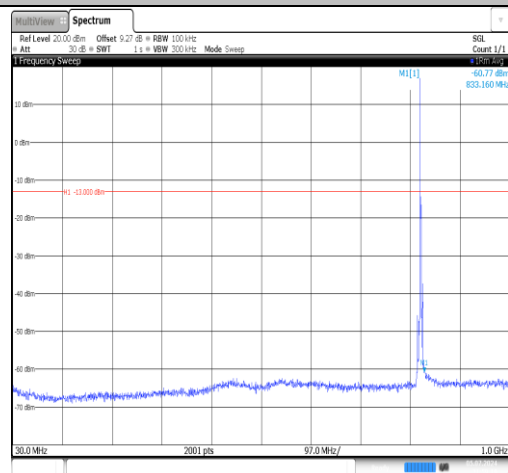
Band5-3MHz-16QAM-20415-1RB#0-30~1000-PASS
