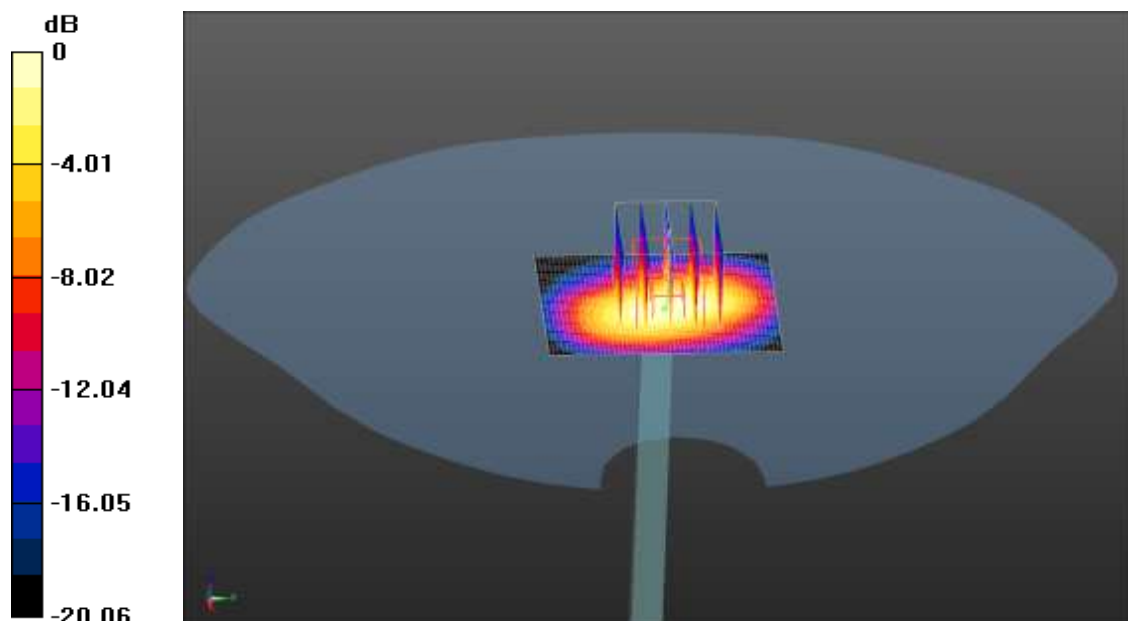
0 dB = 2.33W/kg = 3.67 dBW/kg
