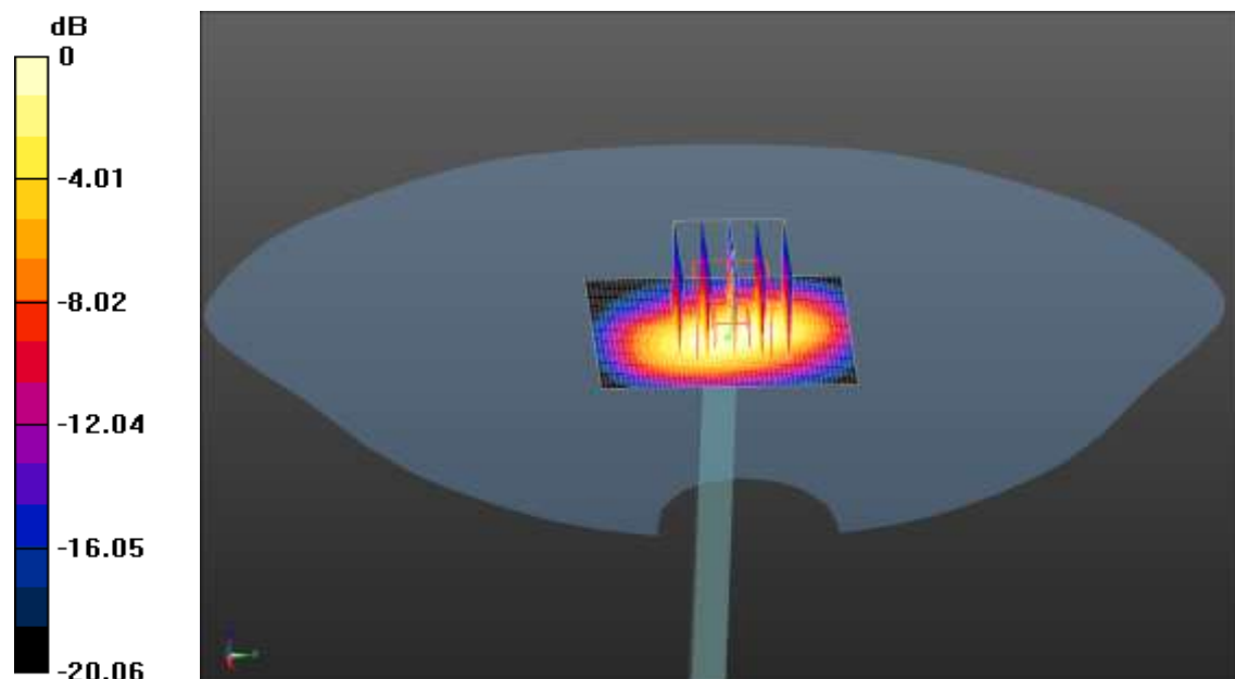
0 dB = 2.29 W/kg = 3.60dBW/kg
