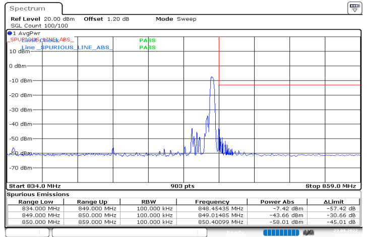
n5_15MHz_15kHz_841.5MHz_DFT-s-OFDM QPSK_RB1@78
