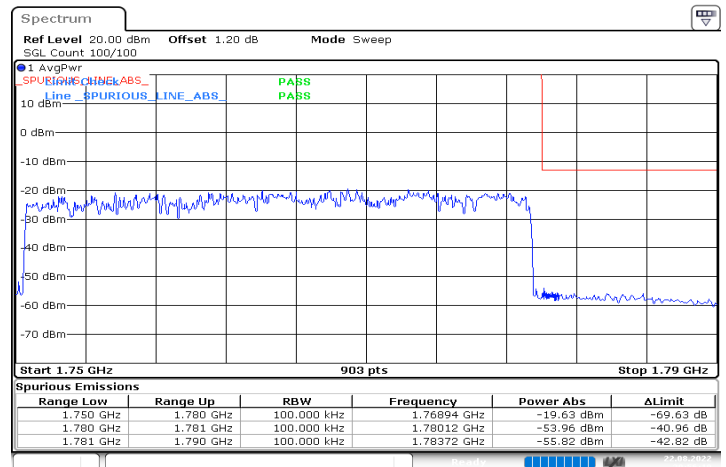
n66_30MHz_15kHz_1765MHz_DFT-s-OFDM QPSK_RB160@0
