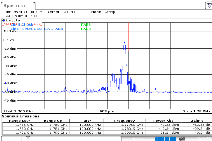
n66_15MHz_15kHz_1772.5MHz_DFT-s-OFDM QPSK_RB1@78
