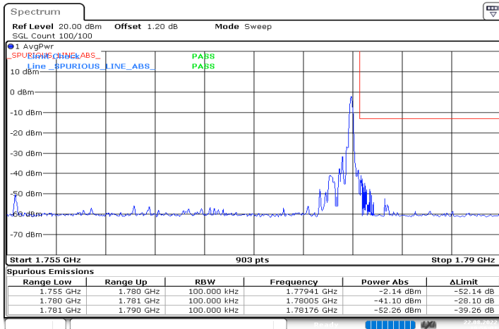
n66_25MHz_15kHz_1767.5MHz_DFT-s-OFDM QPSK_RB1@132
