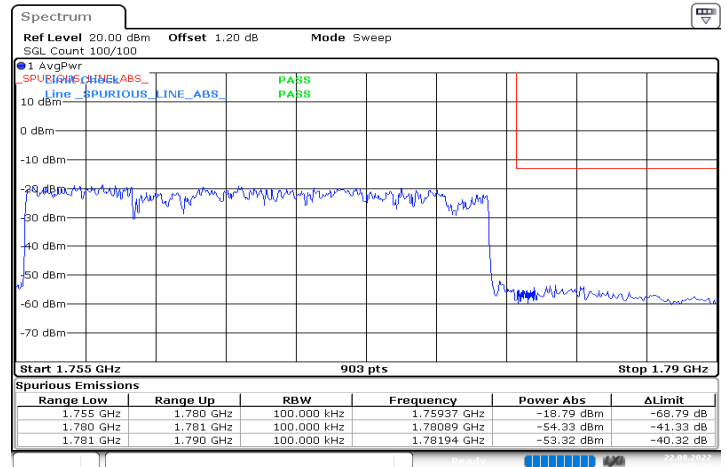
n66_25MHz_15kHz_1767.5MHz_DFT-s-OFDM QPSK_RB128@0
