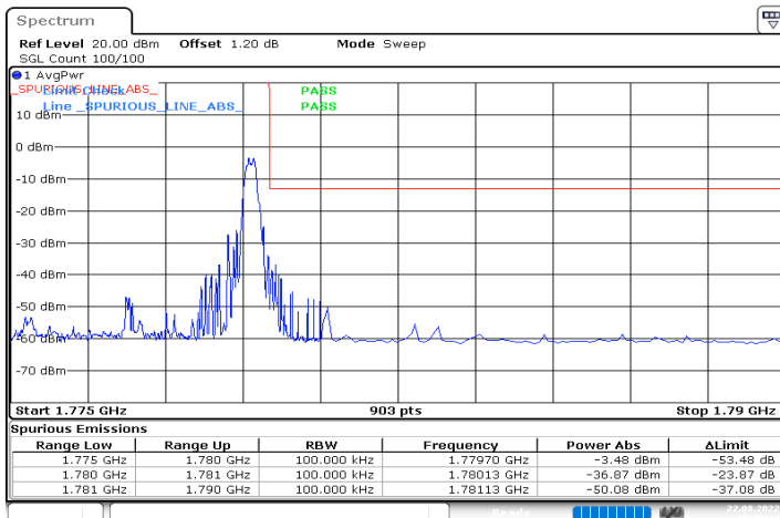
n66_5MHz_15kHz_1777.5MHz_DFT-s-OFDM QPSK_RB1@24
