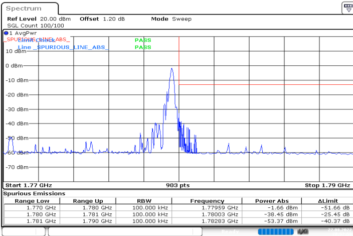
n66_10MHz_15kHz_1775MHz_DFT-s-OFDM QPSK_RB1@51
