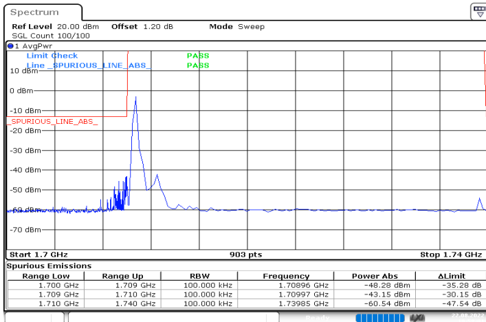
n66_30MHz_15kHz_1725MHz_DFT-s-OFDM QPSK_RB1@0
