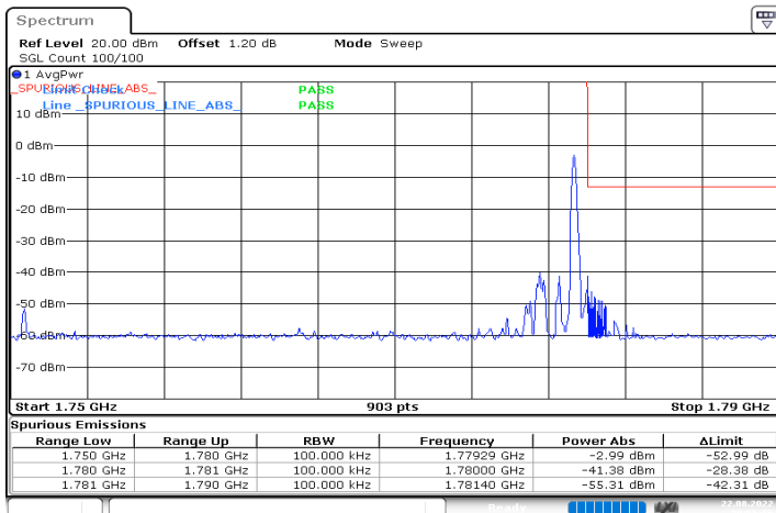
n66_30MHz_15kHz_1765MHz_DFT-s-OFDM QPSK_RB1@159
