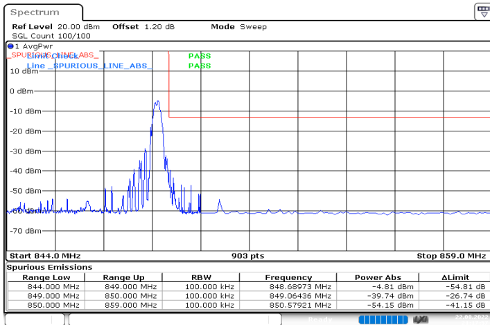
n5_5MHz_15kHz_846.5MHz_DFT-s-OFDM QPSK_RB1@24
