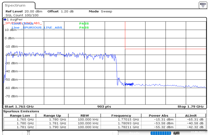
n66_15MHz_15kHz_1772.5MHz_DFT-s-OFDM QPSK_RB75@0
