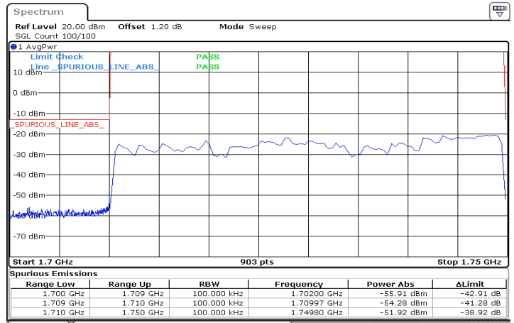
n66_40MHz_15kHz_1730MHz_DFT-s-OFDM QPSK_RB216@0
