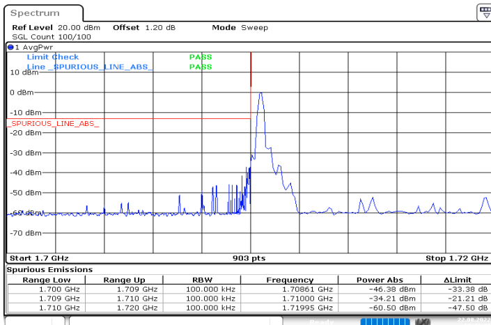
n66_10MHz_15kHz_1715MHz_DFT-s-OFDM QPSK_RB1@0
