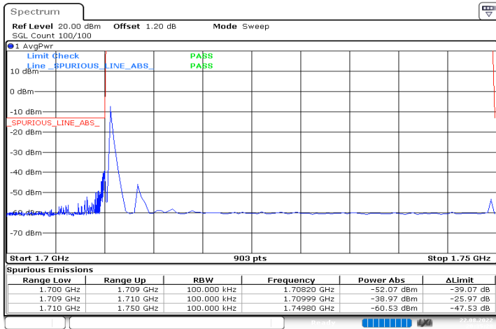
n66_40MHz_15kHz_1730MHz_DFT-s-OFDM QPSK_RB1@0
