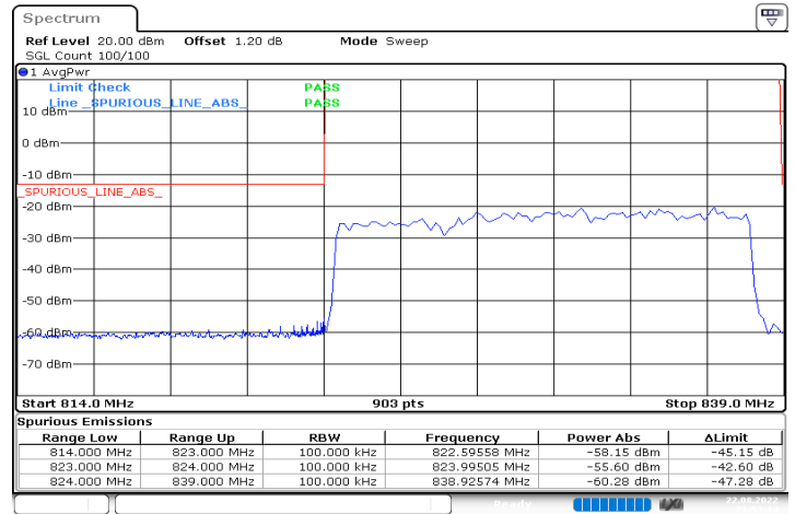
n5_15MHz_15kHz_831.5MHz_DFT-s-OFDM QPSK_RB75@0
