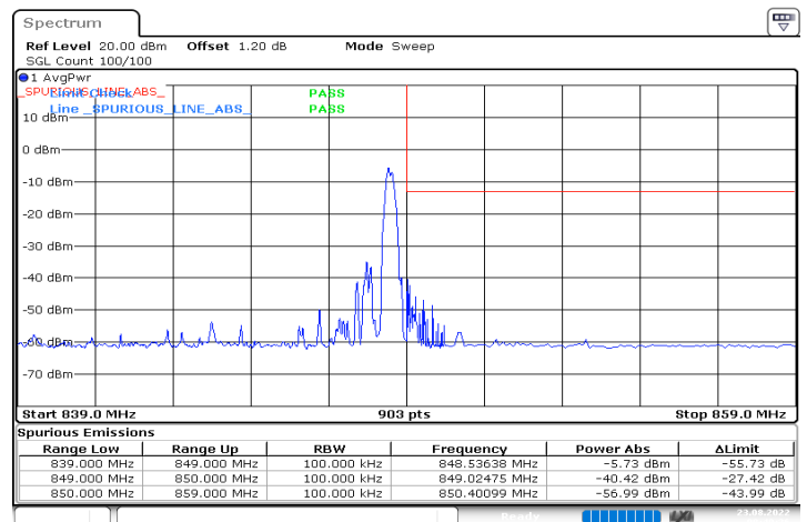
n5_10MHz_15kHz_844MHz_DFT-s-OFDM QPSK_RB1@51
