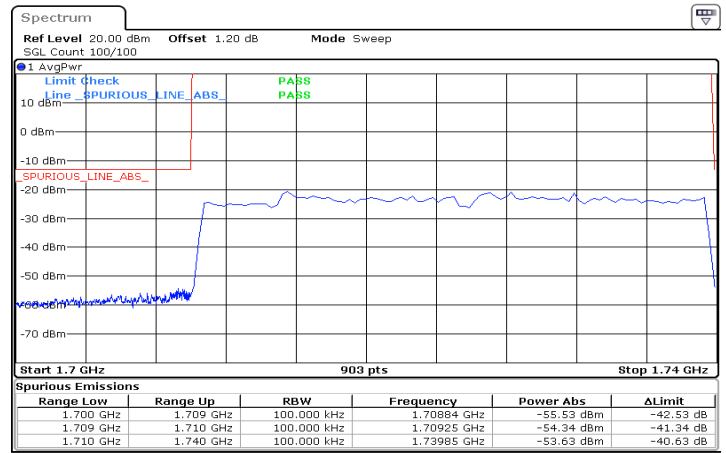
n66_30MHz_15kHz_1725MHz_DFT-s-OFDM QPSK_RB160@0
