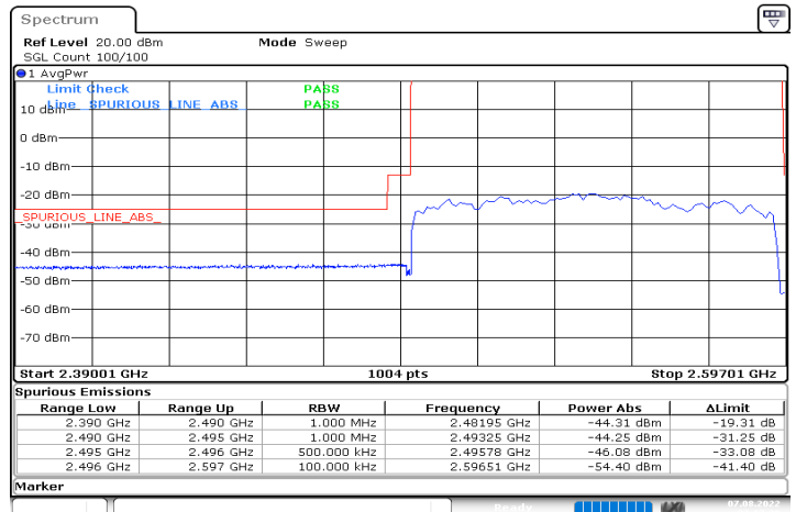
DC_2A_n41A_10MHz|100MHz_30kHz_1880MHz|2546.01MHz_DFT-s-OFDM QPSK_RB0|RB270@0
