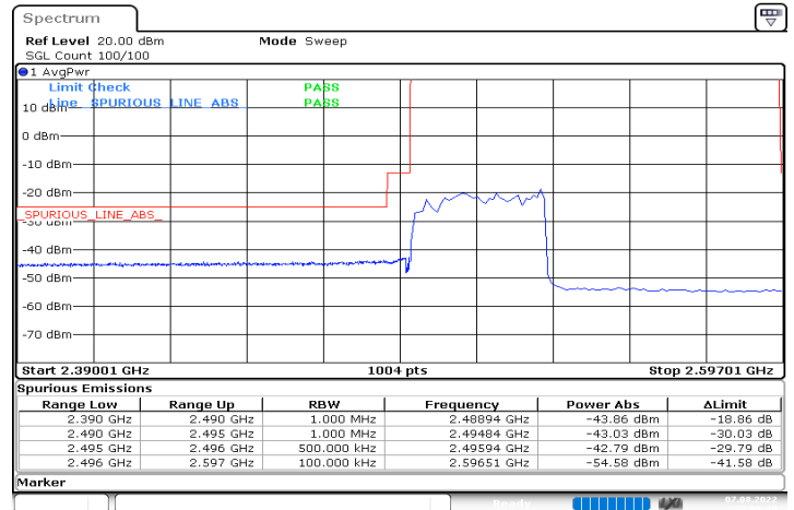
DC_2A_n41A_10MHz|40MHz_30kHz_1880MHz|2516.01MHz_DFT-s-OFDM QPSK_RB0|RB100@0
