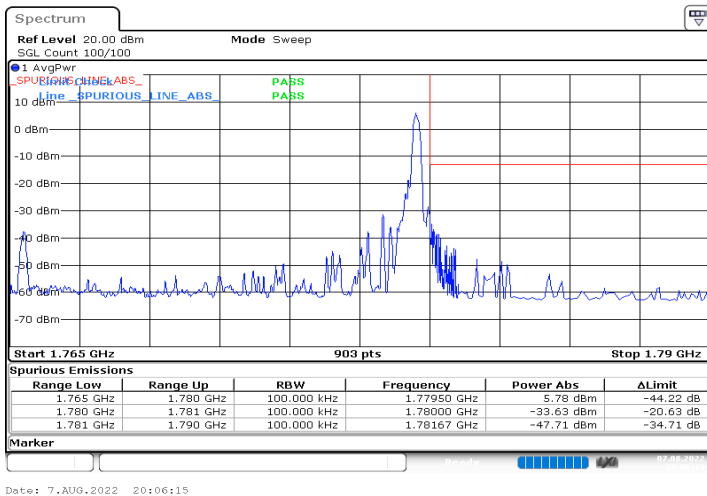
DC_12A_n66A_10MHz|15MHz_15kHz_707.5MHz|1772.5MHz_DFT-s-OFDM QPSK_RB0|RB1@78
