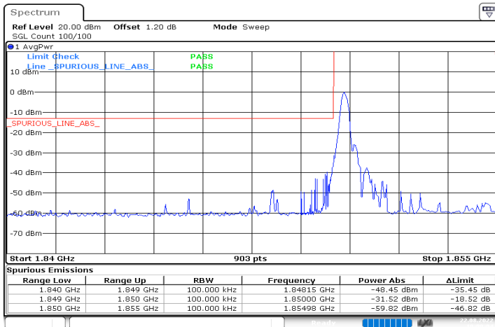
n25_5MHz_15kHz_1852.5MHz_DFT-s-OFDM QPSK_RB1@0
