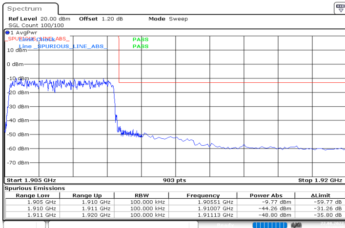
n2_5MHz_15kHz_1907.5MHz_DFT-s-OFDM QPSK_RB25@0
