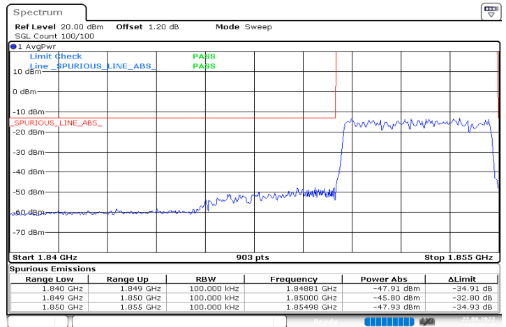
n2_5MHz_15kHz_1852.5MHz_DFT-s-OFDM QPSK_RB25@0
