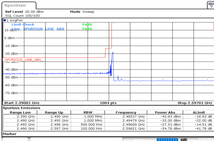
DC_2A_n41A_10MHz|100MHz_30kHz_1880MHz|2546.01MHz_DFT-s-OFDM QPSK_RB0|RB1@0
