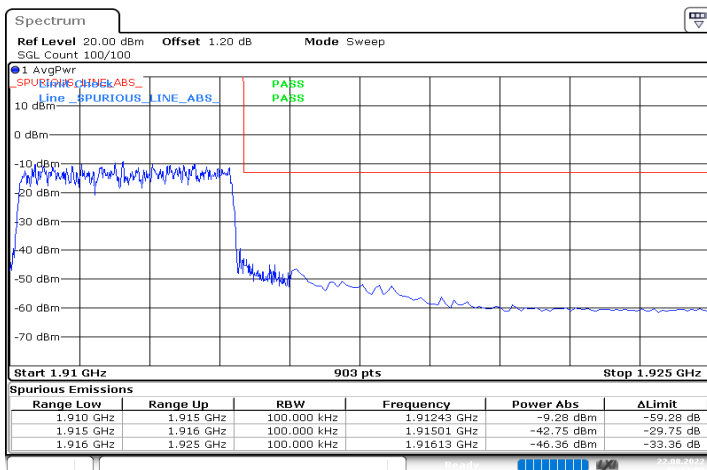
n25_5MHz_15kHz_1912.5MHz_DFT-s-OFDM QPSK_RB25@0
