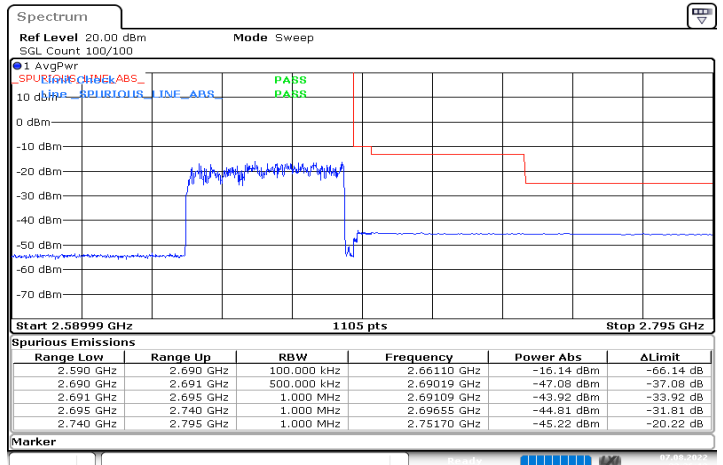
DC_66A_n41A_10MHz|50MHz_30kHz_1745MHz|2664.99MHz_DFT-s-OFDM QPSK_RB0|RB128@0
