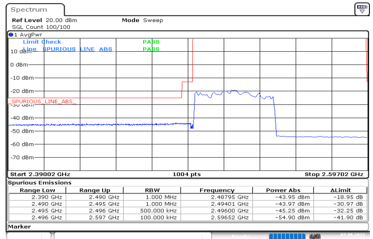
DC_2A_n41A_10MHz|50MHz_30kHz_1880MHz|2521.02MHz_DFT-s-OFDM QPSK_RB0|RB128@0
