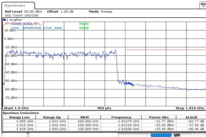
n25_15MHz_15kHz_1907.5MHz_DFT-s-OFDM QPSK_RB75@0
