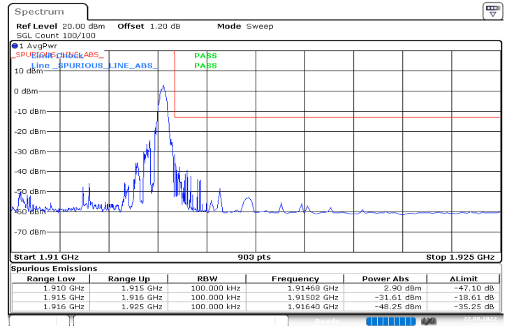
n25_5MHz_15kHz_1912.5MHz_DFT-s-OFDM QPSK_RB1@24
