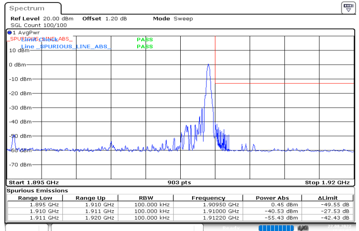
n2_15MHz_15kHz_1902.5MHz_DFT-s-OFDM QPSK_RB1@78
