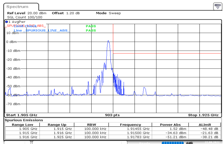
n25_10MHz_15kHz_1910MHz_DFT-s-OFDM QPSK_RB1@51
