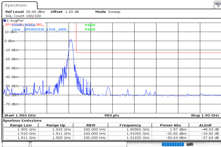
n2_5MHz_15kHz_1907.5MHz_DFT-s-OFDM QPSK_RB1@24
