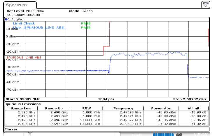
DC_2A_n41A_10MHz|80MHz_30kHz_1880MHz|2536.02MHz_DFT-s-OFDM QPSK_RB0|RB216@0
