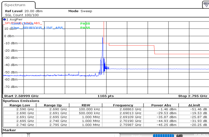
DC_66A_n41A_10MHz|50MHz_30kHz_1745MHz|2664.99MHz_DFT-s-OFDM QPSK_RB0|RB1@132
