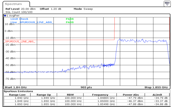
n25_5MHz_15kHz_1852.5MHz_DFT-s-OFDM QPSK_RB25@0
