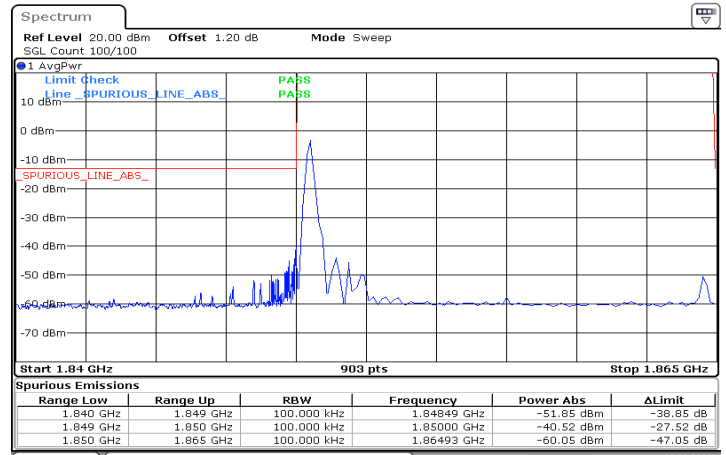
n25_15MHz_15kHz_1857.5MHz_DFT-s-OFDM QPSK_RB1@0
