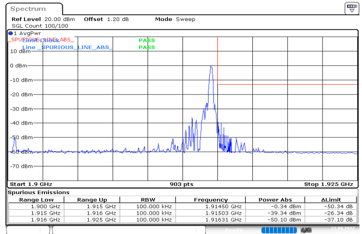
n25_15MHz_15kHz_1907.5MHz_DFT-s-OFDM QPSK_RB1@78
