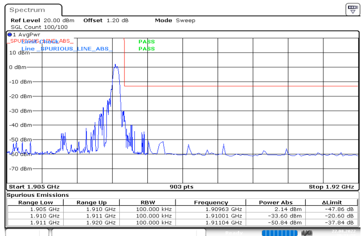
n2_5MHz_15kHz_1907.5MHz_DFT-s-OFDM QPSK_RB1@24
