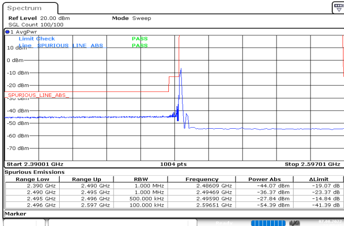
DC_2A_n41A_10MHz|40MHz_30kHz_1880MHz|2516.01MHz_DFT-s-OFDM QPSK_RB0|RB1@0
