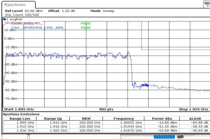
n25_20MHz_15kHz_1905MHz_DFT-s-OFDM QPSK_RB100@0
