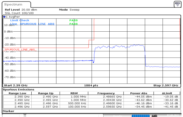
DC_66A_n41A_10MHz|60MHz_30kHz_1745MHz|2526MHz_DFT-s-OFDM QPSK_RB0|RB162@0
