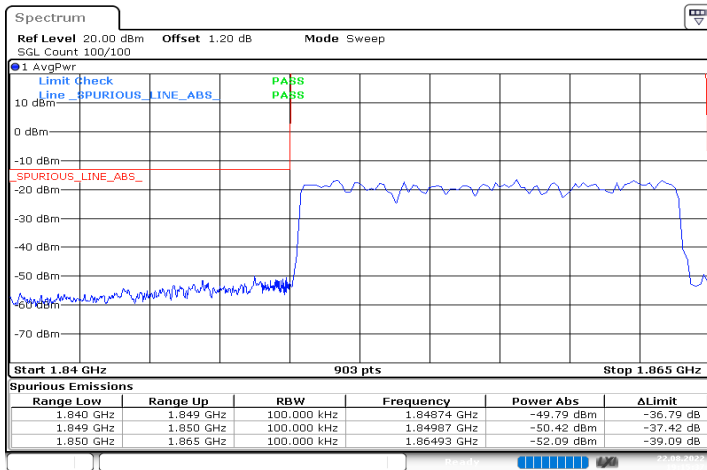
n25_15MHz_15kHz_1857.5MHz_DFT-s-OFDM QPSK_RB75@0
