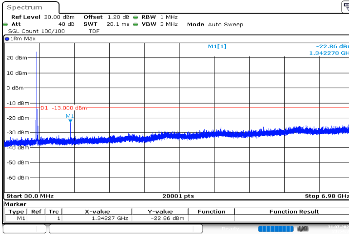
n71_20MHz_15kHz_680.5MHz_DFT-s-OFDM QPSK_RB1@0|30MHz_6.98GHz
