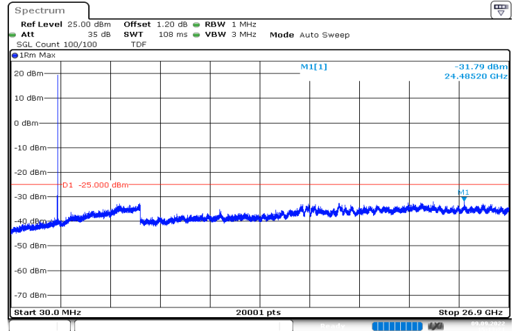
n41_50MHz_30kHz_2521.02MHz_DFT-s-OFDM QPSK_RB1@132|30MHz_26.9GHz
