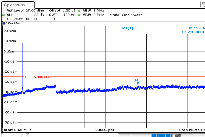
n41_50MHz_30kHz_2664.99MHz_DFT-s-OFDM QPSK_RB128@0|30MHz_26.9GHz
