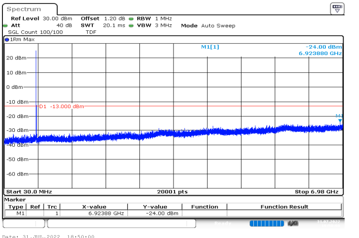
n71_5MHz_15kHz_680.5MHz_DFT-s-OFDM QPSK_RB1@24|30MHz_6.98GHz
