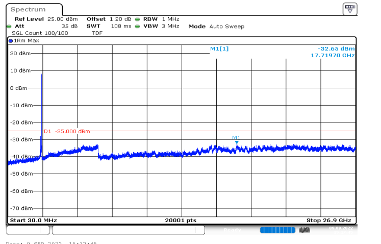
n41_50MHz_30kHz_2592.99MHz_DFT-s-OFDM QPSK_RB128@0|30MHz_26.9GHz
