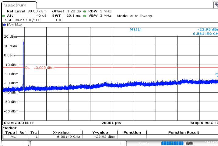
n71_20MHz_15kHz_680.5MHz_DFT-s-OFDM QPSK_RB100@0|30MHz_6.98GHz
