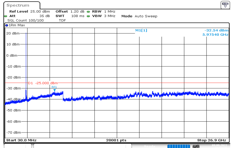
n41_100MHz_30kHz_2592.99MHz_DFT-s-OFDM_QPSK_RB1@0|30MHz_26.9GHz
