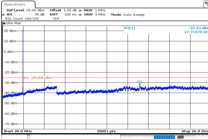
n41_15MHz_30kHz_2592.99MHz_DFT-s-OFDM QPSK_RB1@0|30MHz_26.9GHz
