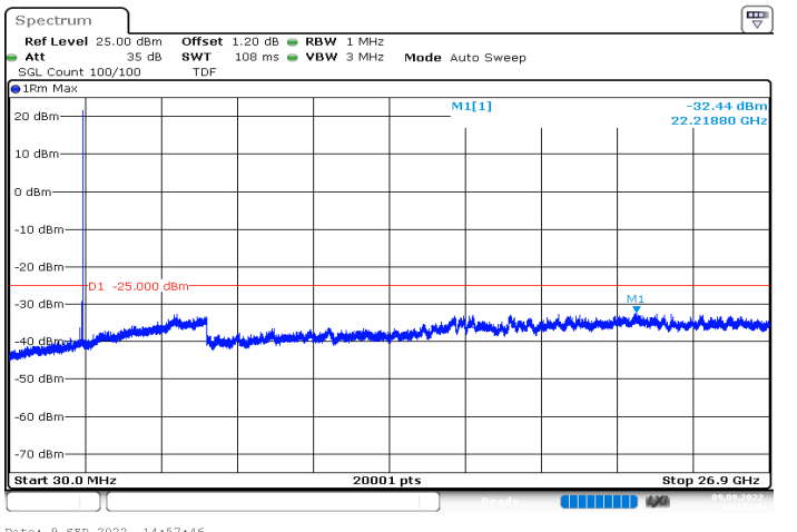
n41_20MHz_30kHz_2592.99MHz_DFT-s-OFDM QPSK_RB1@50|30MHz_26.9GHz
