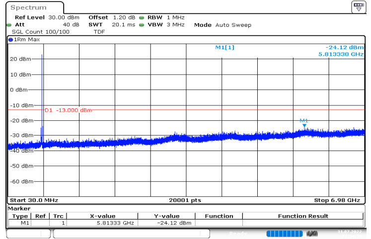
n71_20MHz_15kHz_680.5MHz_DFT-s-OFDM QPSK_RB1@105|30MHz_6.98GHz
