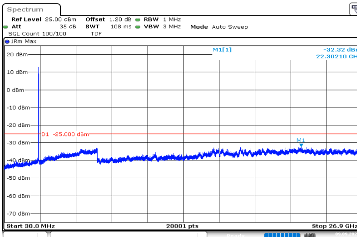
n41_15MHz_30kHz_2592.99MHz_DFT-s-OFDM QPSK_RB36@0|30MHz_26.9GHz
