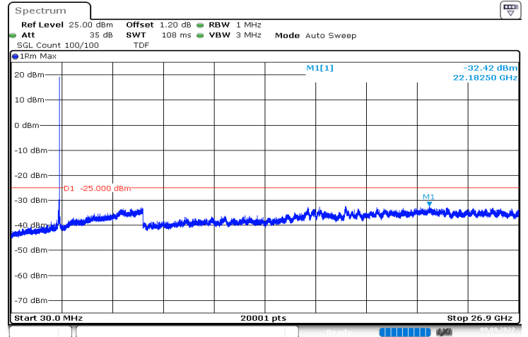
n41_100MHz_30kHz_2546.01MHz_DFT-s-OFDM_QPSK_RB1@272|30MHz_26.9GHz
