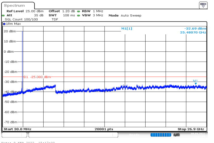
n41_50MHz_30kHz_2592.99MHz_DFT-s-OFDM QPSK_RB1@132|30MHz_26.9GHz
