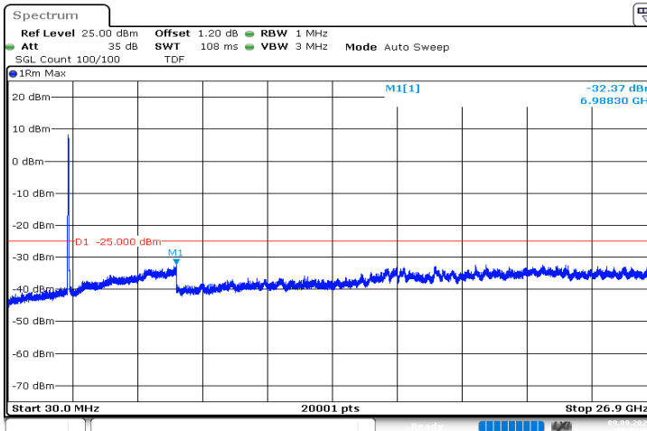
n41_50MHz_30kHz_2521.02MHz_DFT-s-OFDM QPSK_RB128@0|30MHz_26.9GHz
