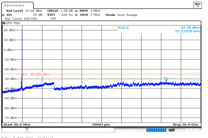
n41_100MHz_30kHz_2592.99MHz_DFT-s-OFDM_QPSK_RB1@272|30MHz_26.9GHz
