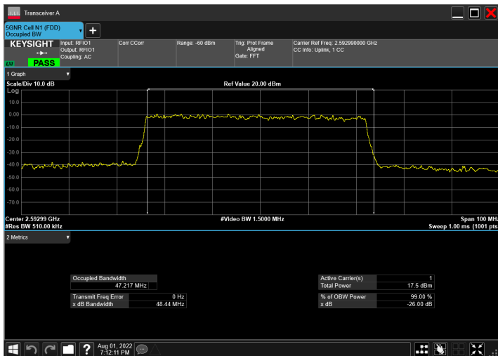
n41_50MHz_30kHz_2592.99MHz_DFT-s-OFDM 256 QAM_RB128@0
