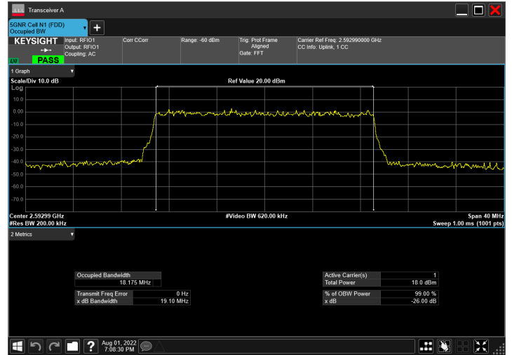
n41_20MHz_30kHz_2592.99MHz_CP-OFDM 64 QAM_RB51@0
