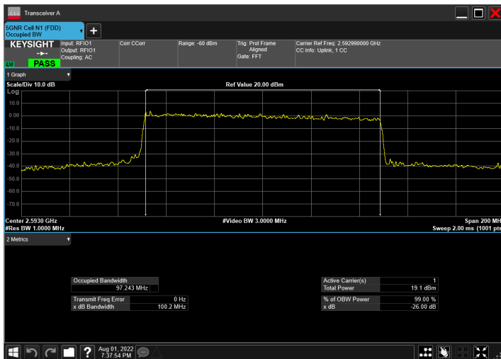
n41_100MHz_30kHz_2592.99MHz_CP-OFDM 64 QAM_RB273@0
