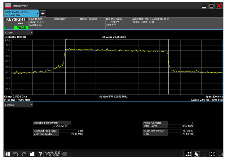
n41_100MHz_30kHz_2592.99MHz_DFT-s-OFDM 16 QAM_RB270@0
