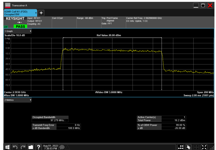
n41_100MHz_30kHz_2592.99MHz_CP-OFDM 256 QAM_RB273@0
