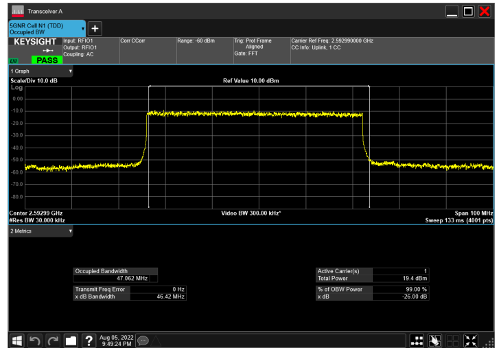
DC_66A_n41A_10MHz|50MHz_30kHz_1745MHz|2592.99MH z_QPSK|CP-OFDM 64 QAM_RB1@50|RB133@0
