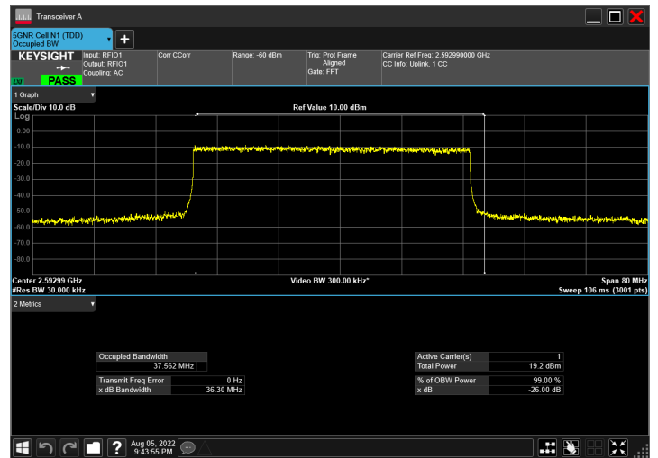
DC_66A_n41A_10MHz|40MHz_30kHz_1745MHz|2592.99MH z_QPSK|DFT-s-OFDM 16 QAM_RB1@50|RB100@0
