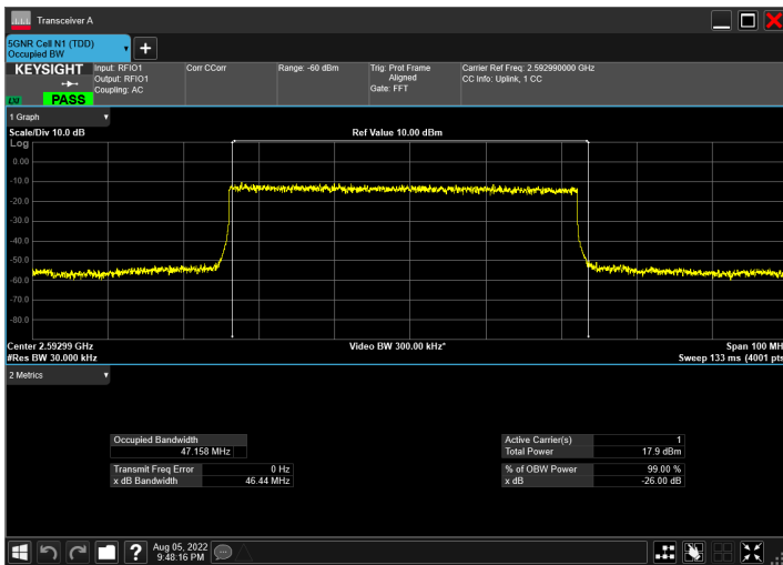
DC_66A_n41A_10MHz|50MHz_30kHz_1745MHz|2592.99MH z_QPSK|DFT-s-OFDM 256 QAM_RB1@50|RB128@0
