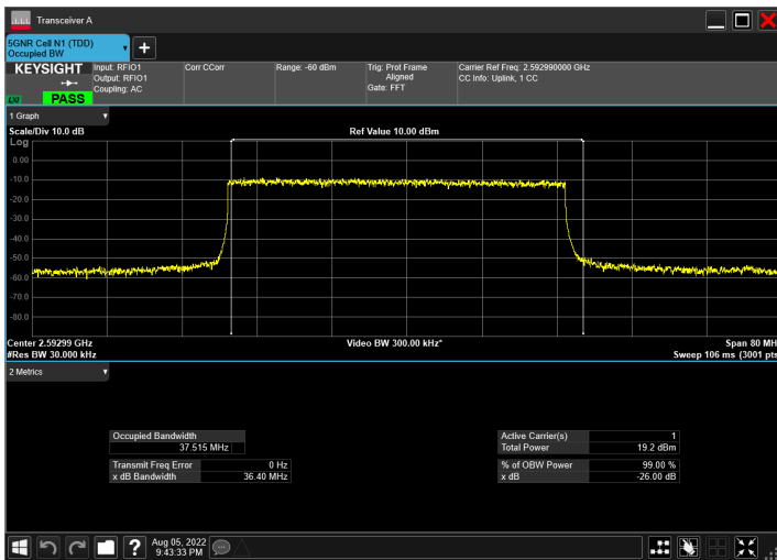
DC_66A_n41A_10MHz|40MHz_30kHz_1745MHz|2592.99MH z_QPSK|DFT-s-OFDM QPSK_RB1@50|RB100@0
