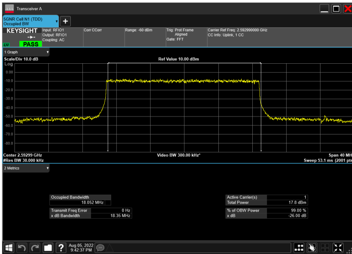
DC_66A_n41A_10MHz|20MHz_30kHz_1745MHz|2592.99MH z_QPSK|CP-OFDM 256 QAM_RB1@50|RB51@0
