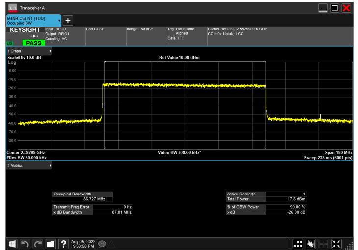
DC_66A_n41A_10MHz|90MHz_30kHz_1745MHz|2592.99MH z_QPSK|DFT-s-OFDM 256 QAM_RB1@50|RB243@0
