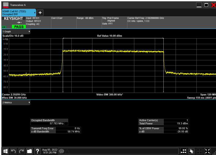
DC_66A_n41A_10MHz|60MHz_30kHz_1745MHz|2592.99MH z_QPSK|DFT-s-OFDM 64 QAM_RB1@50|RB162@0
