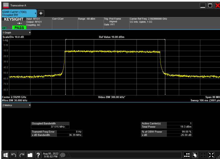
DC_66A_n41A_10MHz|40MHz_30kHz_1745MHz|2592.99MH z_QPSK|CP-OFDM QPSK_RB1@50|RB106@0
