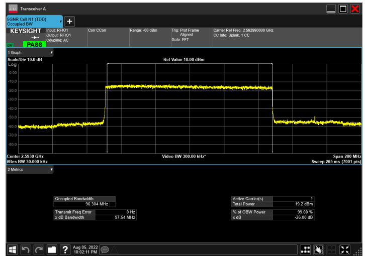
DC_66A_n41A_10MHz|100MHz_30kHz_1745MHz|2592.99M Hz_QPSK|DFT-s-OFDM 64 QAM_RB1@50|RB270@0
