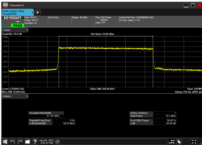
DC_66A_n41A_10MHz|60MHz_30kHz_1745MHz|2592.99MH z_QPSK|CP-OFDM 64 QAM_RB1@50|RB162@0
