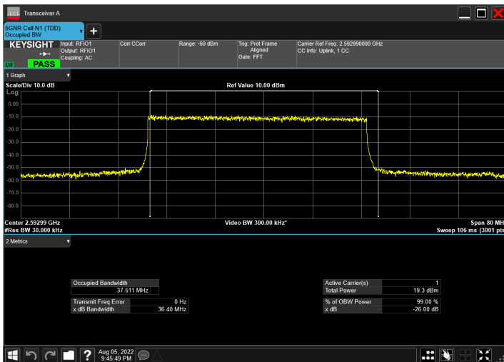
DC_66A_n41A_10MHz|40MHz_30kHz_1745MHz|2592.99MH z_QPSK|CP-OFDM 64 QAM_RB1@50|RB106@0
