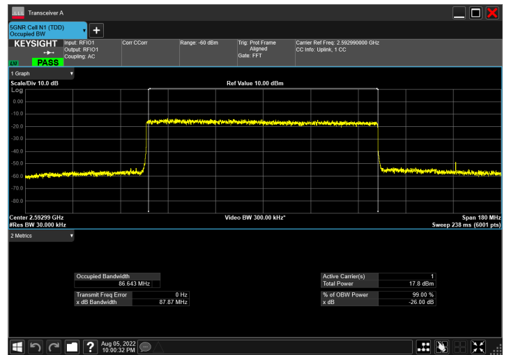
DC_66A_n41A_10MHz|90MHz_30kHz_1745MHz|2592.99MH z_QPSK|CP-OFDM 256 QAM_RB1@50|RB245@0
