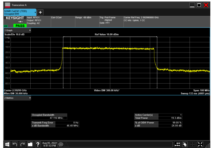
DC_66A_n41A_10MHz|50MHz_30kHz_1745MHz|2592.99MH z_QPSK|DFT-s-OFDM 64 QAM_RB1@50|RB128@0
