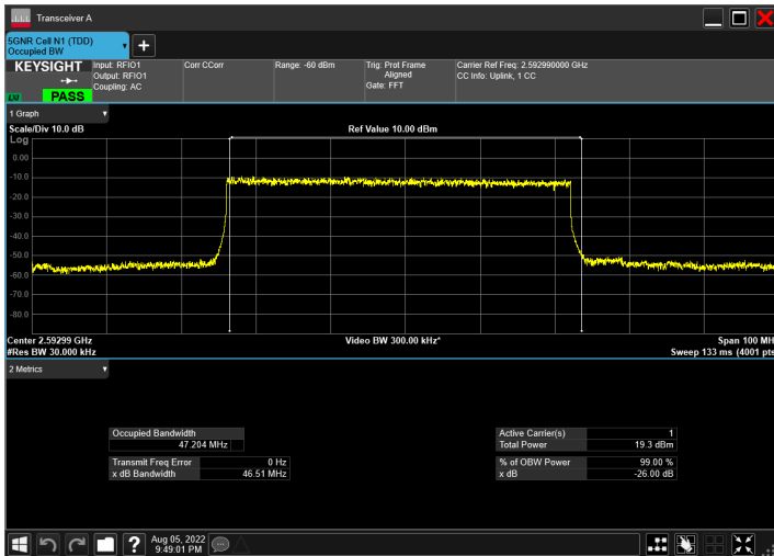
DC_66A_n41A_10MHz|50MHz_30kHz_1745MHz|2592.99MH z_QPSK|CP-OFDM 16 QAM_RB1@50|RB133@0
