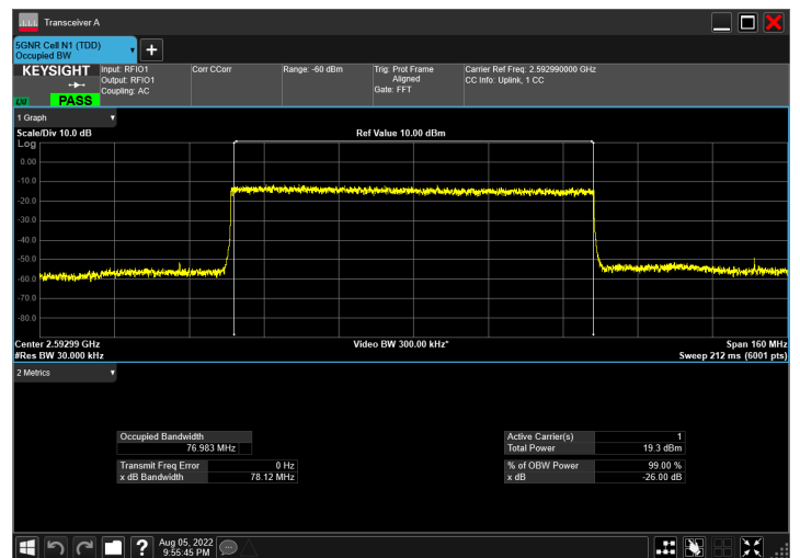
DC_66A_n41A_10MHz|80MHz_30kHz_1745MHz|2592.99MH z_QPSK|CP-OFDM QPSK_RB1@50|RB217@0
