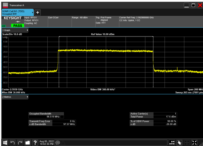
DC_66A_n41A_10MHz|100MHz_30kHz_1745MHz|2592.99M Hz_QPSK|DFT-s-OFDM 256 QAM_RB1@50|RB270@0
