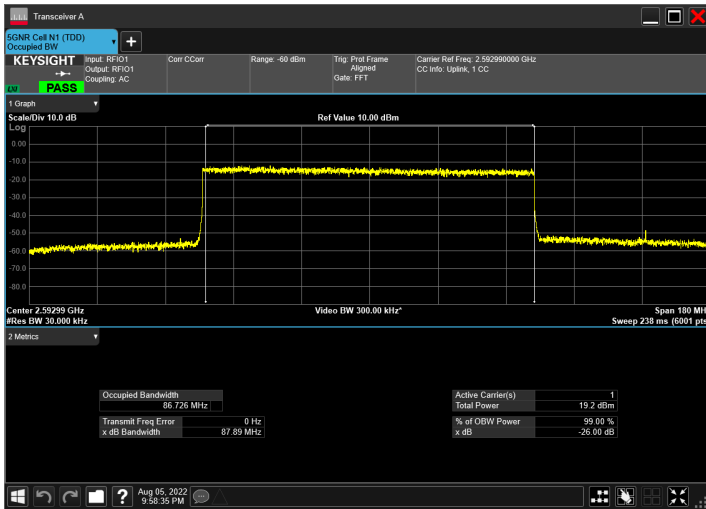
DC_66A_n41A_10MHz|90MHz_30kHz_1745MHz|2592.99MH z_QPSK|DFT-s-OFDM 64 QAM_RB1@50|RB243@0
