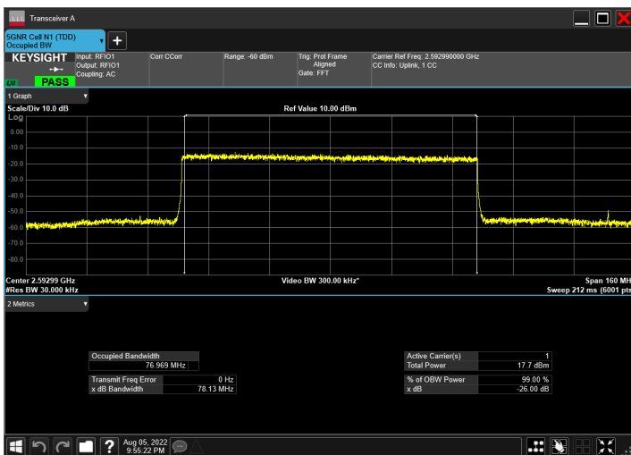
DC_66A_n41A_10MHz|80MHz_30kHz_1745MHz|2592.99MH z_QPSK|DFT-s-OFDM 256 QAM_RB1@50|RB216@0
