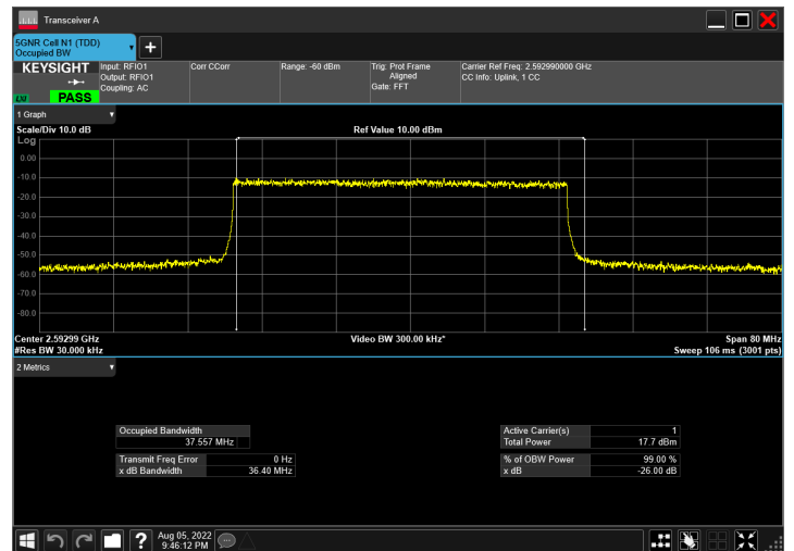
DC_66A_n41A_10MHz|40MHz_30kHz_1745MHz|2592.99MH z_QPSK|CP-OFDM 256 QAM_RB1@50|RB106@0
