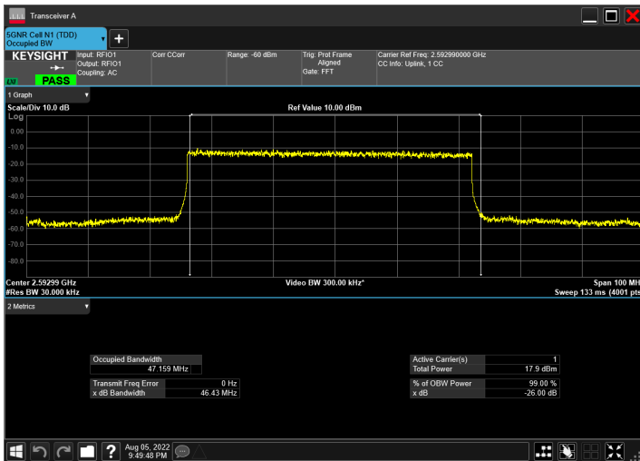
DC_66A_n41A_10MHz|50MHz_30kHz_1745MHz|2592.99MH z_QPSK|CP-OFDM 256 QAM_RB1@50|RB133@0
