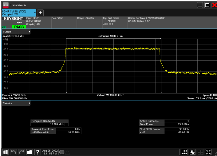
DC_66A_n41A_10MHz|20MHz_30kHz_1745MHz|2592.99MH z_QPSK|CP-OFDM 16 QAM_RB1@50|RB51@0
