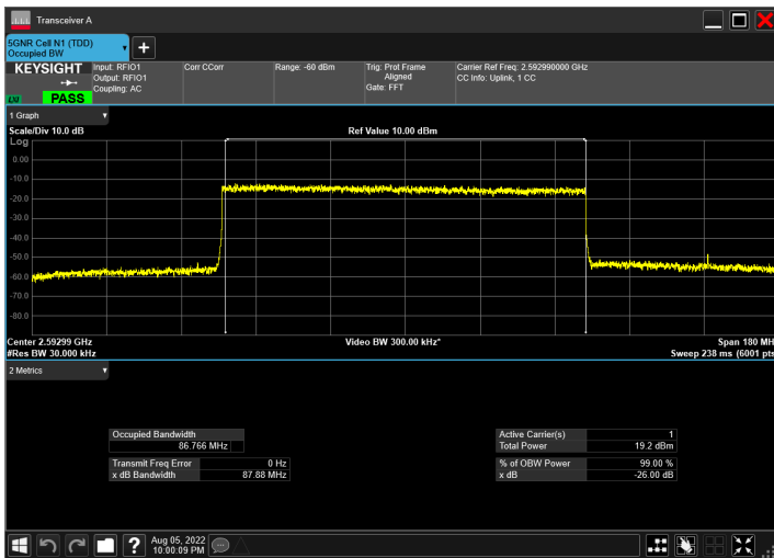
DC_66A_n41A_10MHz|90MHz_30kHz_1745MHz|2592.99MH z_QPSK|CP-OFDM 64 QAM_RB1@50|RB245@0
