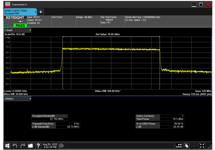
DC_66A_n41A_10MHz|60MHz_30kHz_1745MHz|2592.99MH z_QPSK|CP-OFDM 16 QAM_RB1@50|RB162@0
