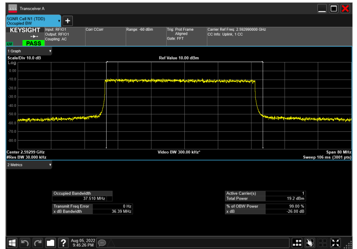
DC_66A_n41A_10MHz|40MHz_30kHz_1745MHz|2592.99MH z_QPSK|CP-OFDM 16 QAM_RB1@50|RB106@0
