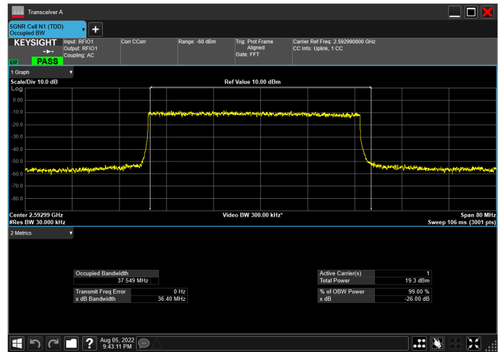
DC_66A_n41A_10MHz|40MHz_30kHz_1745MHz|2592.99MH z_QPSK|DFT-s-OFDM PI/2 BPSK_RB1@50|RB100@0
