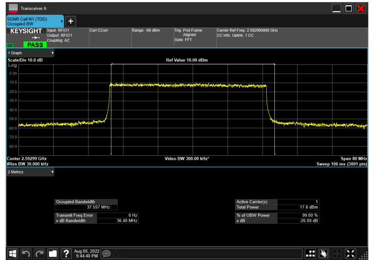
DC_66A_n41A_10MHz|40MHz_30kHz_1745MHz|2592.99MH z_QPSK|DFT-s-OFDM 256 QAM_RB1@50|RB100@0
