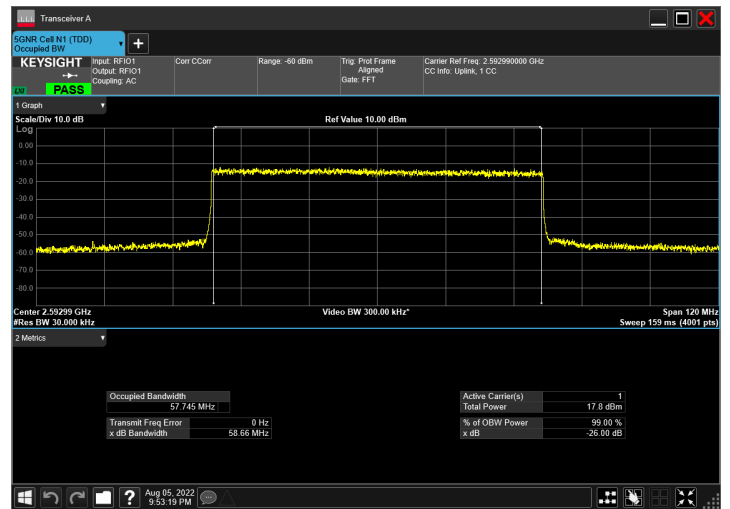
DC_66A_n41A_10MHz|60MHz_30kHz_1745MHz|2592.99MH z_QPSK|CP-OFDM 256 QAM_RB1@50|RB162@0
