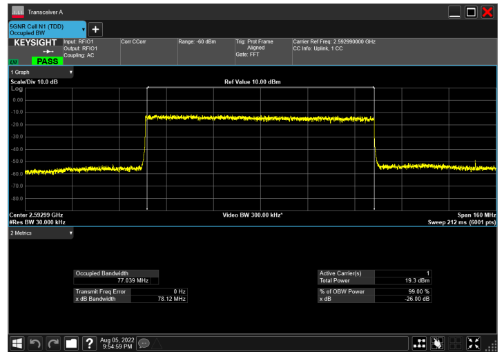
DC_66A_n41A_10MHz|80MHz_30kHz_1745MHz|2592.99MH z_QPSK|DFT-s-OFDM 64 QAM_RB1@50|RB216@0
