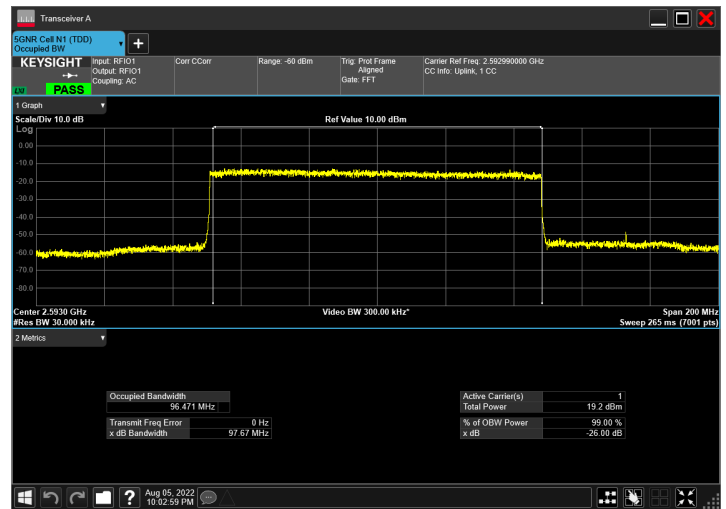
DC_66A_n41A_10MHz|100MHz_30kHz_1745MHz|2592.99M Hz_QPSK|CP-OFDM QPSK_RB1@50|RB273@0
