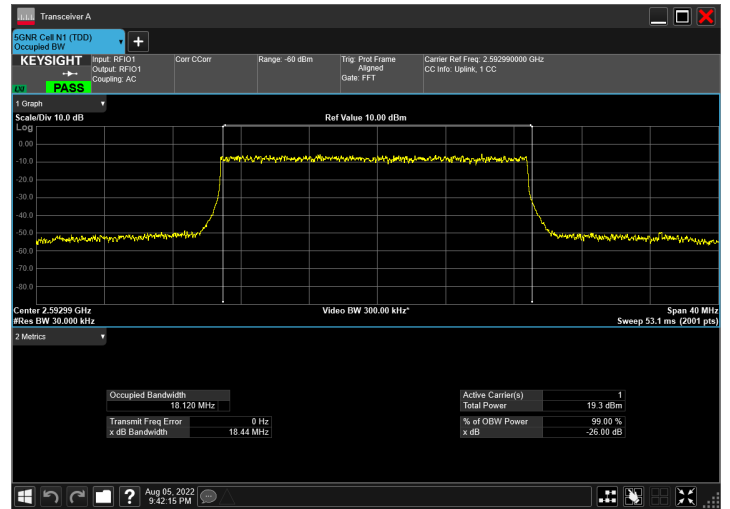
DC_66A_n41A_10MHz|20MHz_30kHz_1745MHz|2592.99MH z_QPSK|CP-OFDM 64 QAM_RB1@50|RB51@0
