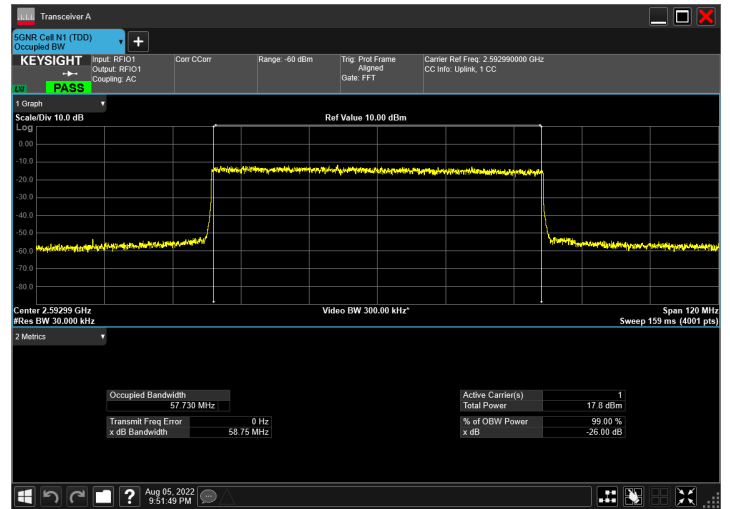
DC_66A_n41A_10MHz|60MHz_30kHz_1745MHz|2592.99MH z_QPSK|DFT-s-OFDM 256 QAM_RB1@50|RB162@0
