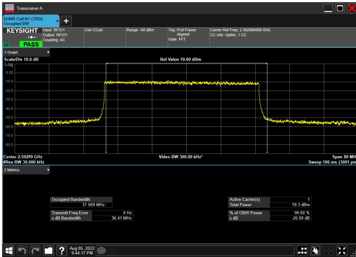
DC_66A_n41A_10MHz|40MHz_30kHz_1745MHz|2592.99MH z_QPSK|DFT-s-OFDM 64 QAM_RB1@50|RB100@0
