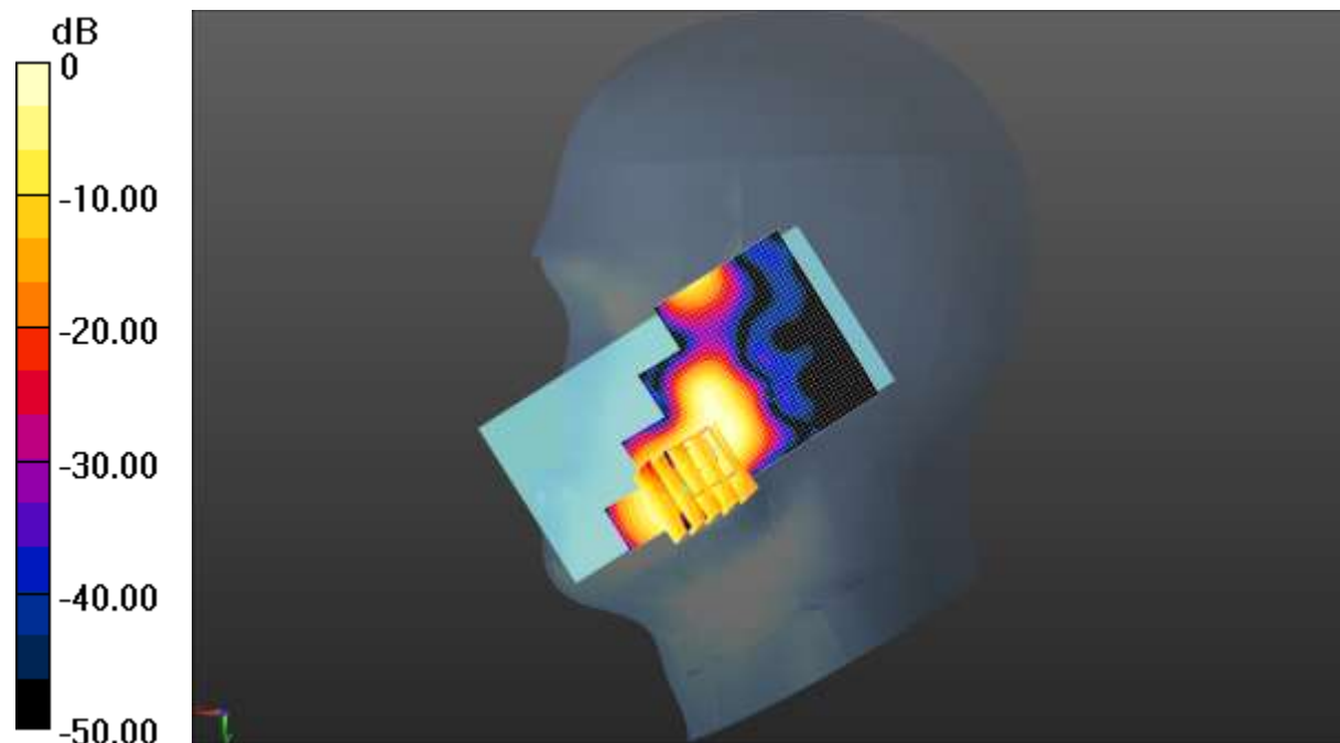
0 dB = 0.0226 W/kg = -16.46 dBW/kg
