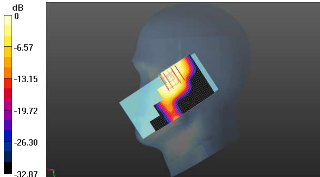
0 dB = 0.0488 W/kg = -13.12 dBW/kg
