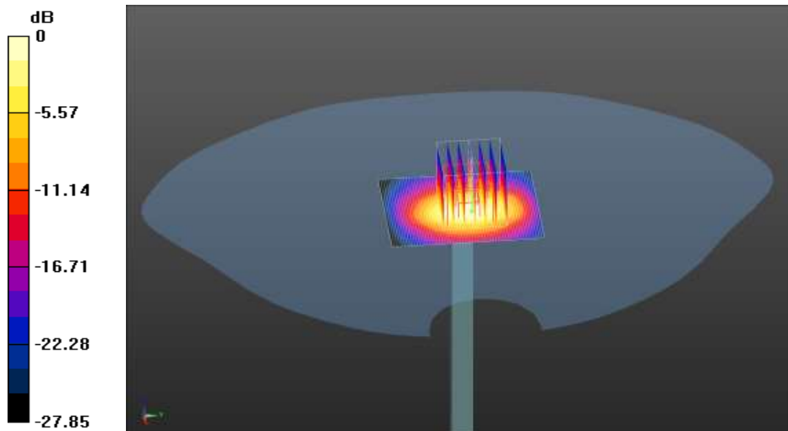
0 dB = 3.99 W/kg = 6.01 dBW/kg
