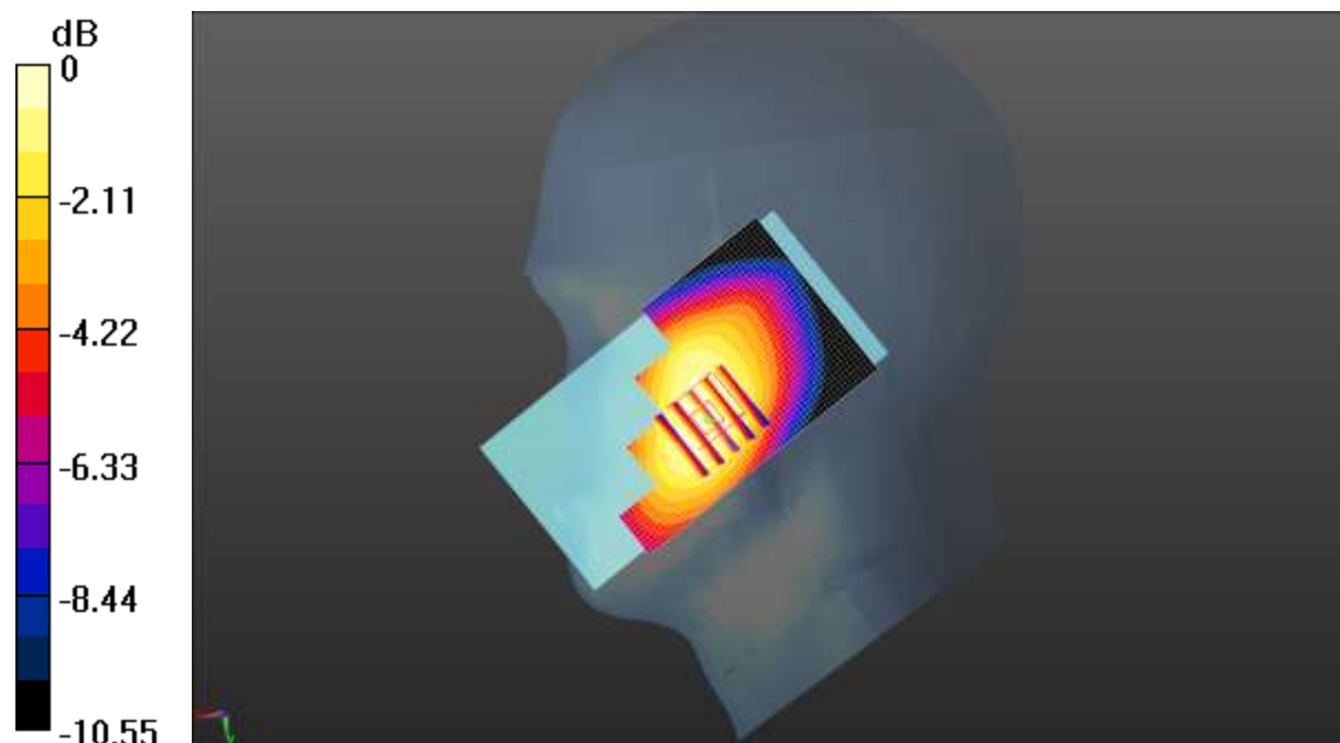
0 dB = 0.103 W/kg = -9.87 dBW/kg
