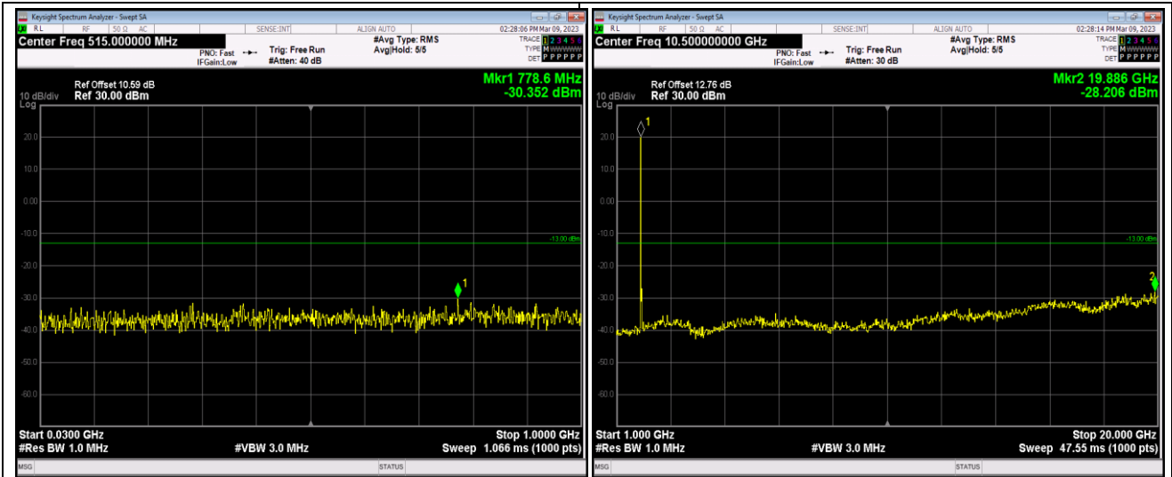
Band25-20MHz-64QAM-26365-1RB#0-Range1:30~1000MHz
