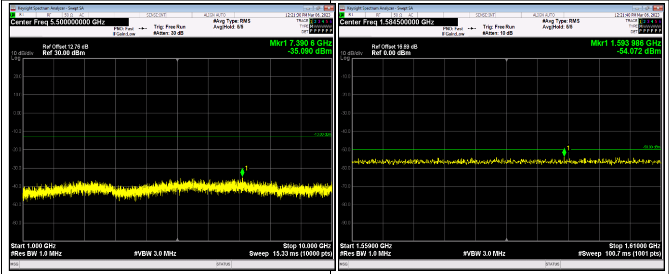
Band13-5MHz-16QAM-23205-1RB#0-Range2:1000~10000MHz
