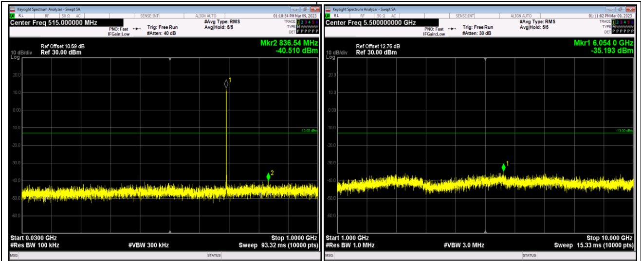
Band12-1.4MHz-64QAM-23095-1RB#0-Range1:30 ~1000MHz
