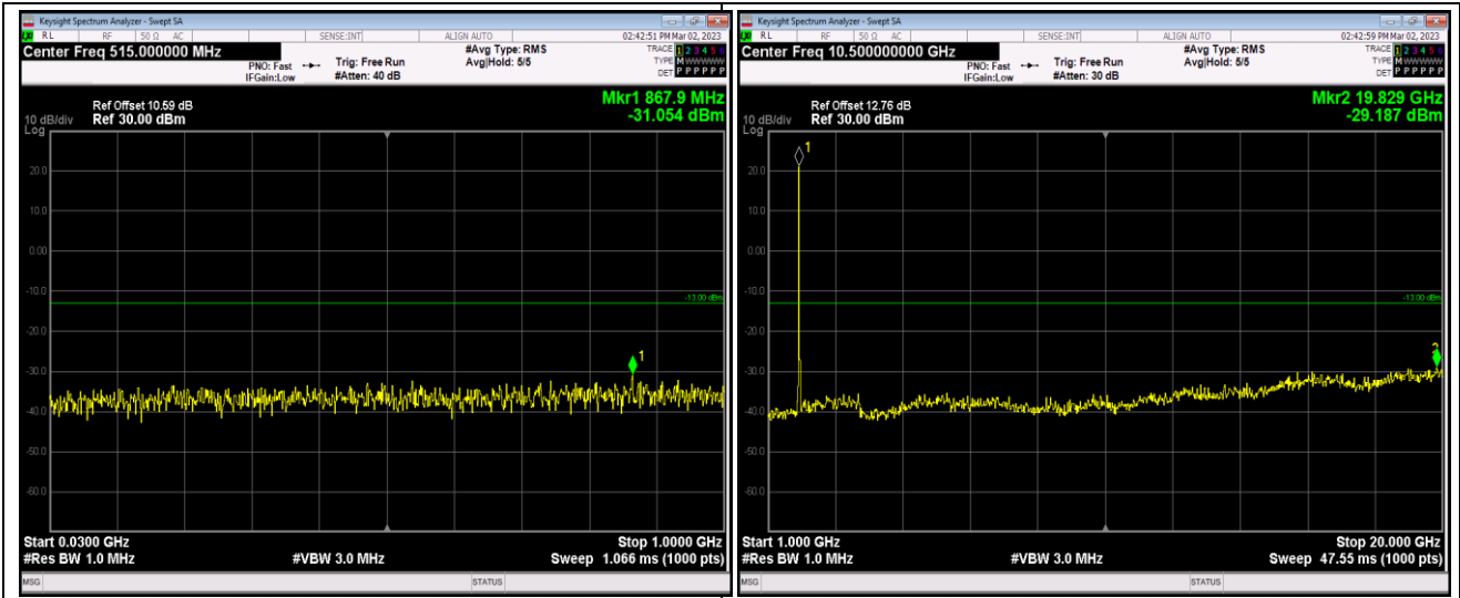
Band25-20MHz-QPSK-26590-1RB#0-Range1:30~1000MHz
