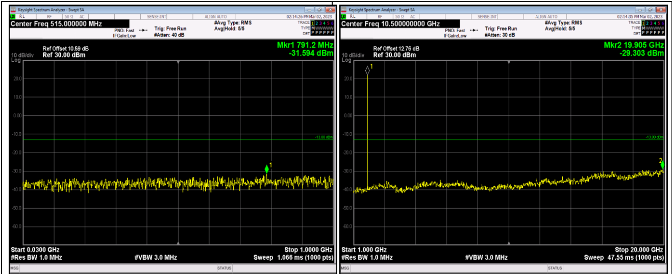
Band25-1.4MHz-QPSK-26365-1RB#0-Range1:30~1000MHz
