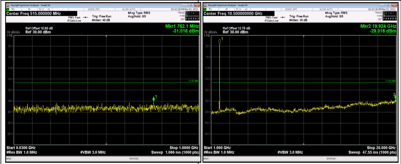
Band25-20MHz-16QAM-26140-1RB#0-Range1:30~1000MHz
