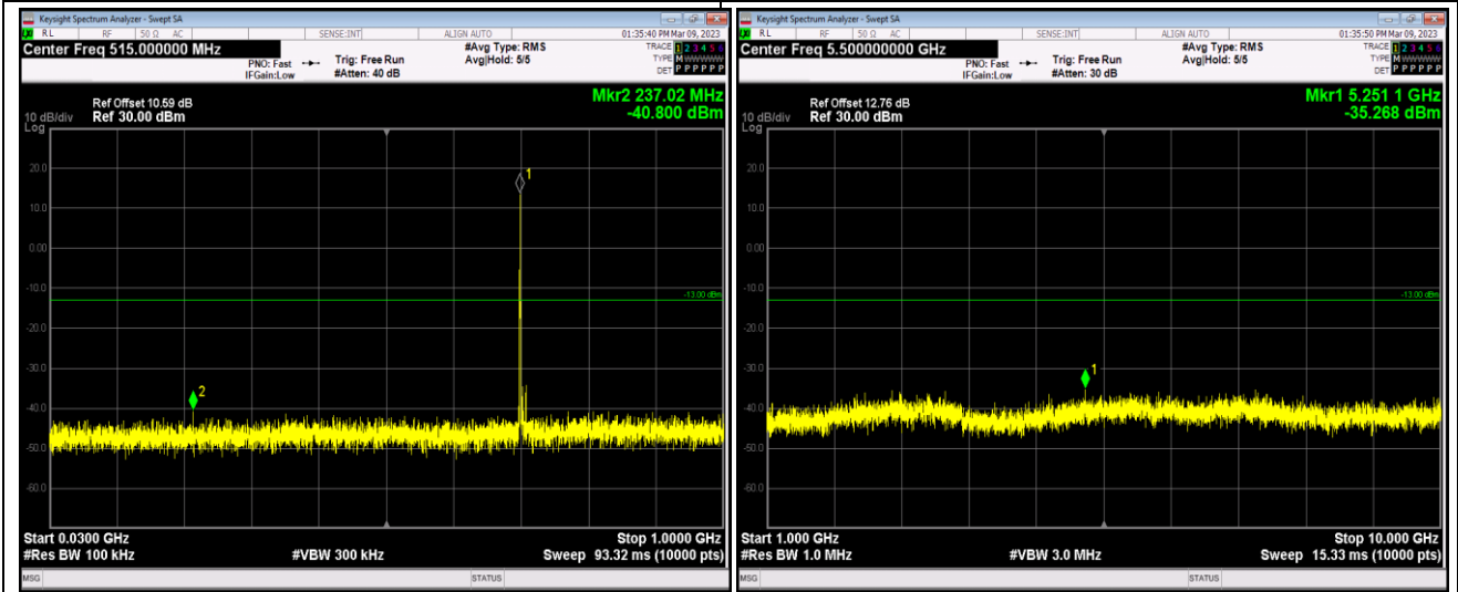
Band13-5MHz-QPSK-23205-1RB#0-Range1:30~1000MHz
