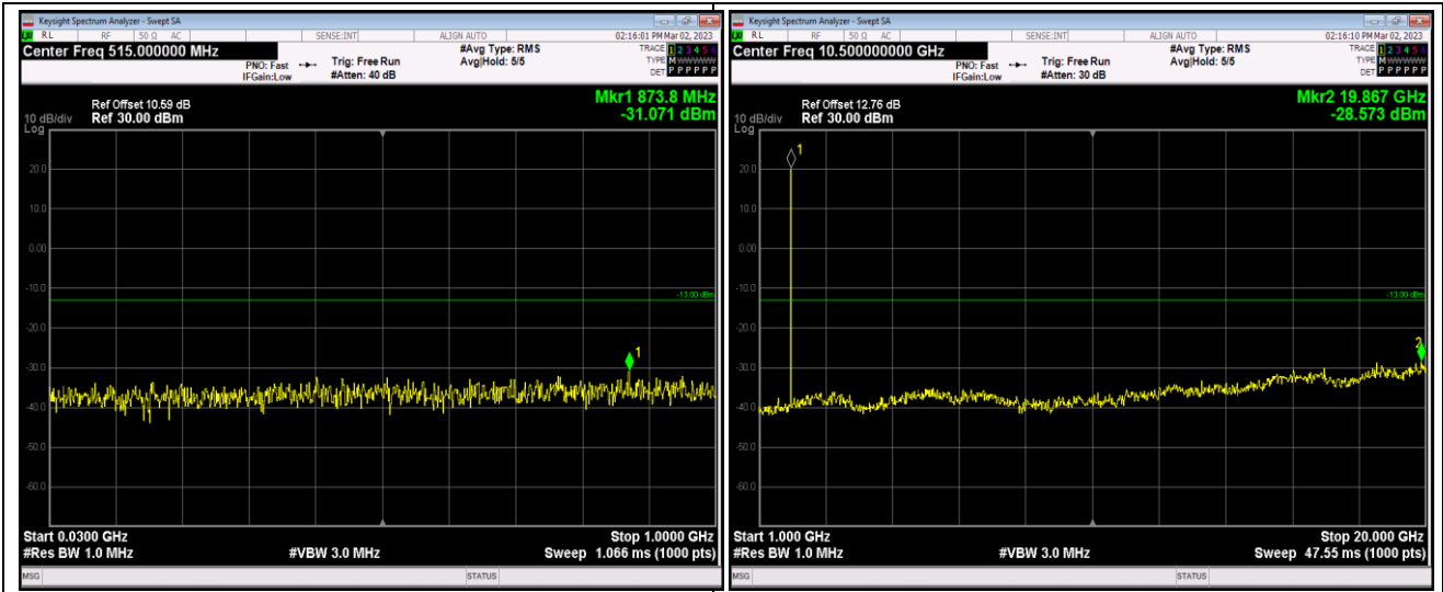
Band25-1.4MHz-64QAM-26047-1RB#0-Range1:30 ~1000MHz
