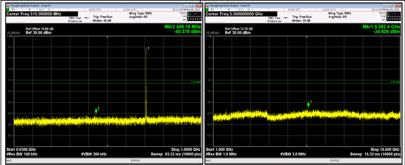
Band12-1.4MHz-64QAM-23173-1RB#0-Range1:30 ~1000MHz
