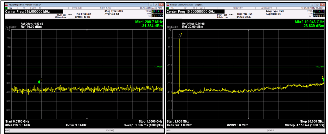
Band7-5MHz-QPSK-20775-1RB#0-Range1:30~100 OMHz
