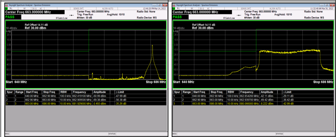
Band71-20MHz-64QAM-133372-1RB#0
