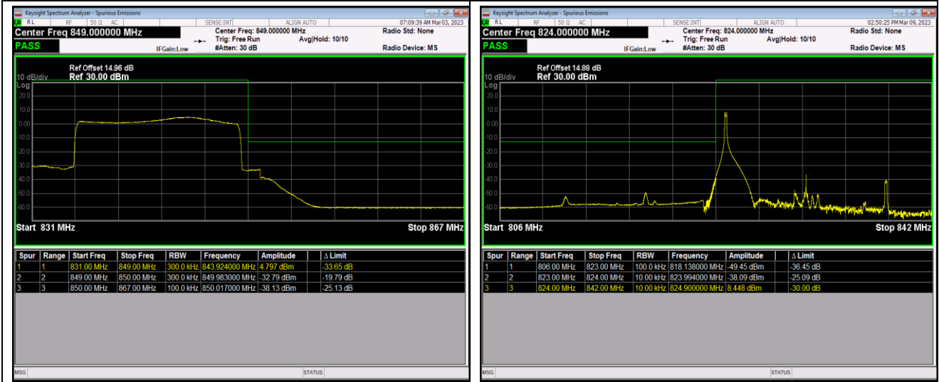
Band26-15MHz-64QAM-26865-1RB#74
