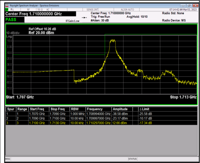
Band66-1.4MHz-QPSK-131979-6RB#0
