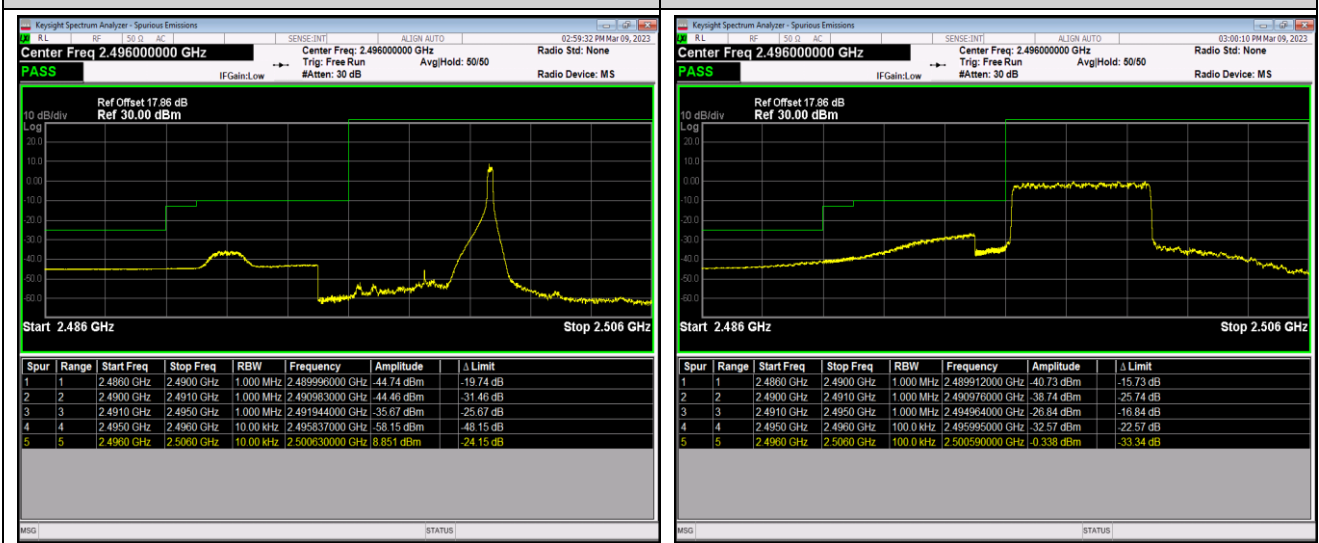
Band41-5MHz-64QAM-41565-1RB#0
