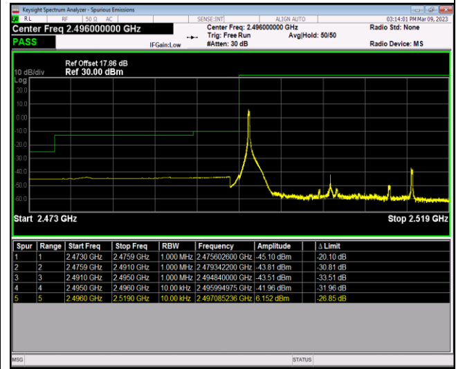
Band41-20MHz-64QAM-39750-100RB#0
