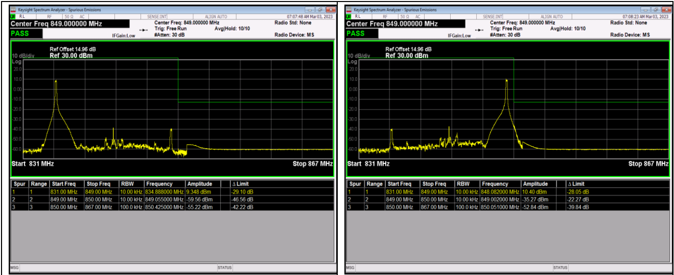
Band26-15MHz-16QAM-26965-75RB#0
