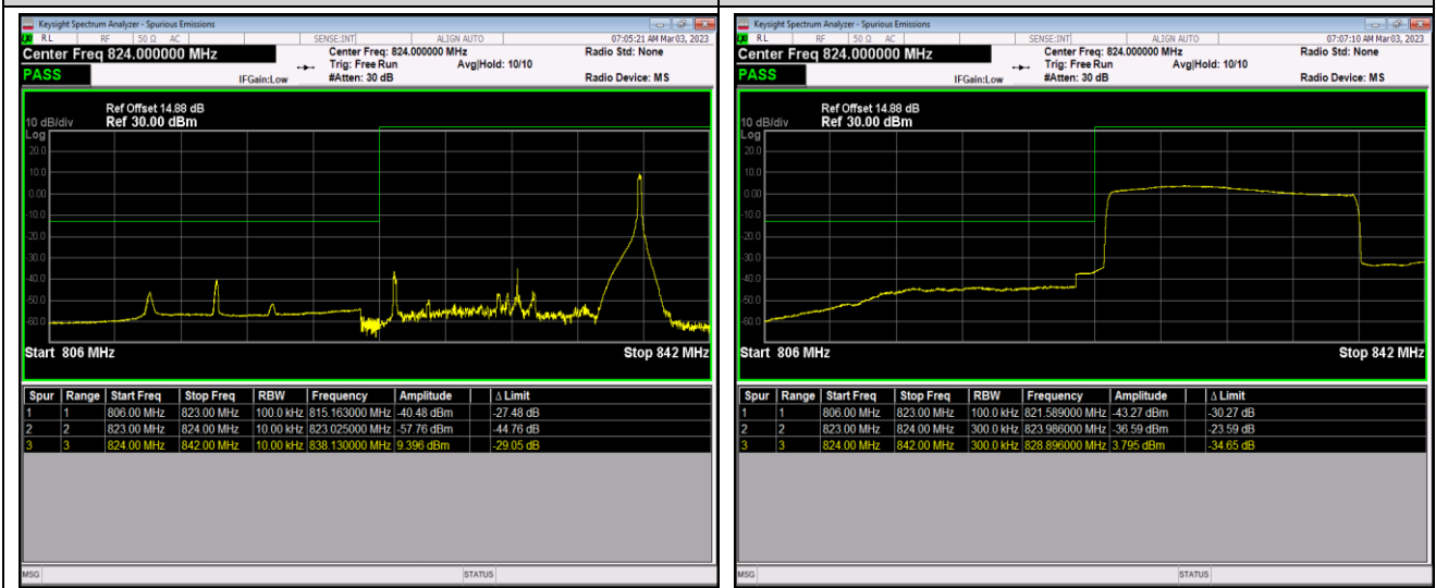
Band26-15MHz-16QAM-26965-1RB#0
