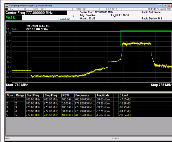
Band13-5MHz-64QAM-23255-1RB#24
