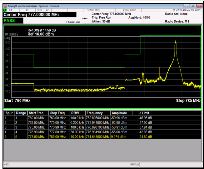
Band13-5MHz-64QAM-23255-1RB#0
