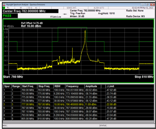
Band13-10MHz-16QAM-23230-1RB#0
