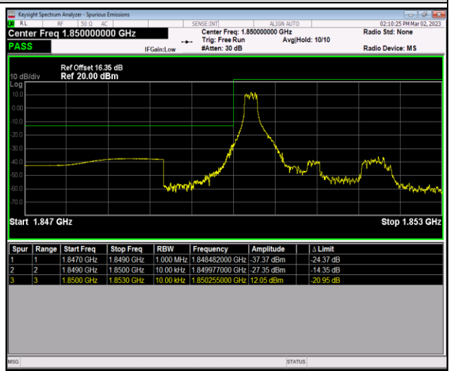
Band25-1.4MHz-16QAM-26047-6RB#0
