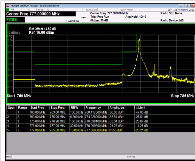
Band13-5MHz-64QAM-23205-25RB#0
