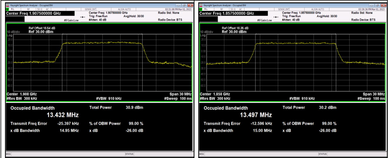
Band25-15MHz-16QAM-26365-75RB#0
