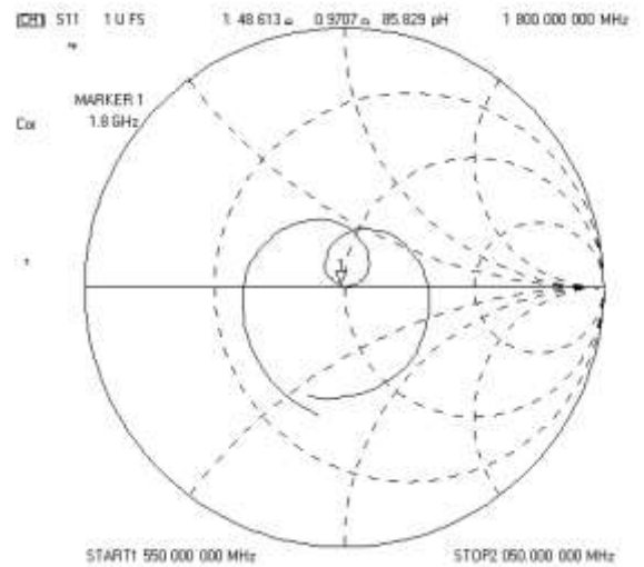
Measurement Plot for Body TSL In 2017 (Mar 15,2017)
