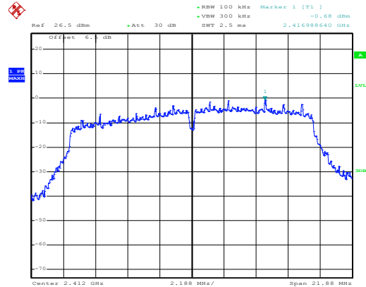
Test mode: 802.11g
