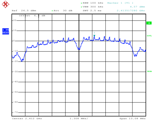
Test mode: 802.11b
