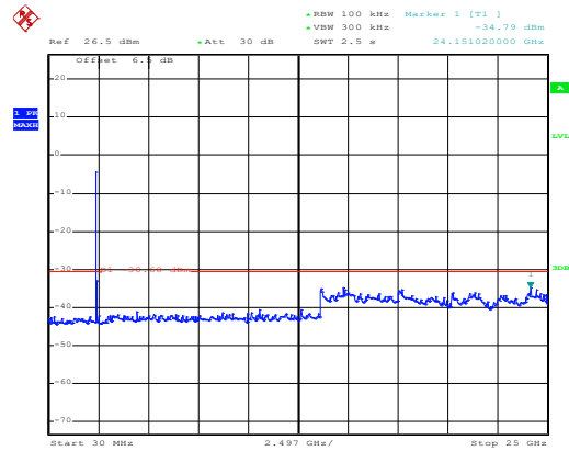
Test mode: 802.11g Lowest channel
