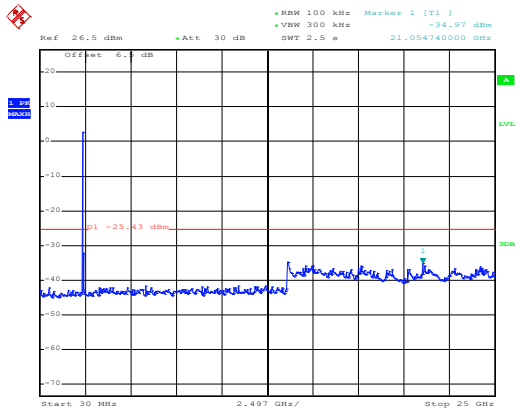
Test mode: 802.11b Lowest channel
