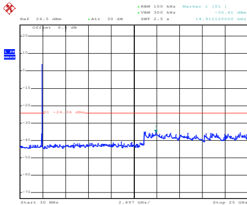
30MHz~25GHz Middle channel
