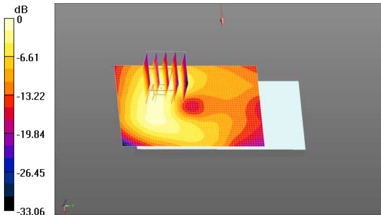
0 dB = 0.352 W/kg = -4.53 dBW/kg
