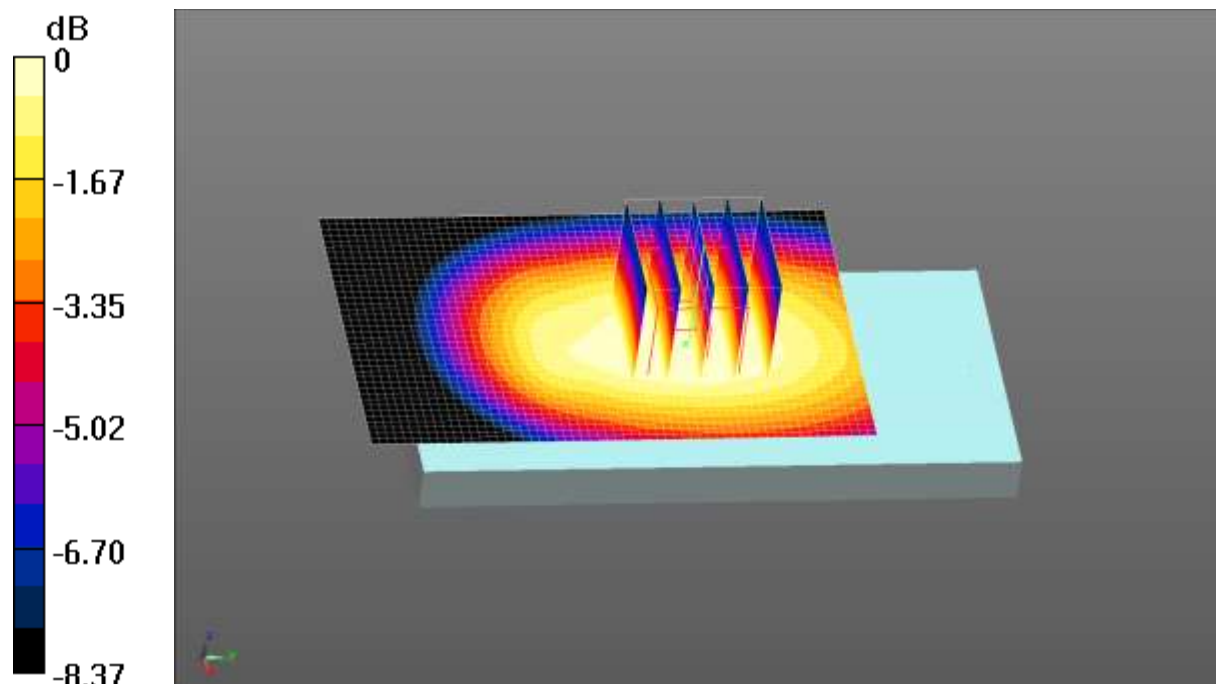
0 dB = 0.387 W/kg = -4.12 dBW/kg
