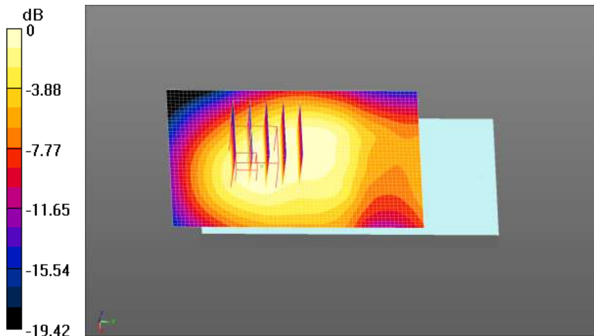
0 dB = 0.452 W/kg = -3.45 dBW/kg
