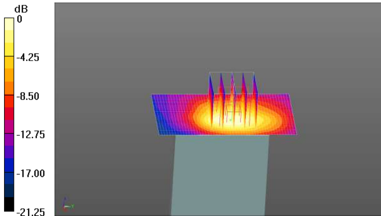
0 dB = 0.535 W/kg = -2.72 dBW/kg
