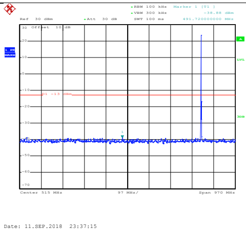
30MHz~1GHz
