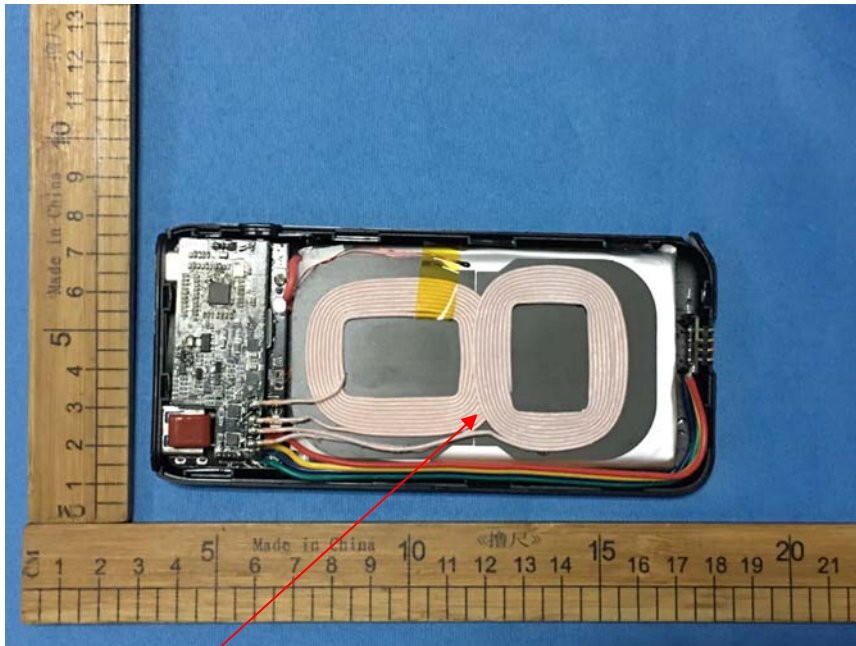
Coil Antenna
