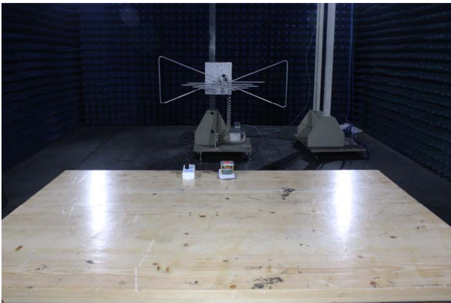
Photo of Radiation Emission Measurement: 30MHz to 1GHz
