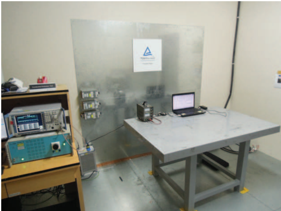
Photograph 27: Set-up for Mains Conducted testing (Front View)
