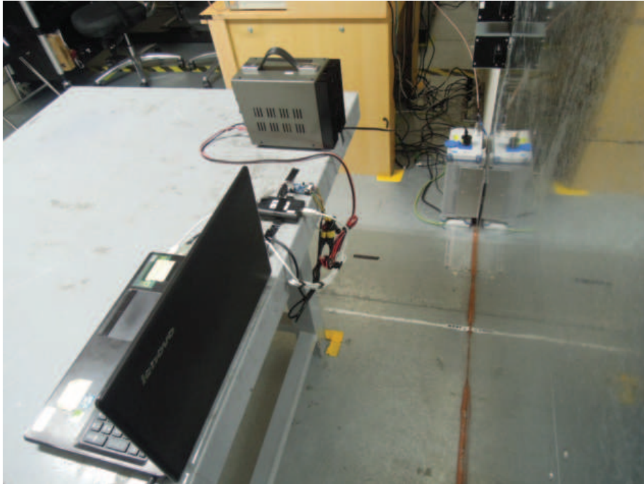
Photograph 28: Set-up for Mains Conducted testing (Back View)
