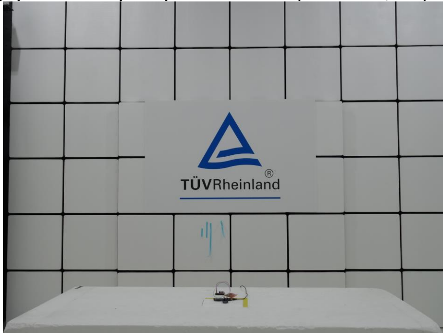
Photograph 9: Test Setup for Spurious Emissions (Front View 1, WiFi)
