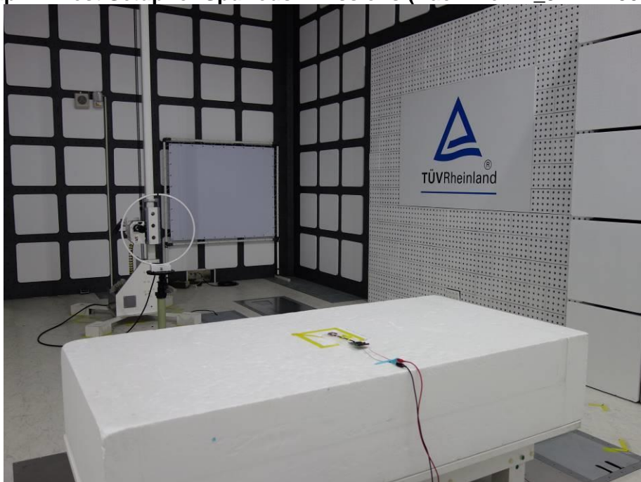
Photograph 4: Test Setup for Spurious Emissions (Back View 2_9kHz ~ 30MHz)
