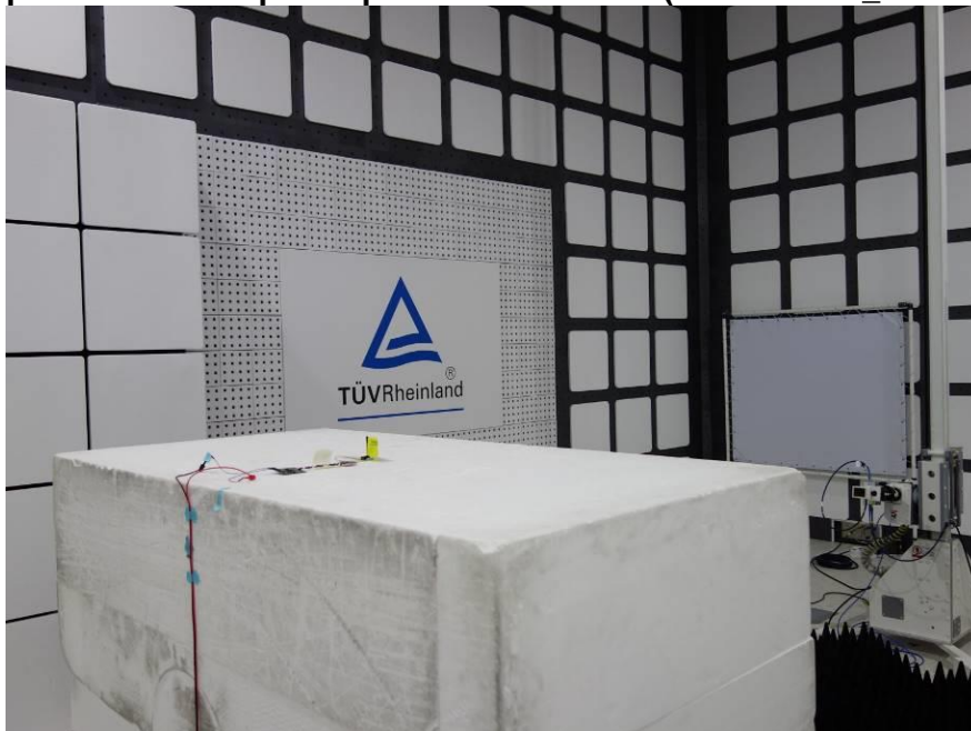
Photograph 12: Test Setup for Spurious Emissions (Back View 4_18GHz ~ 26.5GHz)
