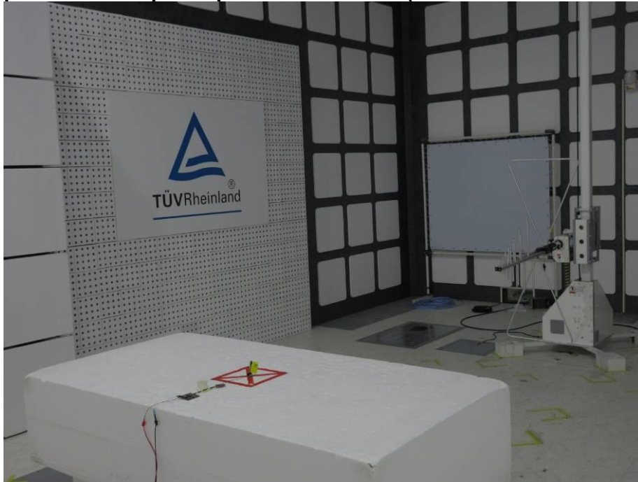
Photograph 10: Test Setup for Spurious Emissions (Back View 2_9kHz ~ 30MHz)
