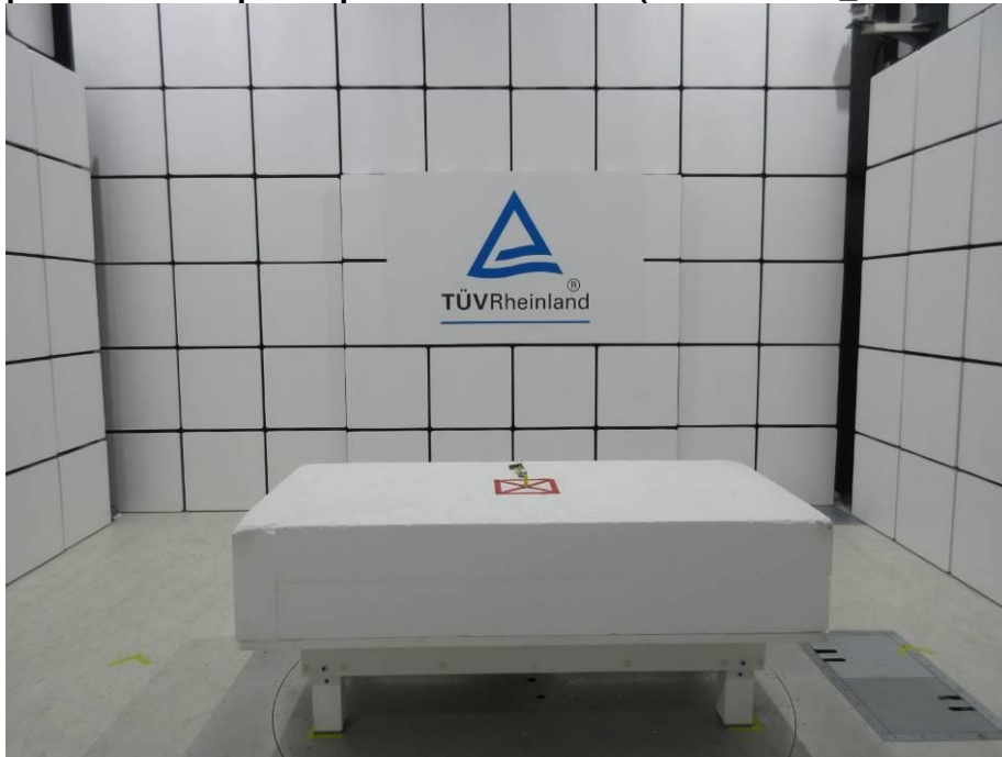
Photograph 8: Test Setup for Spurious Emissions (Front View 2_Above 1GHz)
