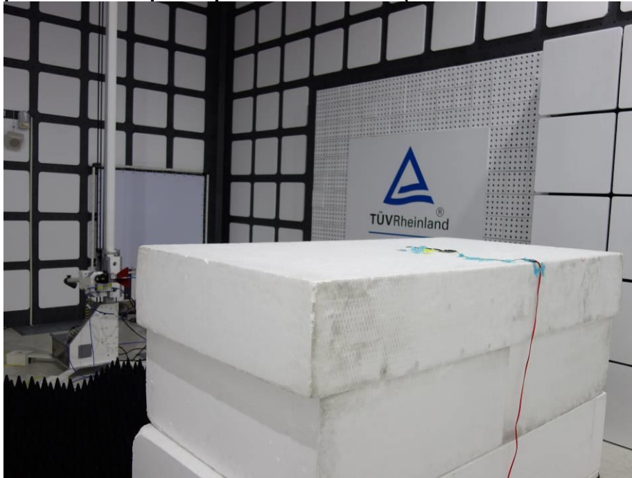
Photograph 6: Test Setup for Spurious Emissions (Back View 4_18GHz ~ 26.5GHz)
