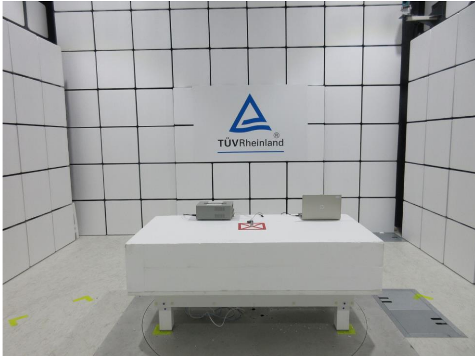
Photograph 7: Set-up for Spurious Emissions (Front View 1, #6)
