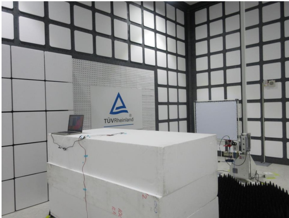
Photograph 26: Set-up for Spurious Emissions (Back View 1, #238)
