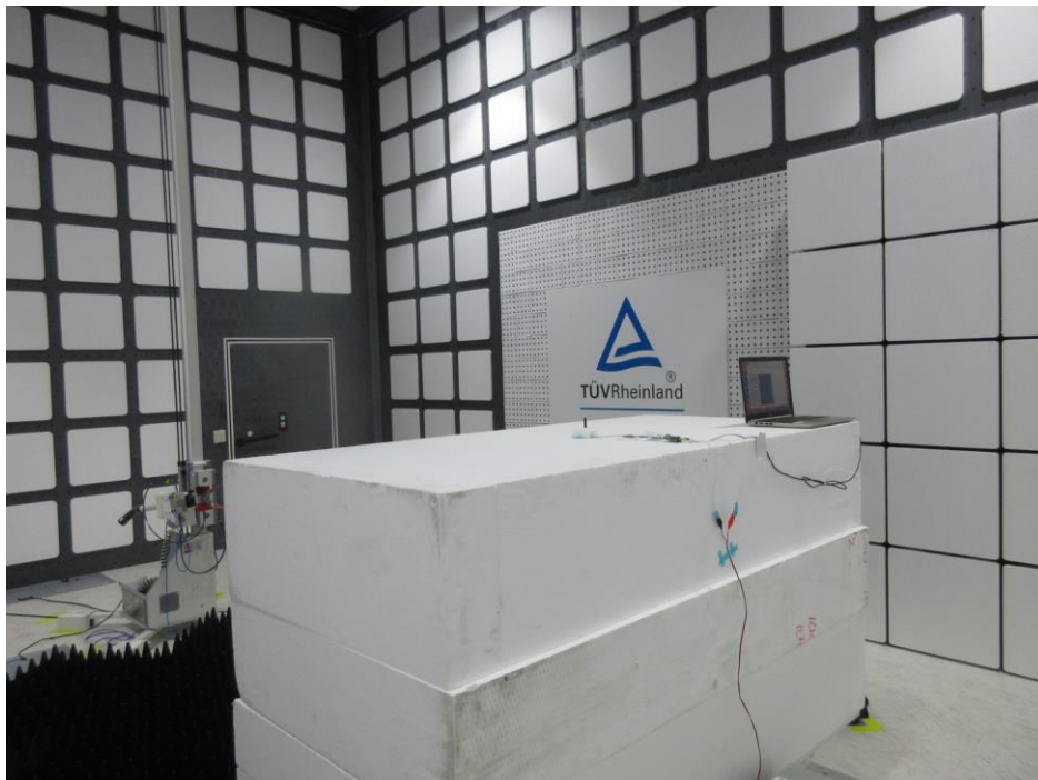
Photograph 14: Set-up for Spurious Emissions (Back View 1, #61)
