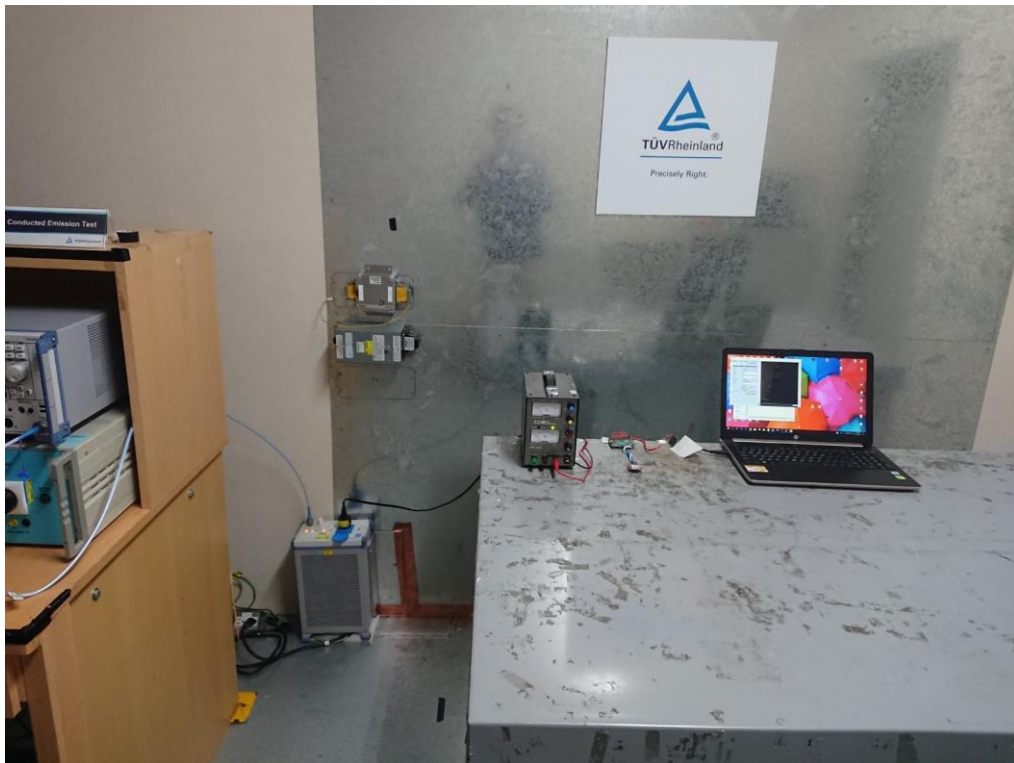
Photograph 34: Set-up for AC Mains (Front View)
