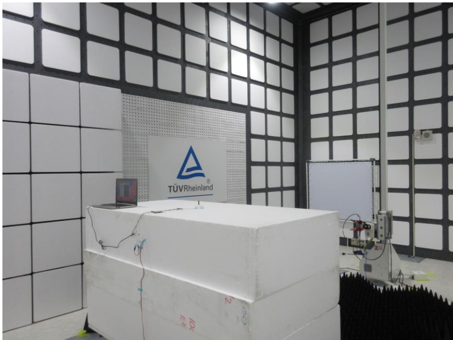
Photograph 20: Set-up for Spurious Emissions (Back View 1, #207)
