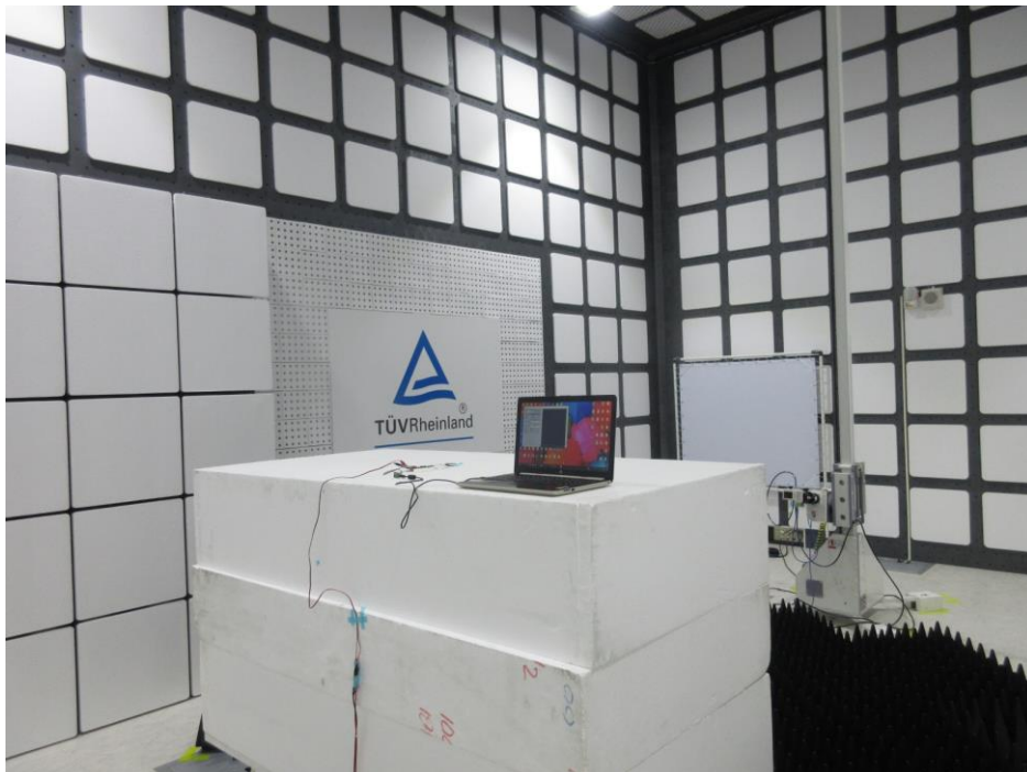
Photograph 24: Set-up for Spurious Emissions (Back View 2, #221)
