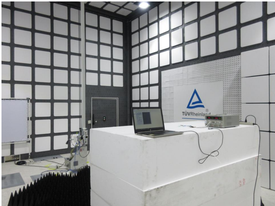
Photograph 12: Set-up for Spurious Emissions (Back View 4, #6)
