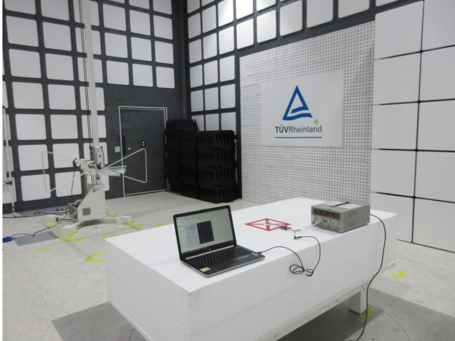
Photograph 9: Set-up for Spurious Emissions (Back View 1, #6)
