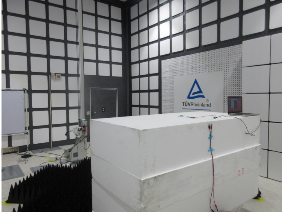
Photograph 17: Set-up for Spurious Emissions (Back View 1, #64)
