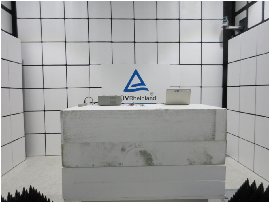
Photograph 8: Set-up for Spurious Emissions (Front View 2, #6)
