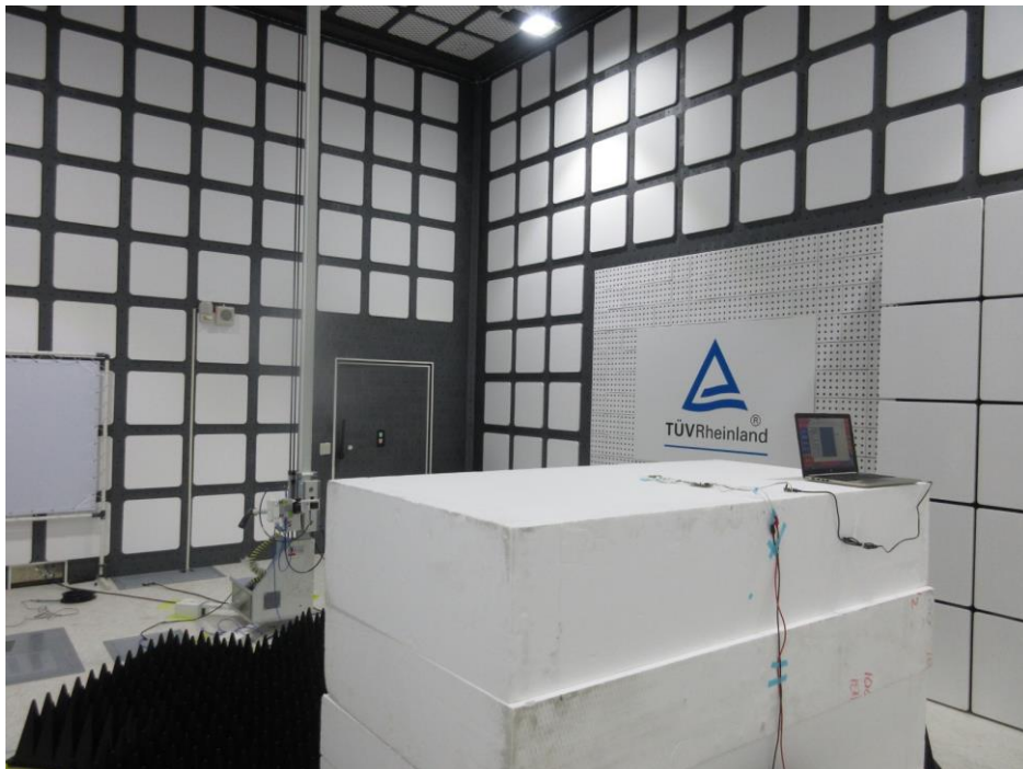
Photograph 18: Set-up for Spurious Emissions (Back View 2, #64)
