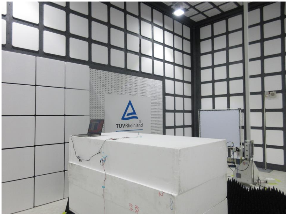
Photograph 30: Set-up for Spurious Emissions (Back View 2, #240)
