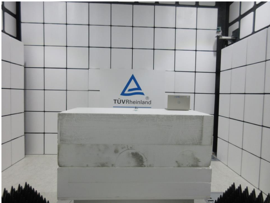
Photograph 28: Set-up for Spurious Emissions (Front View, #240)
