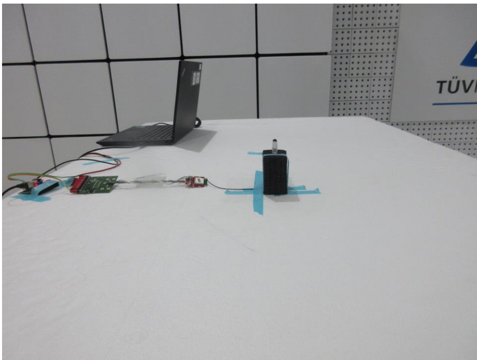
Photograph 32: Set-up for Spurious Emissions (Back View 1, #214)
