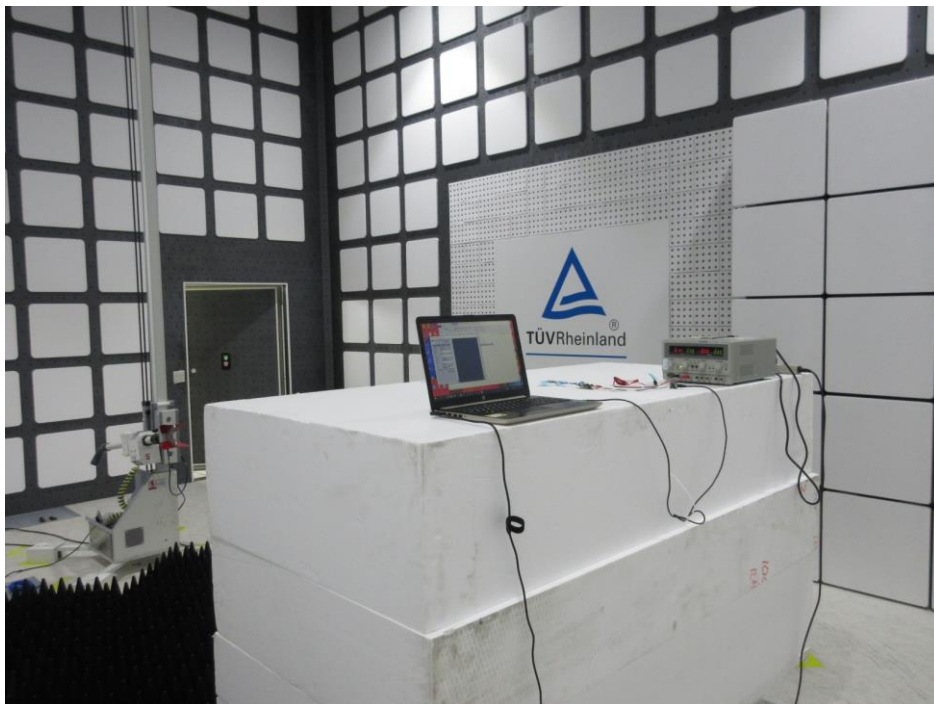
Photograph 10: Set-up for Spurious Emissions (Back View 2, #6)
