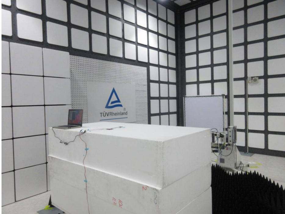
Photograph 27: Set-up for Spurious Emissions (Back View 2, #238)
