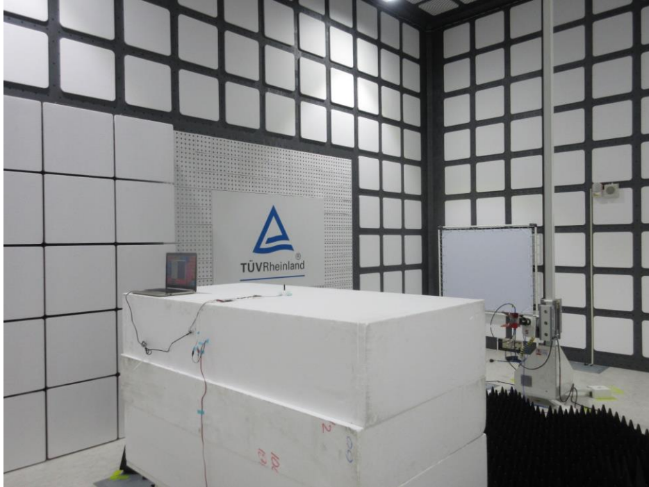
Photograph 29: Set-up for Spurious Emissions (Back View 1, #240)
