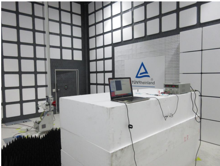
Photograph 4: Set-up for Spurious Emissions (Back View 2, #5)
