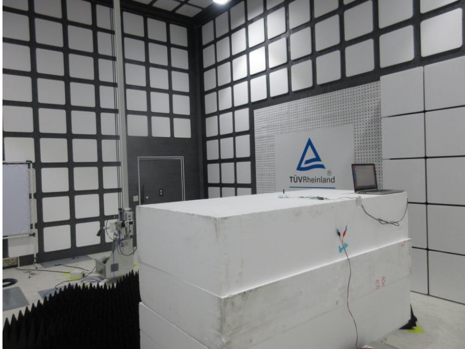
Photograph 15: Set-up for Spurious Emissions (Back View 2, #61)
