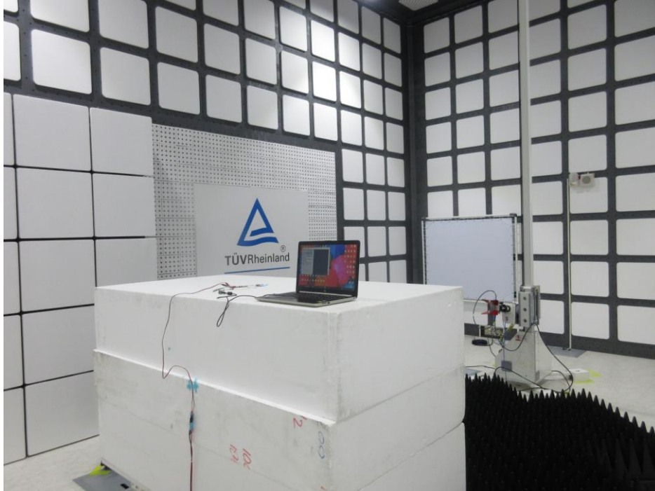
Photograph 23: Set-up for Spurious Emissions (Back View 1, #221)
