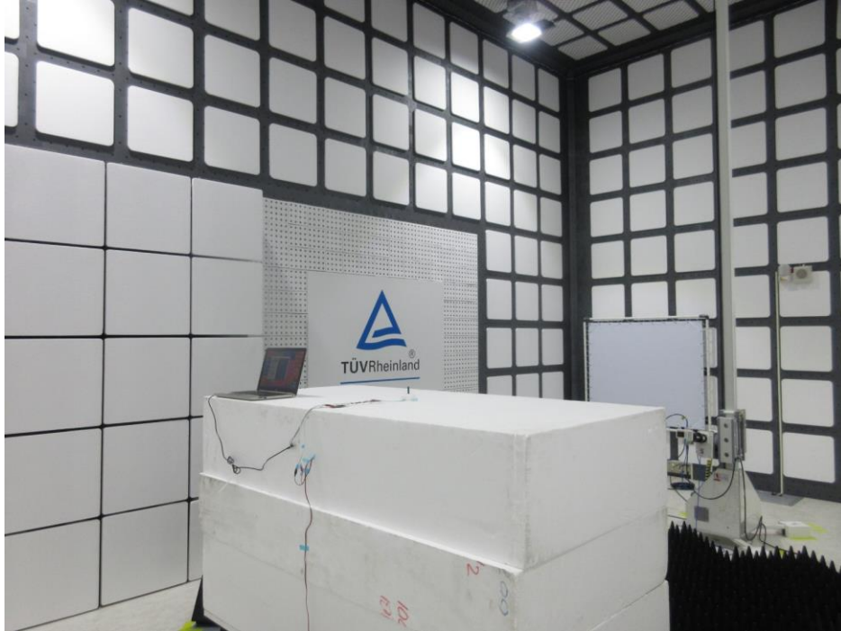
Photograph 21: Set-up for Spurious Emissions (Back View 2, #207)
