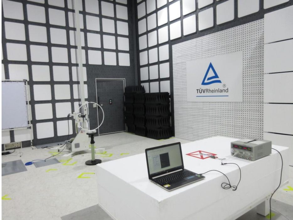
Photograph 11: Set-up for Spurious Emissions (Back View 3, #6)
