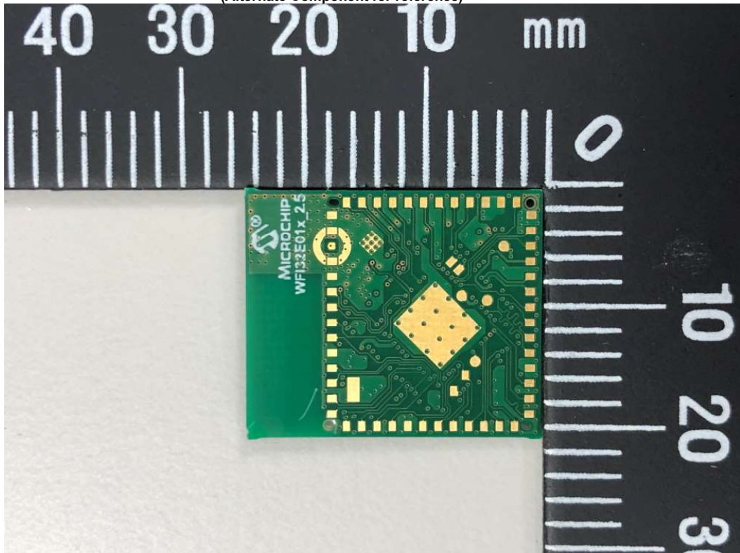
Internal Photo of WFI32E01UC (Module with u.FL Connector for External Antenna and Trust&GO) (Alternate Component for reference)
