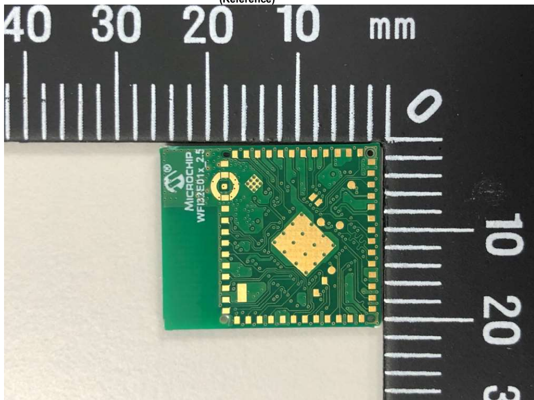
Internal Photo of WFI32E01UC (Module with u.FL Connector for External Antenna and Trust&GO) (Reference)
