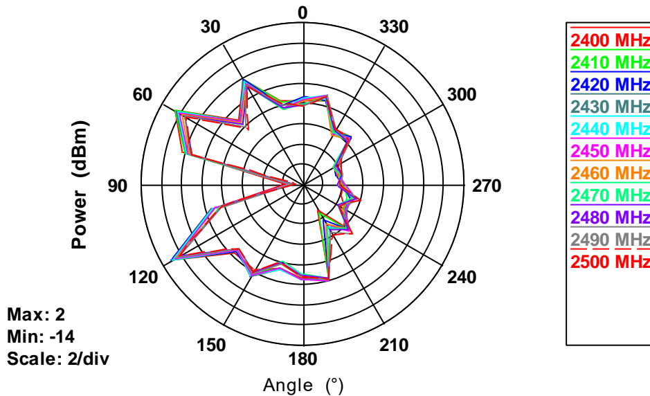
WBZ451HPA with Ground plane 2D_XZ-Cut
