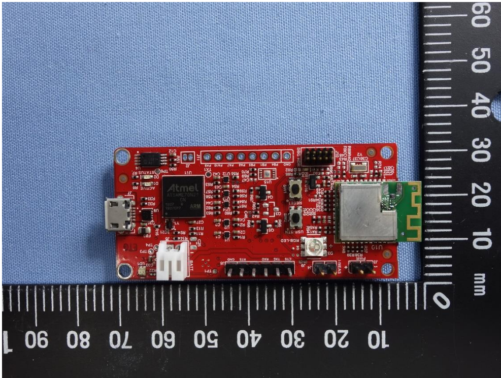
Onboard PCB
