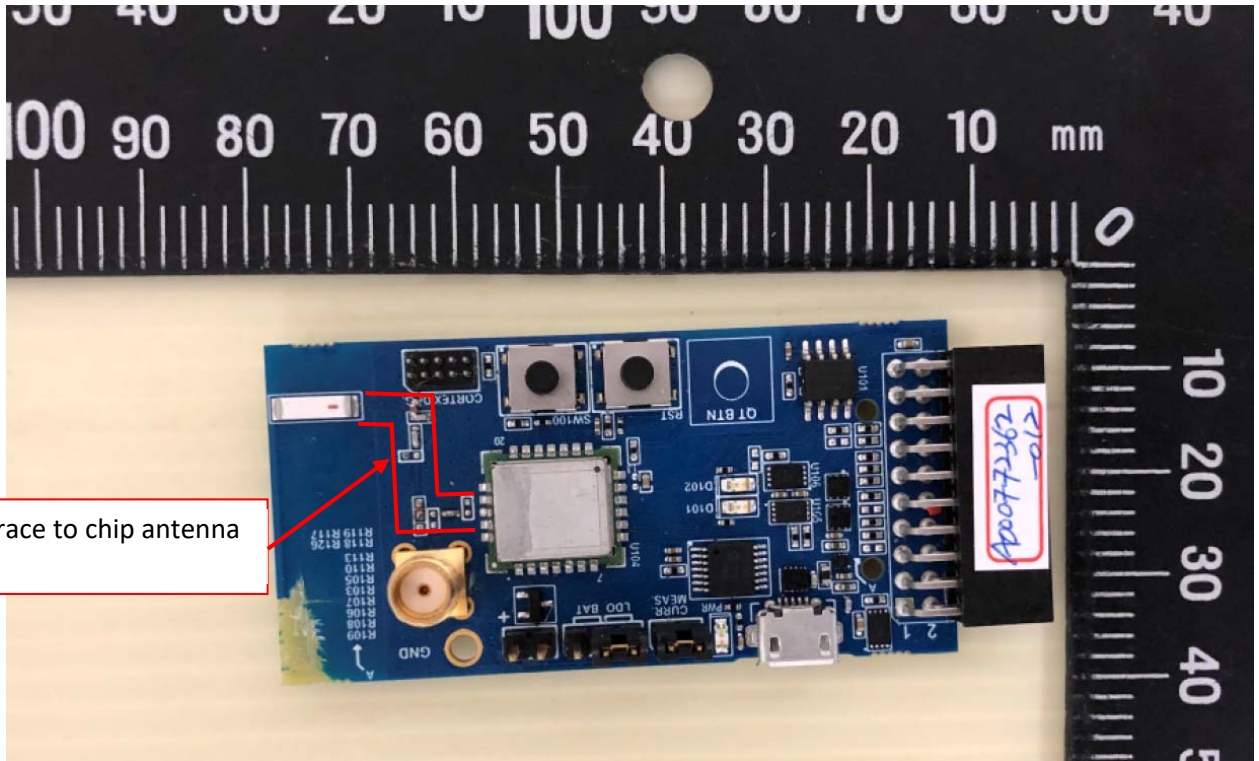
Module with Chip antenna(0900AT43A0070)
