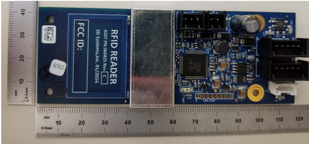
Top view – with EMI shield
