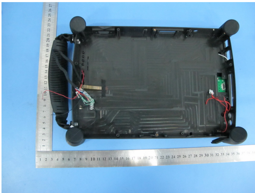
Photo 19 Appearance of Battery
