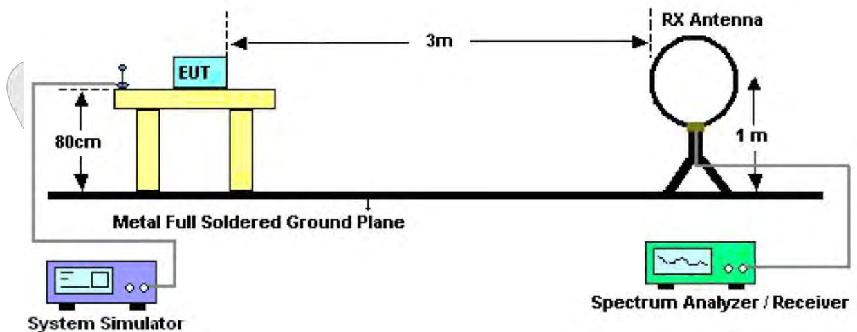
Figure 1. Below 30MHz
