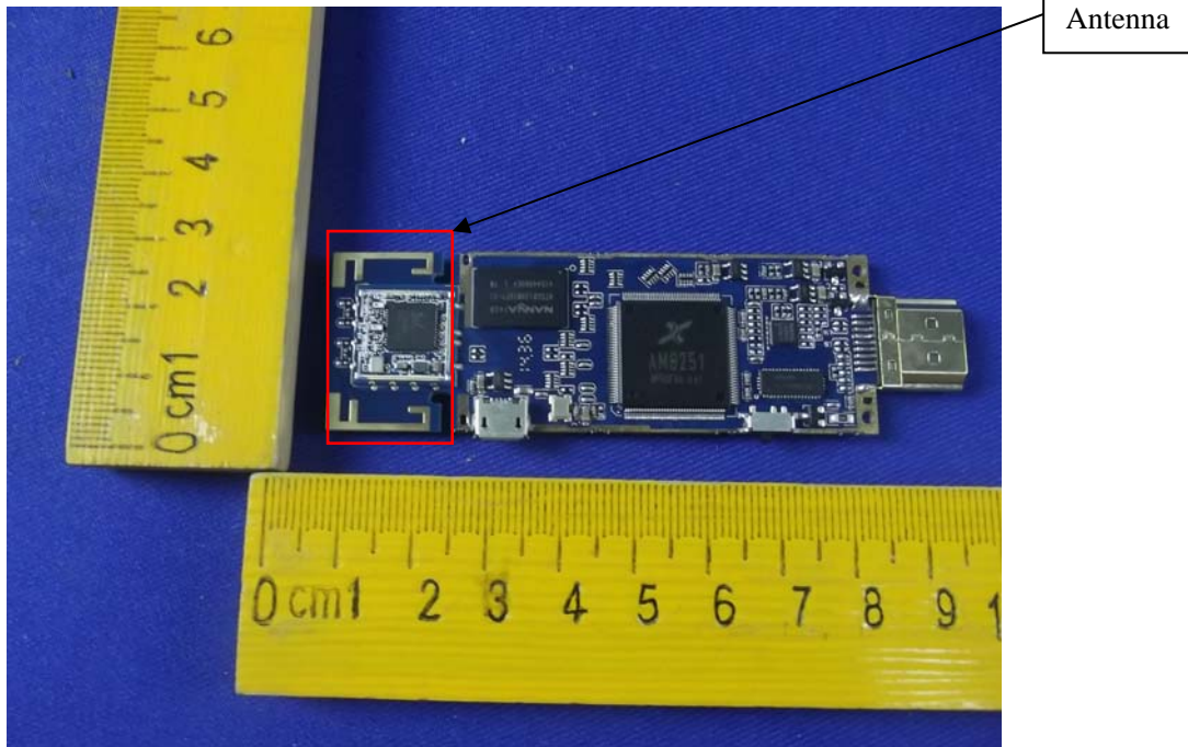
Figure 9 PCB of the EUT-Front View
